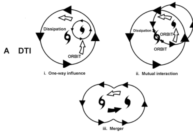
Figure 1-7a. Tropical Cyclone Interaction: (a) Direct TC Interaction (DTI) is composed of three types - (i) one way influence, (ii) mutual interaction, and (iii) merger.
