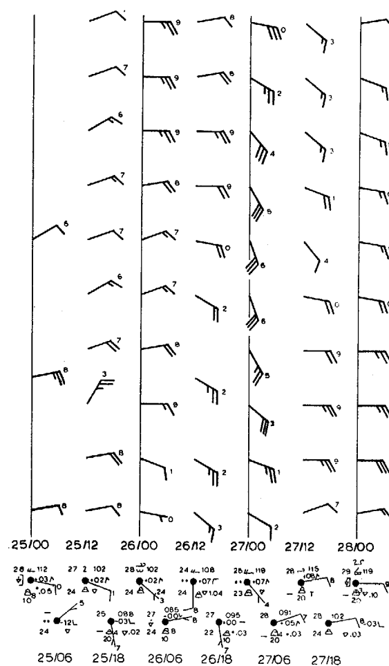
TIME CROSS SECTIONS OF RAWIN PROFILES FOR TRUK AND PONAPE ISLANDS DURING PASSAGE OF THE PRE-OLGA DISTURBANCE LATE JUNE 1970
