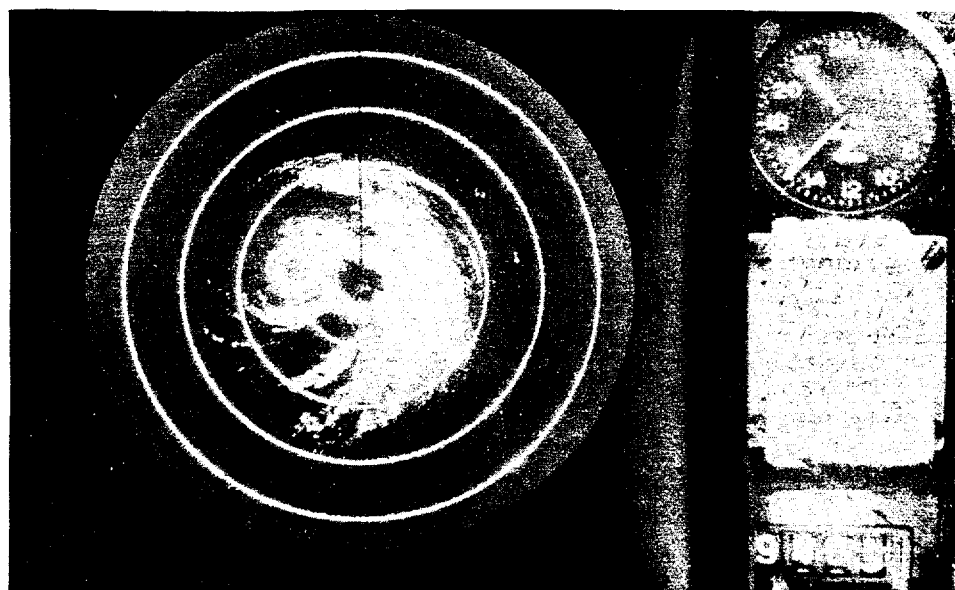
FIGURE 5-26. APS-20 RADARSCOPE PICTURE OF NADINE TAKEN FROM NAVY RECONNAISSANCE AIRCRAFT (VQ-1) AT 2137 GMT 23 JULY (RANGE MARKS ARE AT 50 N MI INTERVALS).
