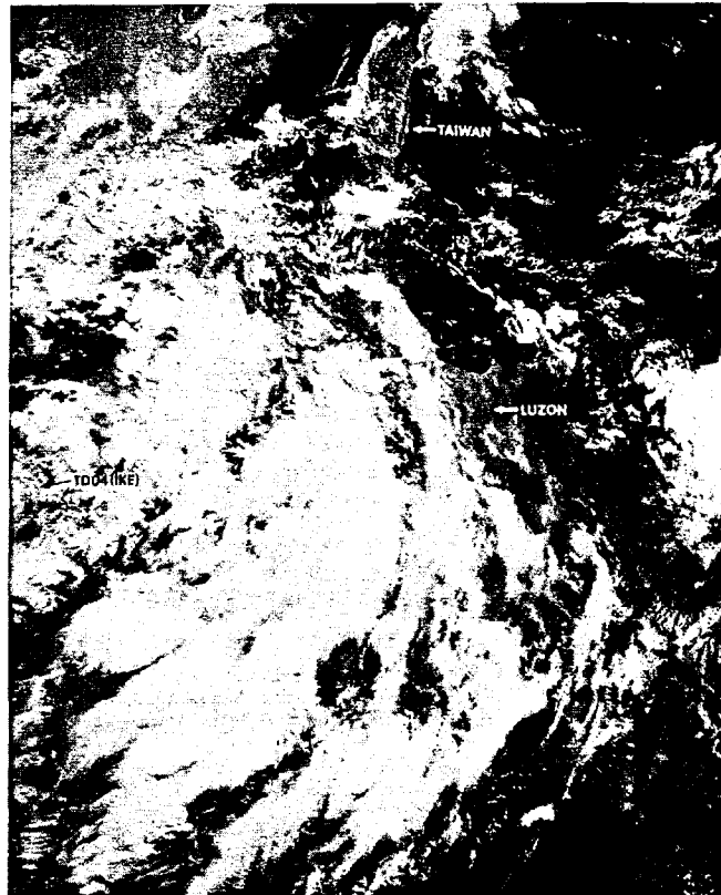
Figure 3-04-1. Tropical Depression 04 as it began to develop and consolidate its associated convection while over the South China Sea, 9 June 1981, 2336Z (NOAA 6 visual imagery).
