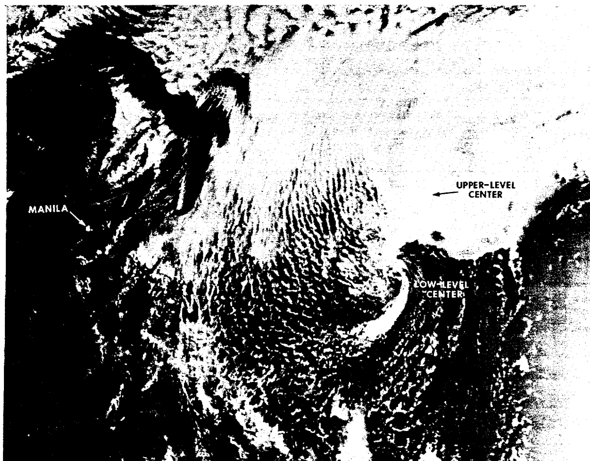
Figure 3-28-7. A weakening Tropical Storm Kit, with the low-level center moving southward while the remnants of her convection move northeastward into a shortwave trough. Note the hyper-extended circulation pattern. The low-level steering was literally stretching Kit southward with time, 200609Z December. (NOAA 7 visual imagery)
