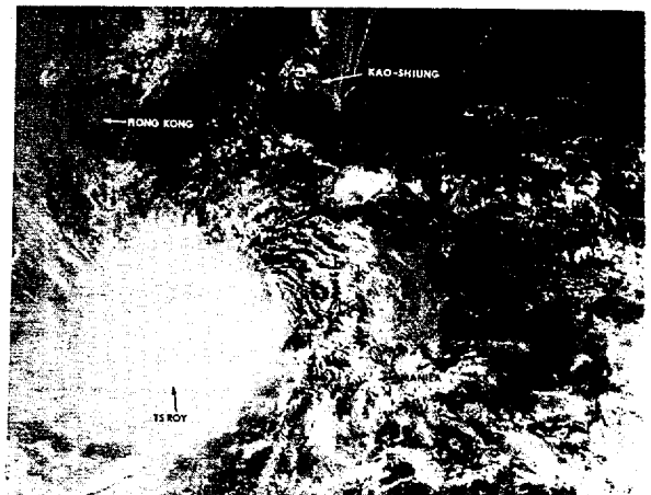
FIGURE 03-13-2. NOAA 6 VIS 052340Z AUG 81 Visual satellite imagery for the first time shows Roy as a partially exposed low-level circulation center. (052340Z Aug 81) During the 24 hours which followed, Roy would become fully exposed and would begin a gradual weakening trend. (NOAA 6 visual imagery)
