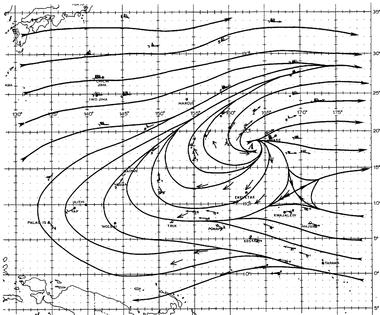
FIGURE 3-01-2. 200-mb streamline analysis at 150000Z depicting a dramatic change in the upper-level flow pattern with the outflow over Freda now the primary feature. The westerly jet has dipped as far south as 25N providing a vigorous outflow channel to the northeast for Freda. Wind data are a combination of RAOBS, AIREPS, and satellite derived winds (←) and blow-off wind directions (←). Wind speeds are in knots.
