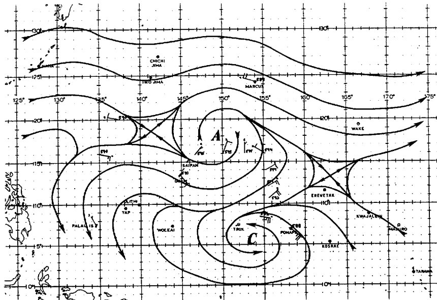
FIGURE 3-02-2. The 151200Z April 1981 500 mb streamline analysis. Wind data are a combination of RAOBS, AIREPS, and satellite derived winds ( ← ). Wind speeds are in knots.
