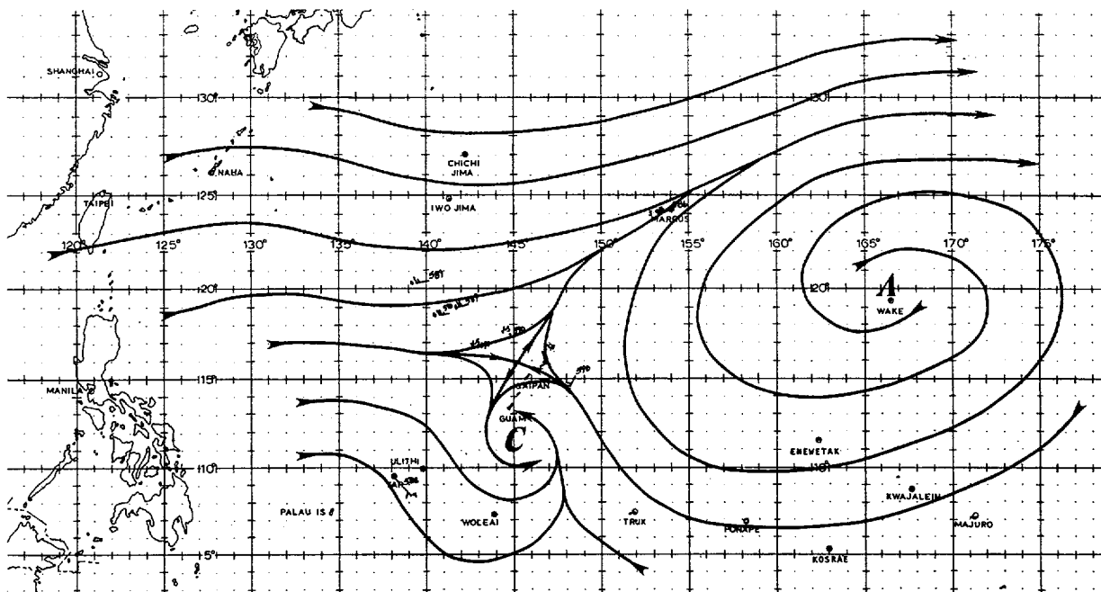
FIGURE 3-02-4. The 171200Z April 1981 500-mb streamline analysis. Wind data are a combination of RAOBS, AIREPS, and satellite derived winds (←). Wind speeds are in knots.
