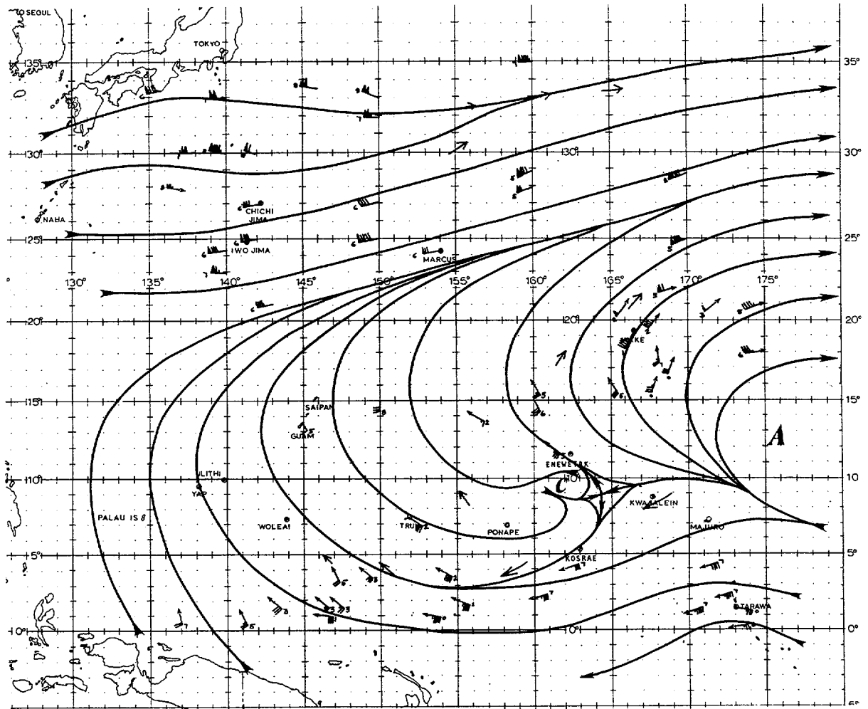
FIGURE 3-01-1. 200-mb streamline analysis at 131200Z. At this time, the flow pattern was still primarily associated with the mid-Pacific ridge with little indication of large-scale outflow over Freda at this level. Wind data are a combination of RAQBS, AIREPS, and satellite derived winds (←) and blow-off wind directions (←). Wind speeds are in knots.
