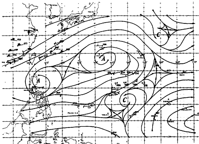
Figure 3-03-4. 500 mb streamline analysis at 051200Z. This analysis was typical of the pattern existing during Holly's lifetime. Wind data are a combination of RAOBS, RECON, and satellite-derived winds (←). Wind speeds are in knots.
