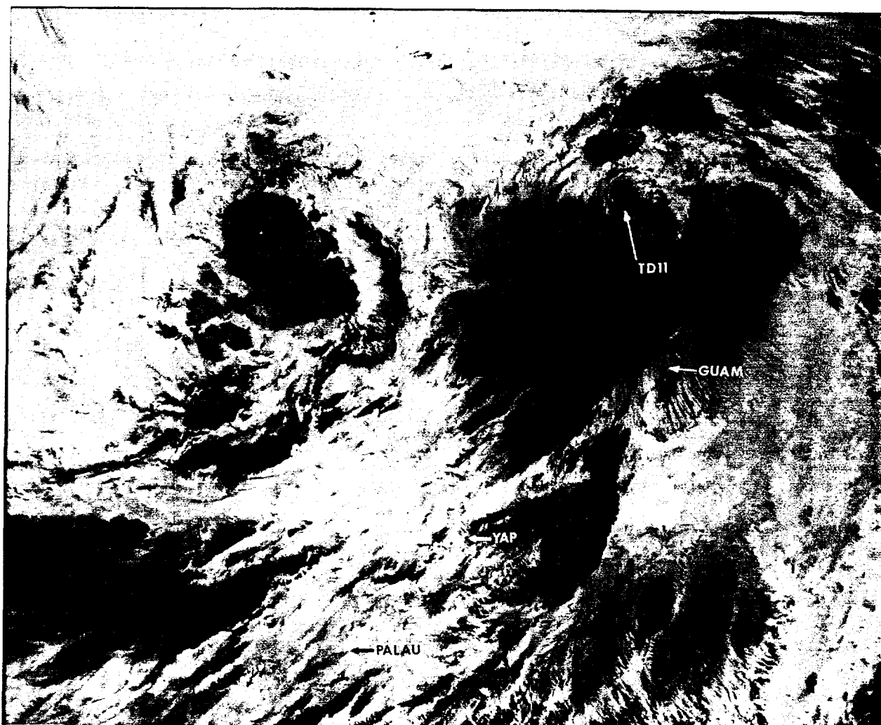
FIGURE 3-11-1. TD-11 early in its development on 30 July 1981, 2236Z. (NOAA 6 infrared imagery)
