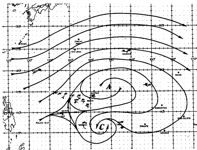
FIGURE 3-02-3. The 161200Z April 1981 500-mb streamline analysis. Wind data are a combination of RAOBS, AIREPS, and satellite derived winds ( ← ). Wind speeds are in knots.
