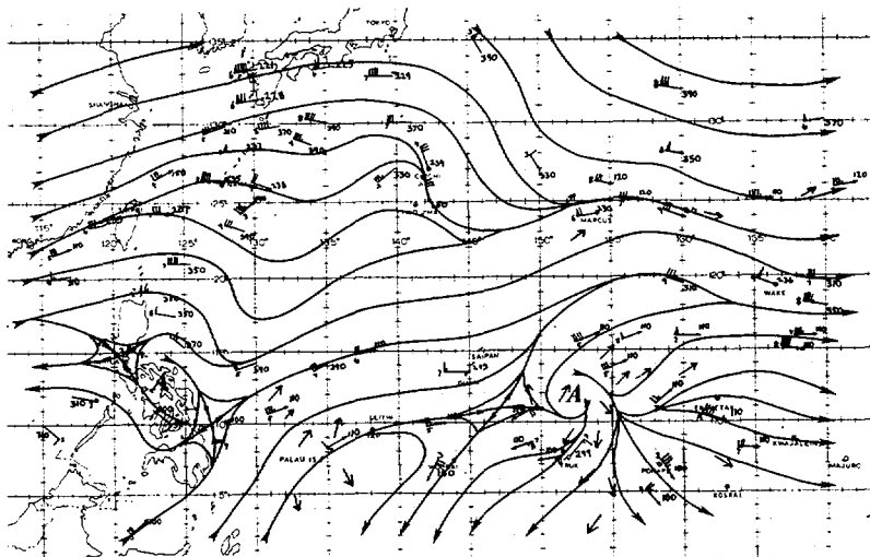
Figure 3-03-5. 200 mb streamline analysis at 031200Z. Wind data are a combination of RAOBS, AIREPS, and satellite-derived winds (←) and blow-off wind directions (←). Wind speeds are in knots.
