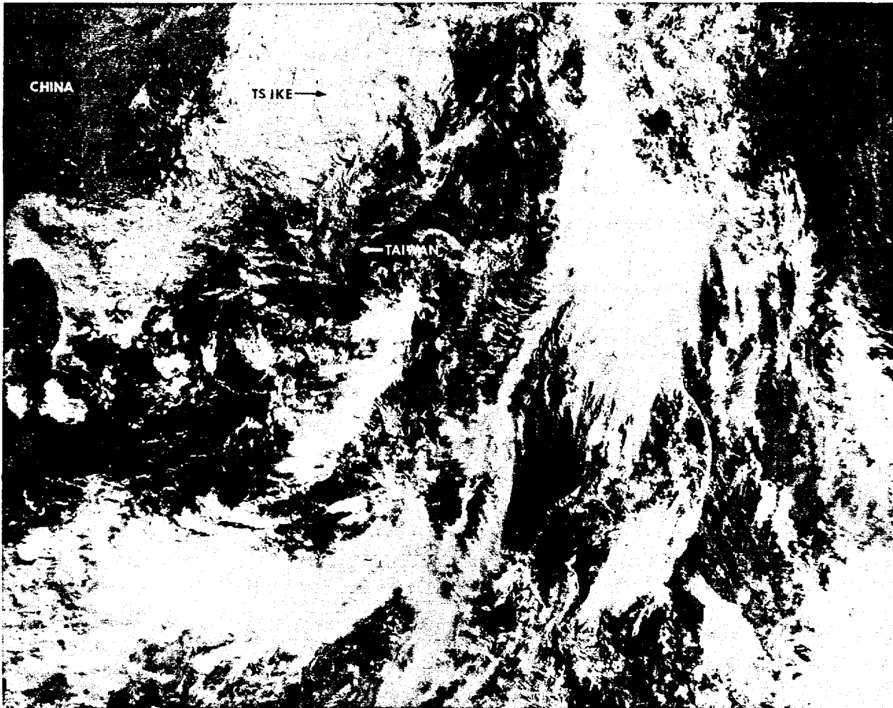
Figure 3-04-2. Tropical Storm Ike as a partially exposed low-level circulation as he began extratropical transition, 13 June 2245Z (NOAA 6 visual imagery).
