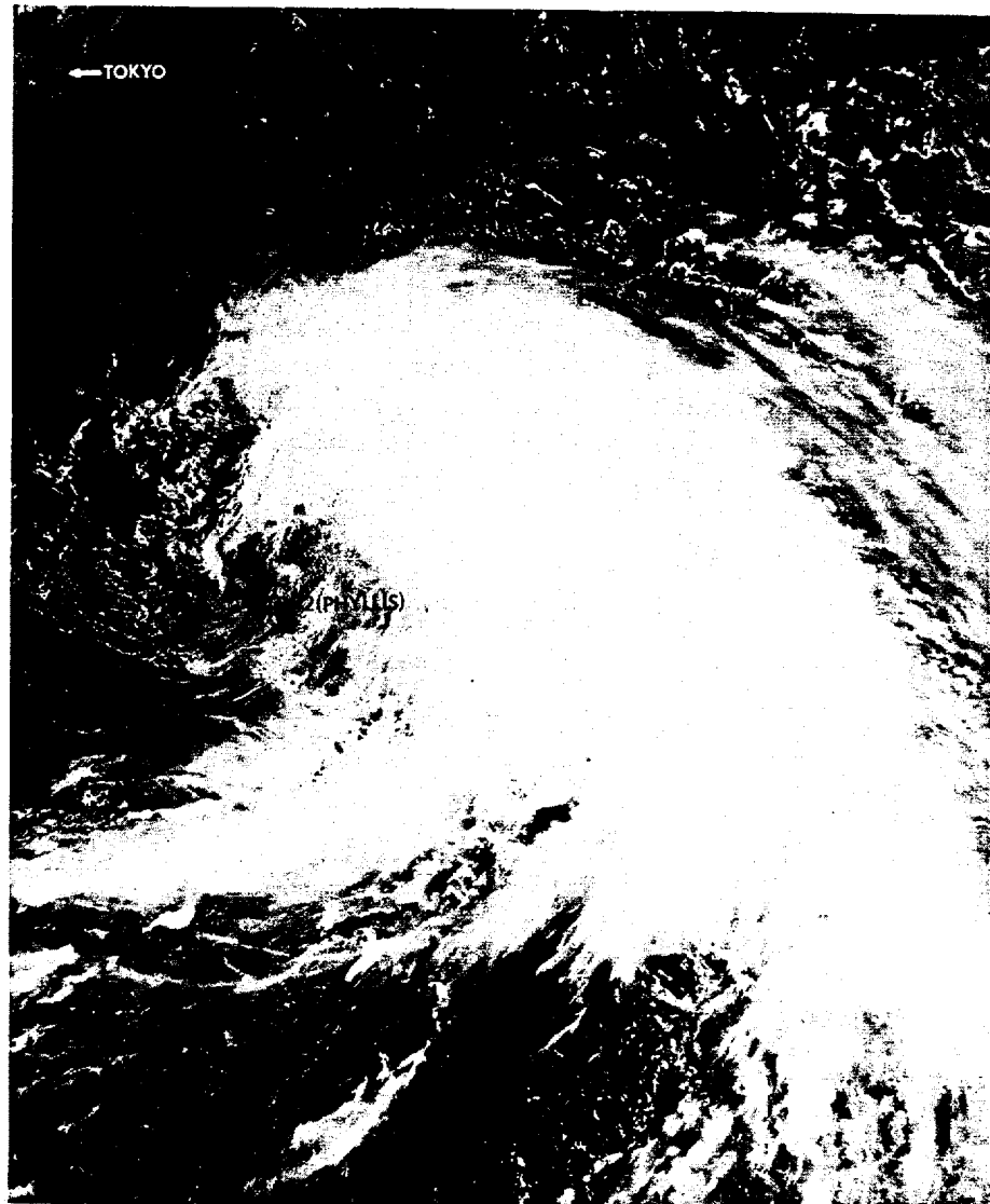
FIGURE 3-12-1. The exposed low level circulation center of Phyllis on 3 August 1981, 0410Z. The convective activity is limited to the east of her center of circulation. (NOAA 7 visual imagery)
