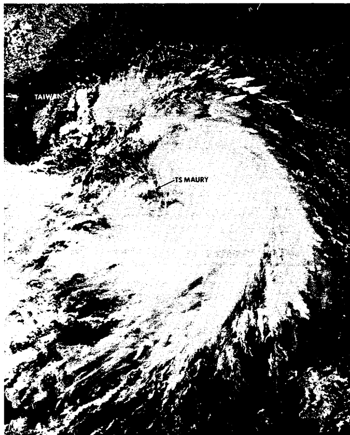
FIGURE 3-08-1. Tropical Storm Maury at 35 kts (18 m/sec) intensity, 18 July 1981, 0513Z. Maury's low-level center was exposed to the southwest of the main convection. (NOAA 7 visual imagery)
