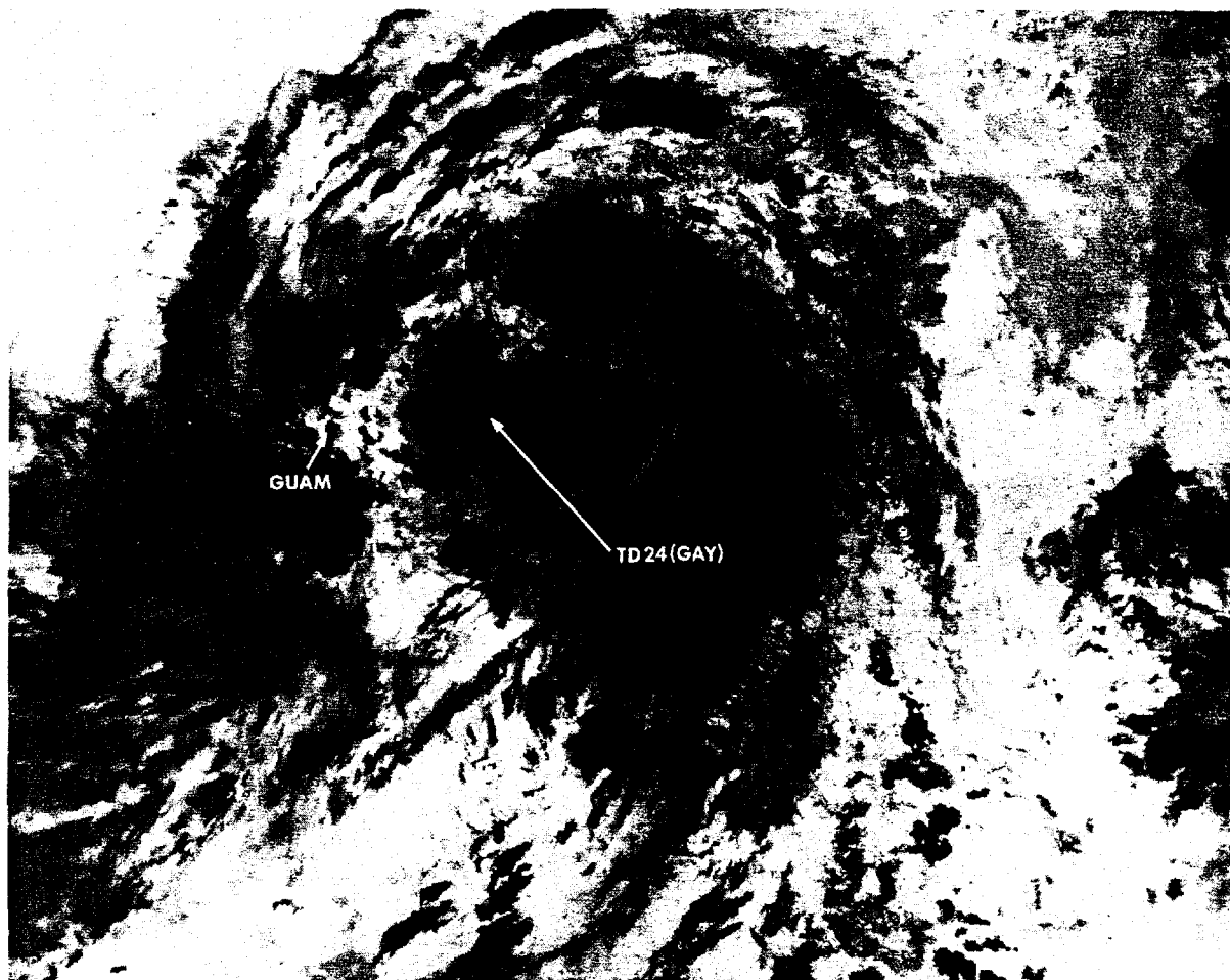
Figure 3-24-1. Tropical Depression 24 (Gay), 14 October 1981, 1614Z. At this time the initial warning with winds of 30 kt (15 m/sec) had been issued. The system was quickly upgraded to tropical storm status. The circulation center was approximately 100 nm (185 km) east of Guam. (NOAA 7 infrared imagery)
