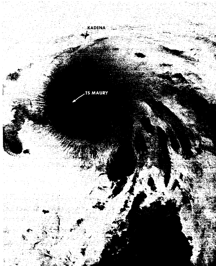
FIGURE 3-08-2. Tropical Storm Maury at 55 kts (28 m/sec) intensity, 18 July 1981, 1816Z. This imagery showed Maury had moved north during the preceding six hours instead of the forecasted northwestward movement. [NOAA 7 infrared imagery]
