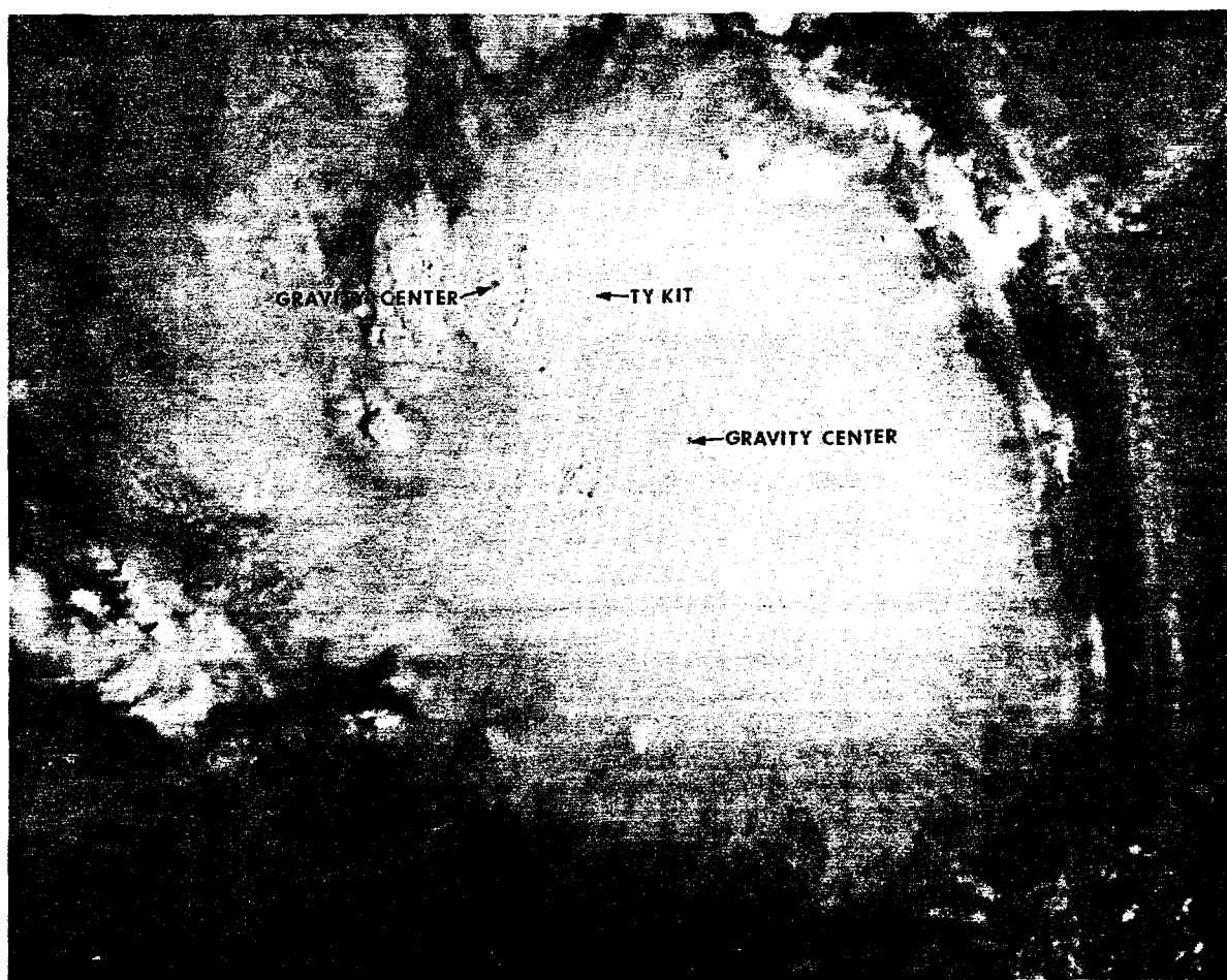
Figure 3-28-4. An intensifying Typhoon Kit, located 165 nm (306 km) west of Guam. Note the textured cloud pattern. Often referred to as gravity waves, these features are frequently seen in rapidly developing tropical cyclones prior to the development of an eye. About 14 hours later, Kit's eye was first detected, 132219Z December. (NOAA 6 visual imagery)
