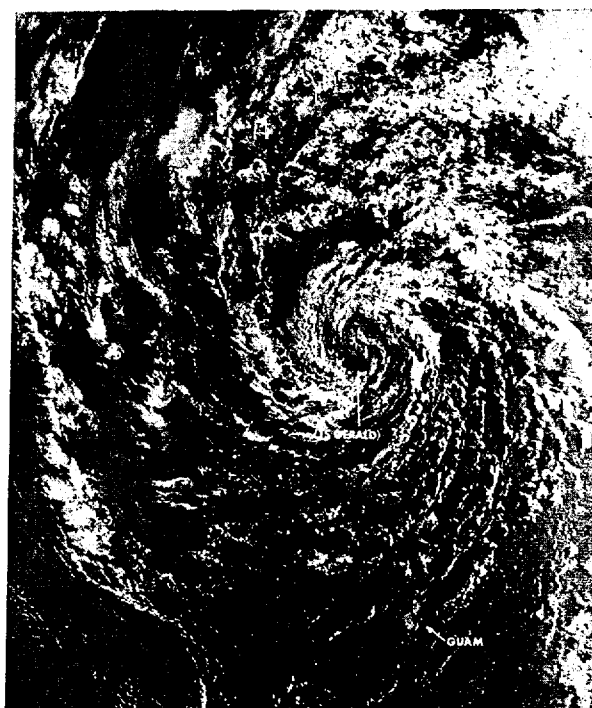
FIGURE 3-02-1. Tropical Storm Gerald as an exposed low-level circulation center north of Guam, 20 April 1981, 2228Z. (NOAA 6 visual imagery)
