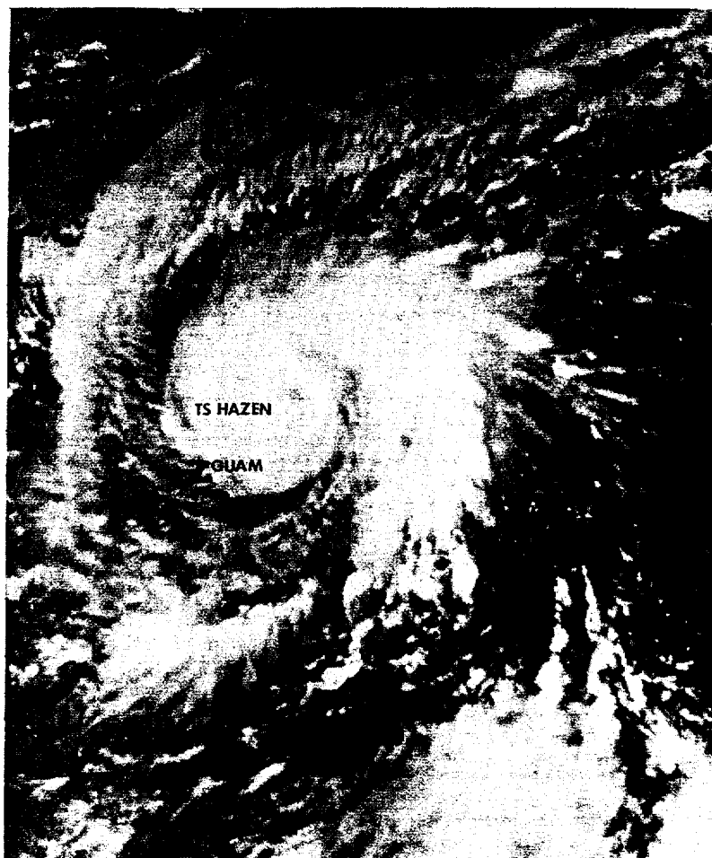
Figure 3-25-1. Tropical Storm Hazen at 55 kt (28 m/sec) intensity 110 nm (204 km) northeast of Guam shortly after crossing Saipan, 150430Z November. (NOAA 7 visual imagery)
