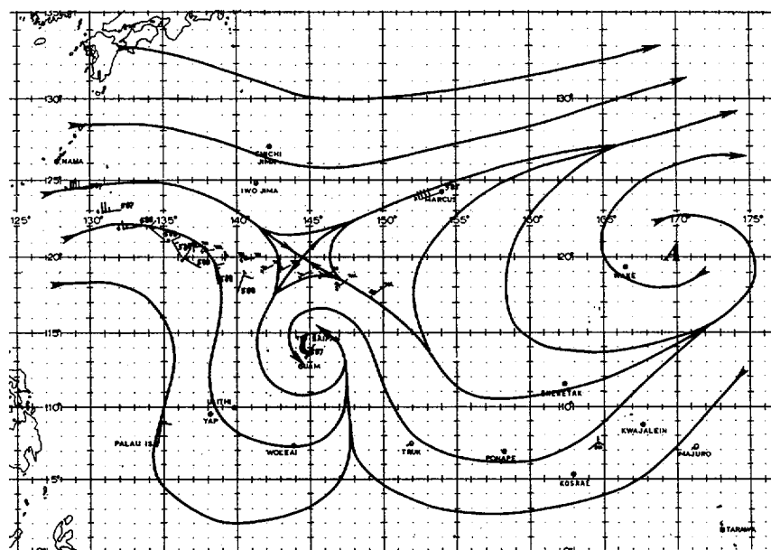
FIGURE 3-02-5. The 181200Z April 1981 mid-level streamline analysis based on 400- and 500-mb aircraft reconnaissance data.
