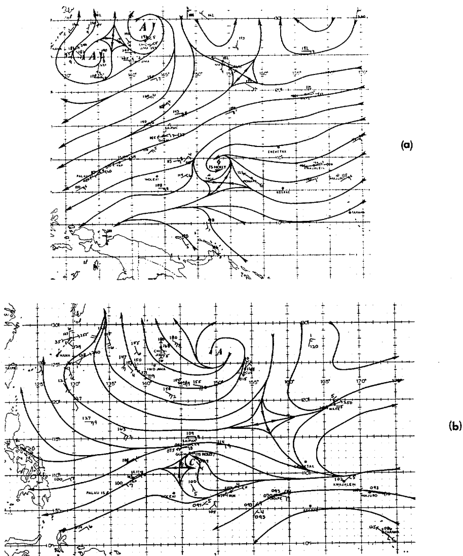
Figure 3-03-3. Surface (—)/gradient (—) level analyses: (a) at 020000Z which was typical during Holly's period of slow movement and (b) at 070000Z showing the pattern as Holly began to accelerate. Winds are in knots.
