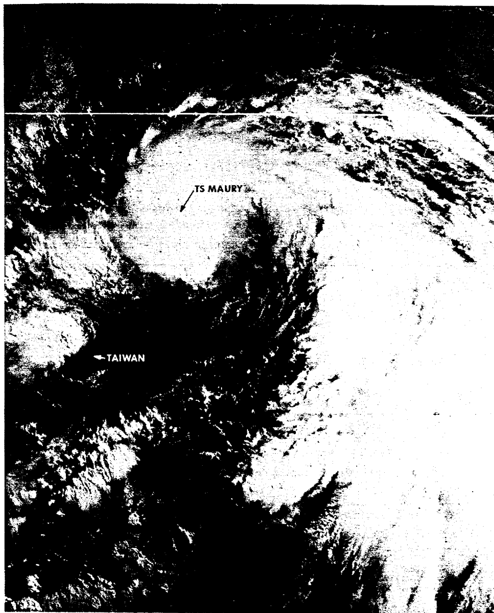
FIGURE 3-08-3. Tropical Storm Maury showed westward movement at the time of this imagery, 18 July 1981, 2305Z. Maury 10 hours before making landfall at the northern tip of Taiwan. (NOAA 6 visual imagery)
