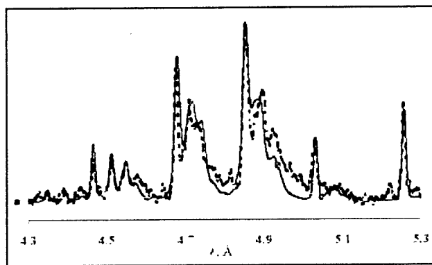
Figure 5. Comparison of the experimental 62μm Mo wire x-pinch spectrum produced on October 10, 2000 (dotted line) and theoretical spectrum (solid line) at 700eV and 10^{22} \text{ cm}^{-3} with 10% hot electrons at 10keV.
