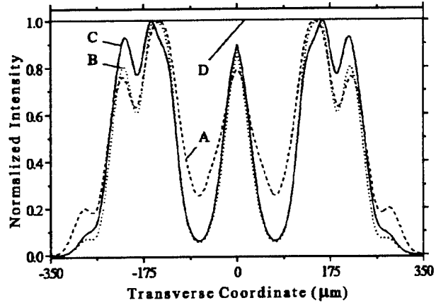
FIG. 6. Normalized intensity distributions of the partially coherent field at the guide exit calculated using Eqs. (10)–(14). The parameters of the light at the guide entrance: A, |\mu|=1 ; B, |\mu|=0.85 ; C, |\mu|=0.75 ; and D, |\mu|=0 .
