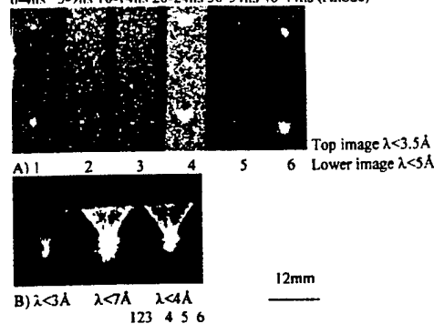
Ti x-pinch SHOT#30 (May 18, 2000)
