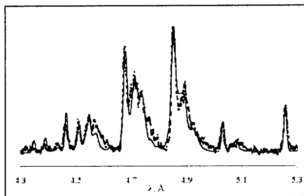
Figure 5. Comparison of the experimental 62μm Mo wire x-pinch spectrum produced on October 10, 2000 (dotted line) and theoretical spectrum (solid line) at 700eV and 10^{22} \text{ cm}^{-3} with 10% hot electrons at 10keV.
