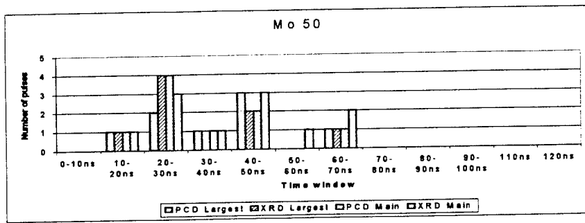
Fig. 15. The time distribution of PCD and XRD signals for a 50 \mu m Mo x-pinch. Largest: the signals with a maximum amplitude; main: signals with an amplitude from 0.9 to 0.3 of the largest value. The data are based on 8 shots.
