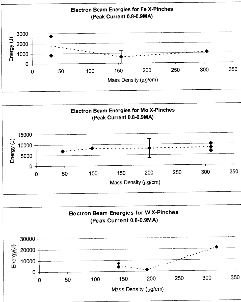
Figure 4.39. The experimental estimation of the energy needed to generate the observed holes at the points of connection of the wires with the anode of an x-pinch vs. mass density of wires.
