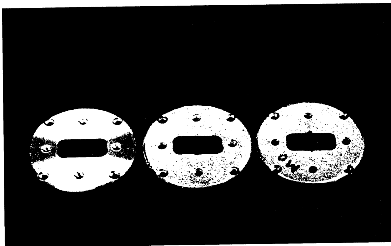
Figure 4.15. An anode electrode before (left) and after the shot for Fe (center) and Mo x-pinch (right). A strong increasing of the diameter of holes in plate for Mo is clearly seen.
