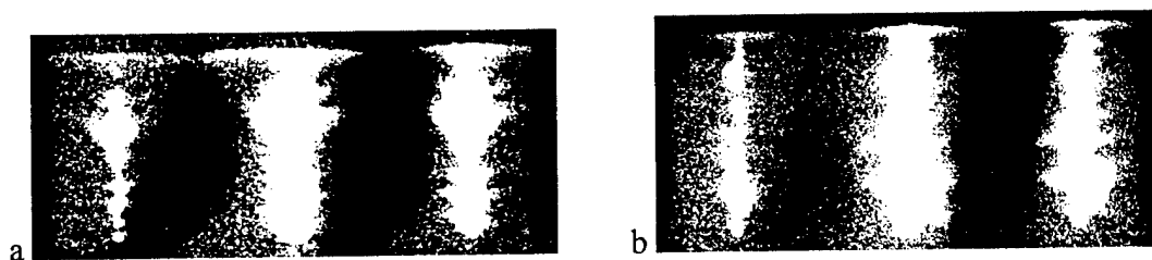
Figure 3.2.4. Time integrated x-ray images of single 76\text{ }\mu\text{m} Ti wire z-pinch plasma recorded on shots #74 (a) and #75 (b), respectively.
