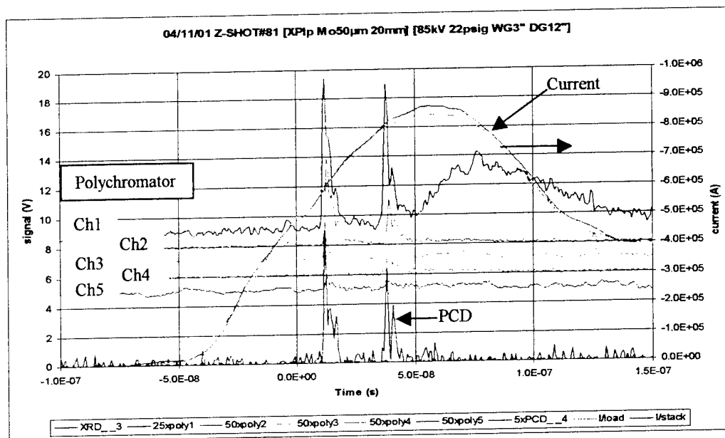
Fig. 4. X-ray signals from an 50 \mu\text{m} Mo x-pinch (shot # 81, April 11, 2001). "Polychromator" (chan.1: \lambda=5.21 \text{\AA} , Ne-like Mo; chan.2: \lambda=4.80 \text{\AA} , Na-like Mo; chan.3: \lambda=1.94 \text{\AA} , "cold" K_{\alpha}\text{Fe} ; chan.4: \lambda=4.41 \text{\AA} , Ne-like Mo; chan.5: \lambda=5.5 \text{\AA} , continuum, control line). PCD (with 25 \mu\text{m} kapton filter) response versus the time. Note, that maximum of "Polychromator" signals correlated in time with PCD signal (Mo L-shell radiation).
