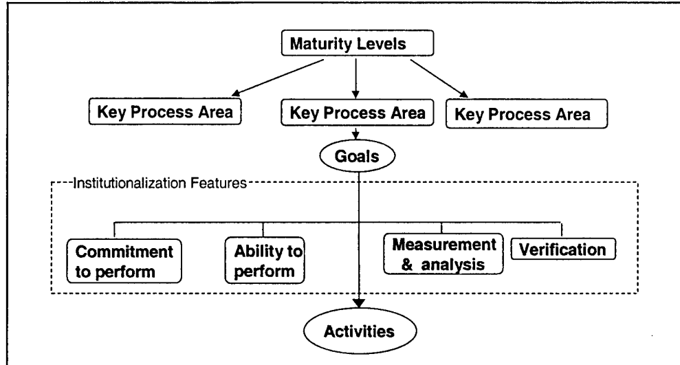
Figure 1. SA-CMM Architecture
