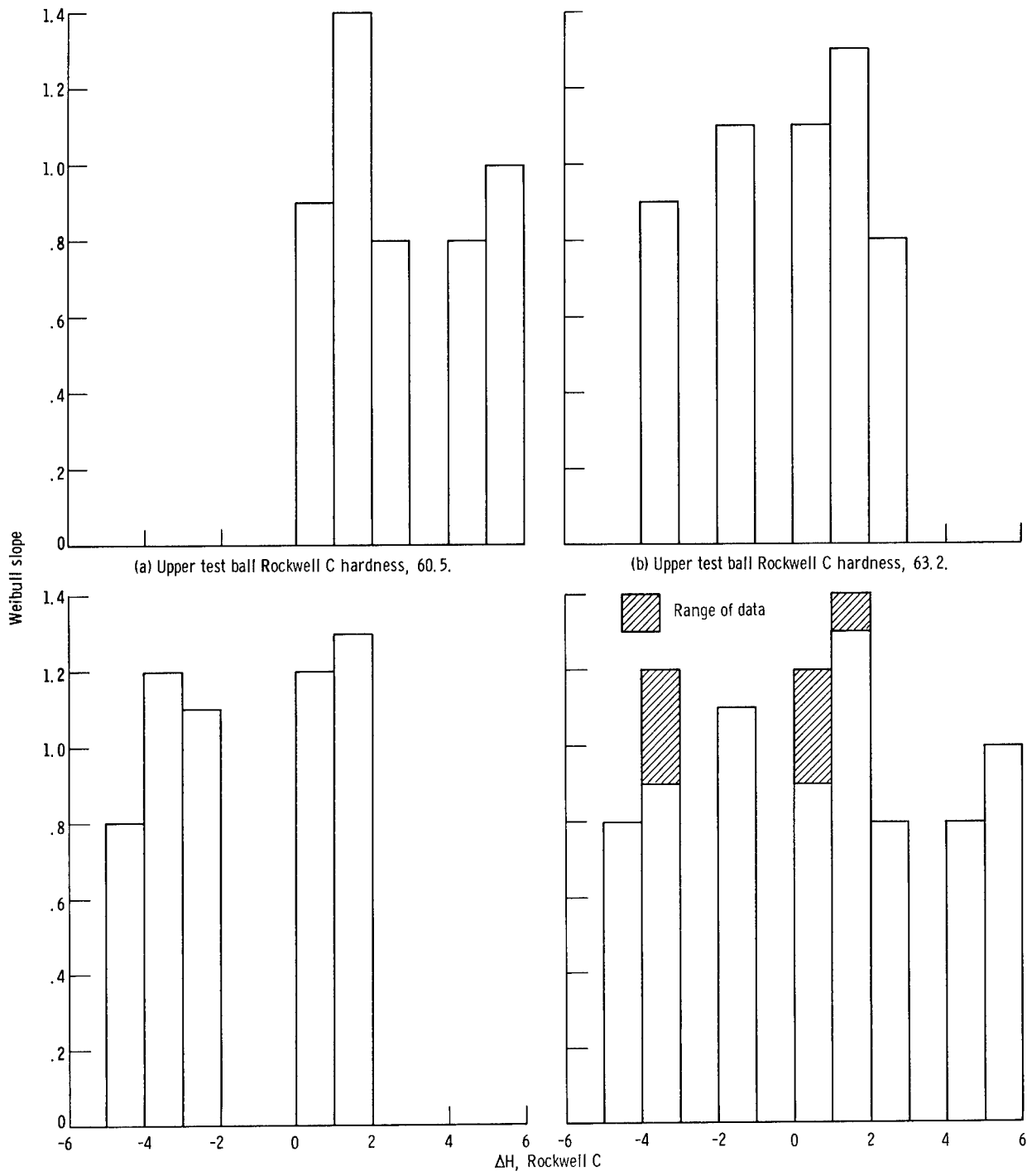
(a) Upper test ball Rockwell C hardness, 60.5. (b) Upper test ball Rockwell C hardness, 63.2. (c) Upper test ball Rockwell C hardness, 65.2. (d) Summary of Weibull slopes. Figure 8. - Weibull slope as function of \Delta H (difference in Rockwell C hardness between lower test balls and upper test ball) for upper and lower test balls of varying hardnesses. Five-ball fatigue tester; initial maximum Hertz stress, 800 000 psi; system thrust load, 390 pounds; contact angle, 30^\circ ; room temperature; material, SAE 52100 steel (data from ref. 1).
