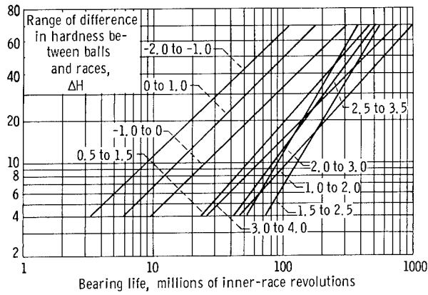
(j) Summary of fatigue lives.
