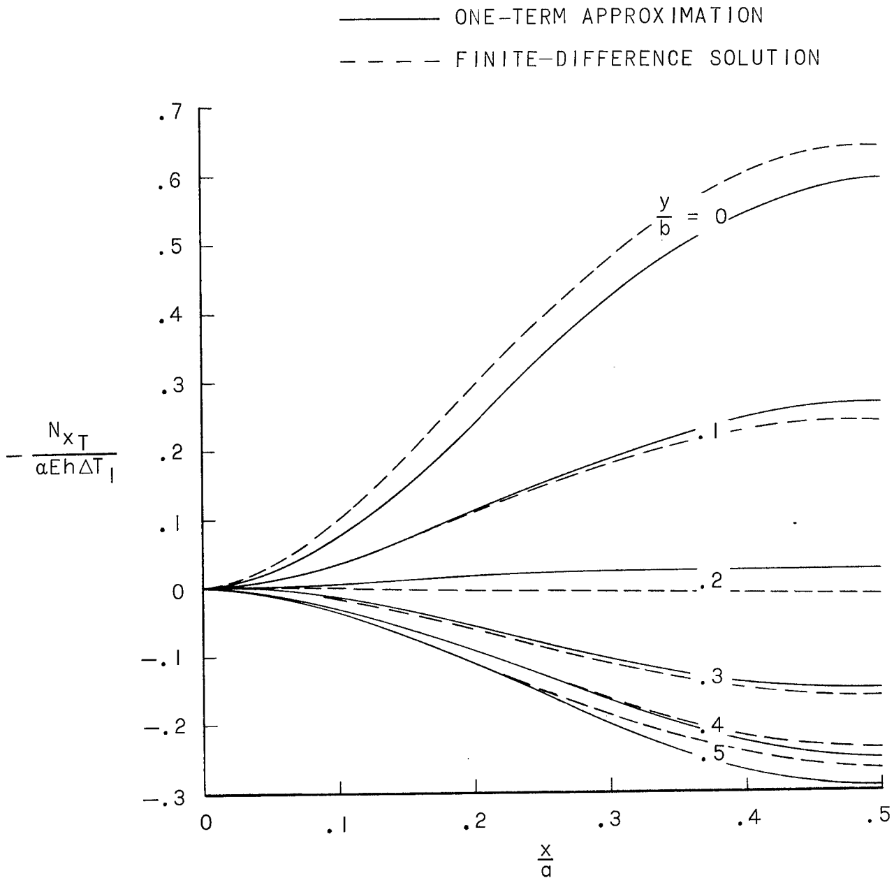
Figure 2.- Variation of stress resultant N_{xT} with x . T = 16\Delta T_1 \left(\frac{x}{a}\right) \left(1 - \frac{x}{a}\right) \left(\frac{y}{b}\right) \left(1 - \frac{y}{b}\right) ; \frac{a}{b} = 1 ; symmetric about \frac{x}{a} = 0.5 and \frac{y}{b} = 0.5 .
