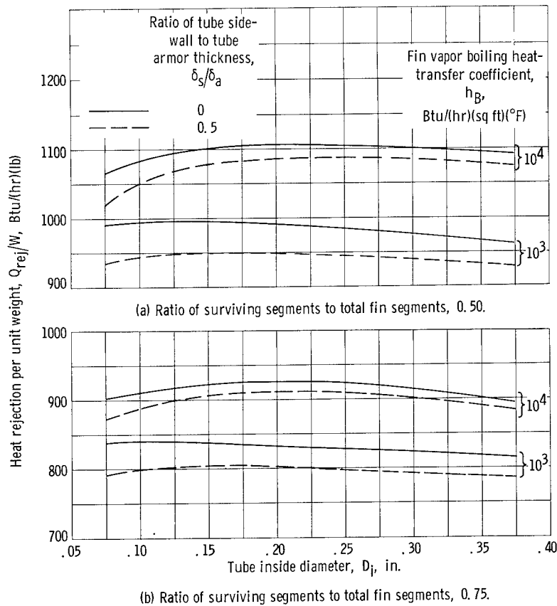
Figure 5. - Vapor-chamber fin-tube radiator peak heat rejection per unit weight. Fin segment planform area, 80 square inches; capillary weight, 0.10 pound per square foot; ratio of fin vapor boiling to fin vapor condensing heat-transfer coefficient, 1.0.
