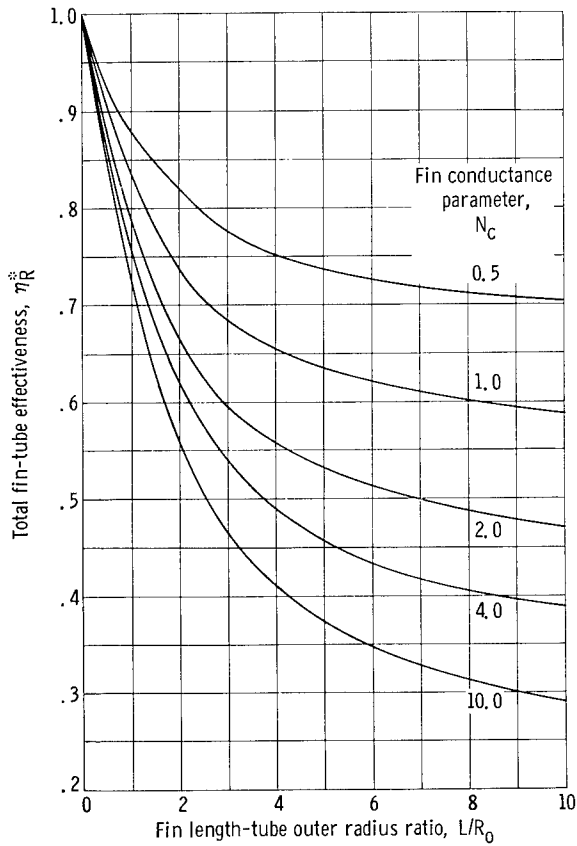
Figure 32. - Total fin-tube effectiveness plotted against fin length-tube outer radius ratio L/R_0 for central fin-tube radiator.
