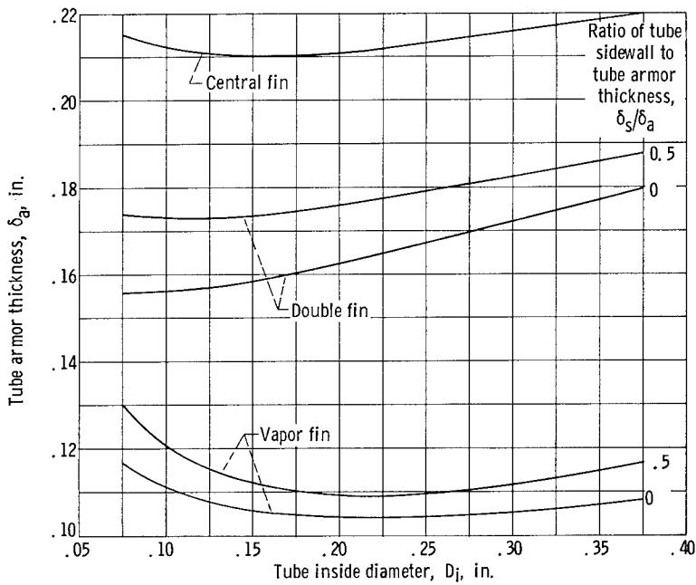
Figure 27. - Comparison of tube armor thickness at peak heat rejection per unit weight. Fin segment planform area, 80 square inches; h_B = h_C = 10^4 Btu/(hr)(sq ft)( ^{\circ} F); tube-header nonpenetration probability, 0.90; ratio of surviving segments to total fin segments, 0.75.
