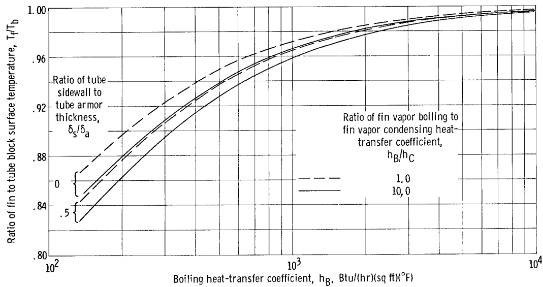
Figure 36. - Variation of ratio of fin to block surface temperature with boiling heat-transfer coefficient for vapor-chamber fin-tube radiator. Fin segment planform area, 80 square inches; capillary weight, 0.1 pound per square foot; tube-header nonpenetration probability, 0.90.
