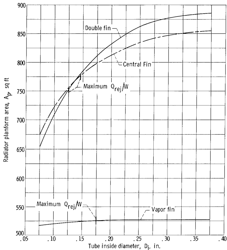
Figure 22. - Comparison of planform area at peak heat rejection per unit weight. Fin segment planform area, 80 square inches; h_B = h_C = 10^4 Btu/(hr)(sq ft)( ^{\circ} F); tube-header nonpenetration probability, 0.90; ratio of surviving segments to total fin segments, 0.75; ratio of tube sidewall to tube armor thickness, 0.5.
