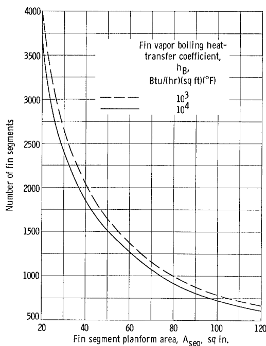
Figure 12. - Variation of number of fin segments with fin segment planform area at maximum heat rejection per unit weight. Capillary weight, 0.1 pounds per square foot; ratio of fin vapor boiling to fin vapor condensing heat-transfer coefficient, 1.0; tube-header nonpenetration probability, 0.90; ratio of surviving segments to total fin segments, 0.75; probability of N_S or more segments not punctured, S , 0.90.
