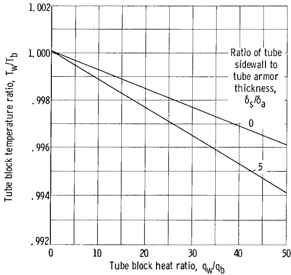
Figure 35. - Ratio of tube block sidewall to outer wall temperature ratio for vapor chamber fin-tube radiator. Static fluid inlet temperature, 836° R; fin segment plan-form area, 80 square inches; capillary weight, 0.10 pound per square foot; h_B = h_C = 10^4 Btu/(hr)(sq ft)(°F); tube inside diameter, 0.1 inch.
