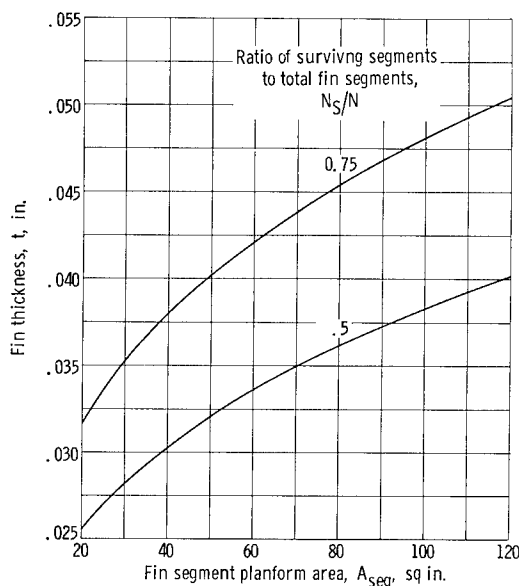
Figure 11. - Variation of fin thickness with fin segment planform area at maximum heat rejection per unit weight for vapor-chamber fin-tube radiator. Capillary weight, 0.1 pound per square foot; h_B = h_C = 10^4 Btu/(hr)(sq ft)(°F); probability of N_S or more segments not punctured, S , 0.90.
