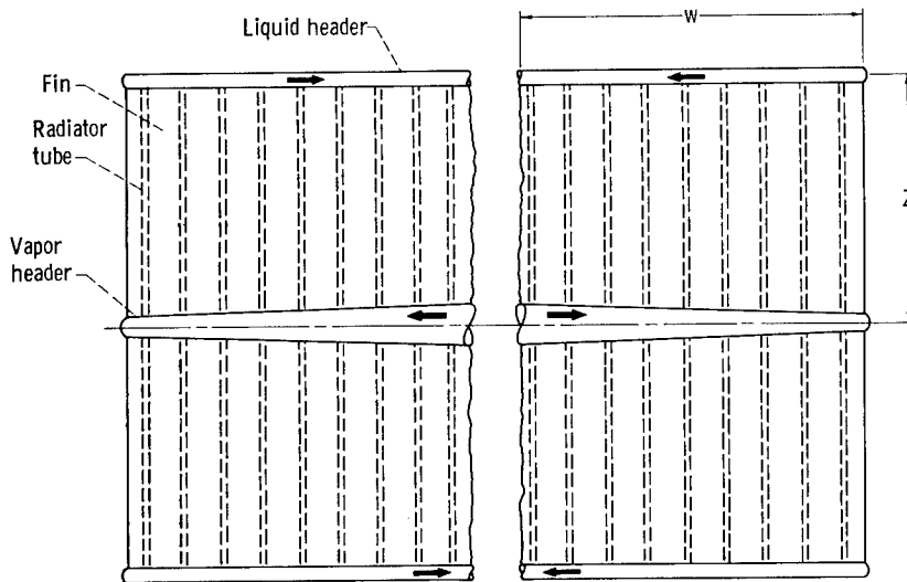
Figure 1. - Four-panel fin-tube radiator.
