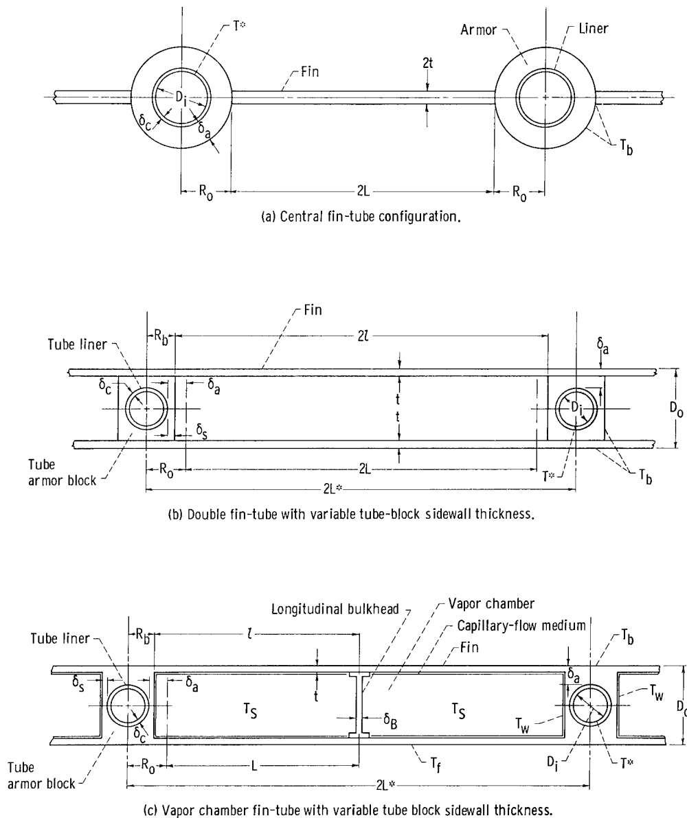
Figure 2. - Cross sections of radiator fin-tube configurations.
