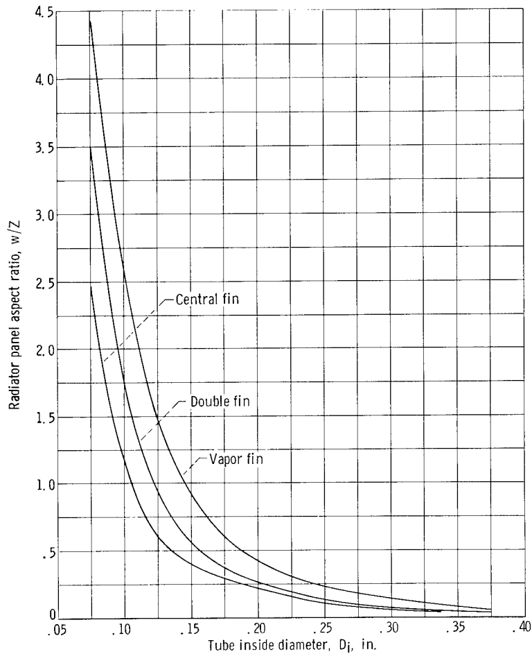
Figure 28. - Comparison of radiator panel aspect ratio at peak heat rejection per unit weight. Fin segment planform area, 80 square inches; h_B = h_C = 10^4 Btu/(hr)(sq ft)(°F); tube-header nonpenetration probability, 0.90; ratio of surviving segments to total fin segments, 0.75; ratio of tube sidewall to tube armor thickness, 0.5.
