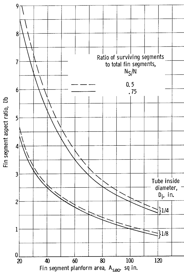
Figure 13. - Fin segment aspect ratio plotted against fin segment planform area for vapor-chamber fin-tube radiator. Capillary weight, 0.1 pound per square foot; h_B = h_C = 10^4 Btu/(hr)(sq ft)(°F); tube-header nonpenetration probability, 0.90; ratio of tube sidewall to tube armor thickness, 0.5.
