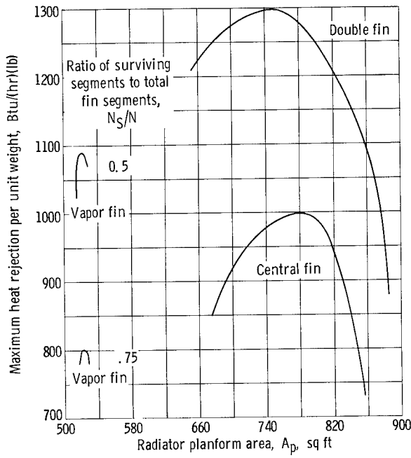
Figure 23. - Maximum heat rejection per unit weight plotted against radiator planform area. Fin segment planform area, 80 square inches; h_B = h_C = 10^4 Btu/(hr)(sq ft)(°F); tube-header nonpenetration probability, 0.90; ratio of tube sidewall to tube armor thickness, 0.5.
