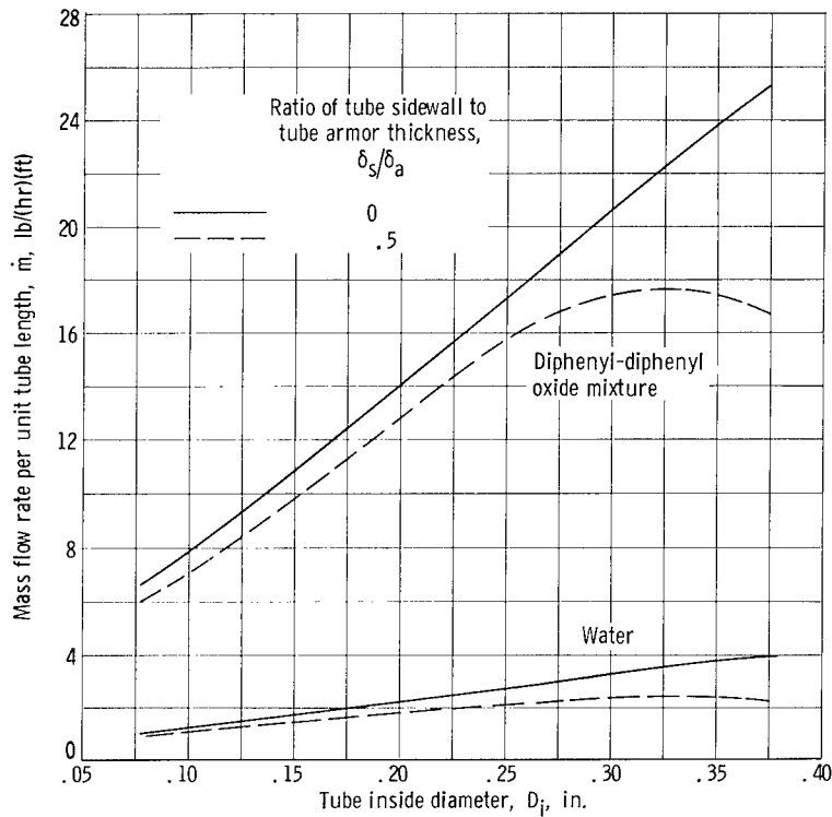
Figure 15. - Capillary fluid flow rate for vapor-chamber fin-tube radiator. Fin segment planform area, 80 square inches; h_B = h_C = 10^4 Btu/(hr)(sq ft)( ^{\circ} F); ratio of surviving segments to total fin segments, 0.75.
