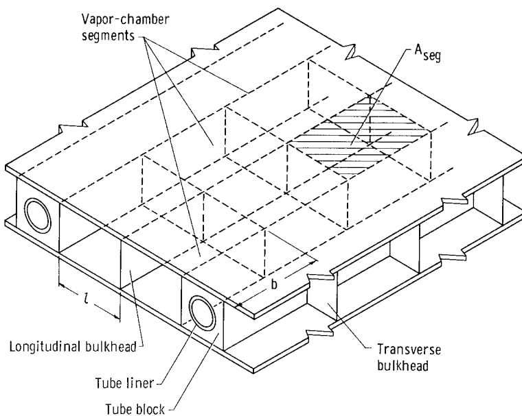
Figure 3. - Isometric drawing of vapor-chamber fin-tube configuration.
