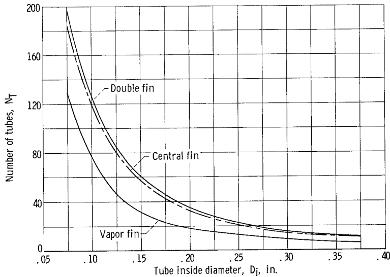
Figure 24. - Comparison of number of radiator tubes at peak heat rejection per unit weight at each diameter. Fin segment planform area, 80 square inches; h_B = h_C = 10^4 Btu/(hr)(sq ft)(°F); tube-header nonpenetration probability, 0.90; ratio of surviving segments to total fin segments, 0.75; ratio of tube sidewall to tube armor thickness, 0.5.
