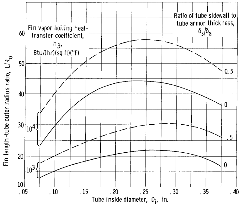
Figure 10. - Fin length-tube outer radius ratio L/R_o at peak heat rejection per unit weight for vapor-chamber fin-tube radiator. Fin segment planform area, 80 square inches; ratio of fin vapor boiling to fin vapor condensing heat-transfer coefficient, 1.0; tube-header nonpenetration probability, 0.90; ratio of surviving segments to total fin segments, 0.75.
