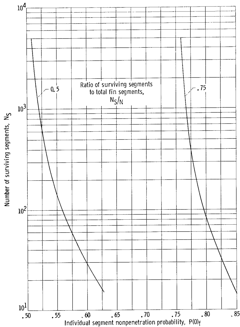
Figure 37. - Nonpenetration probability of one segment of segmented vapor-chamber fin-tube radiator. Probability of N_S or more segments not punctured, S , 0.90.
