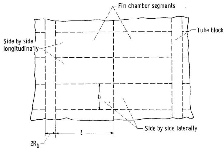
Figure 16. - Vapor-chamber punctured fin segment arrangement.
