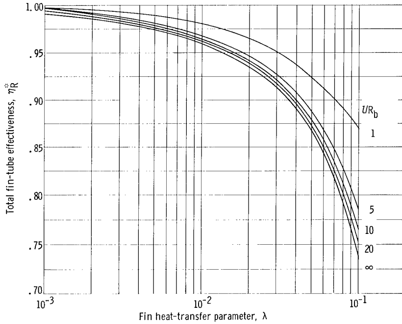
Figure 34. - Total fin-tube effectiveness for vapor-chamber fin-tube radiator.
