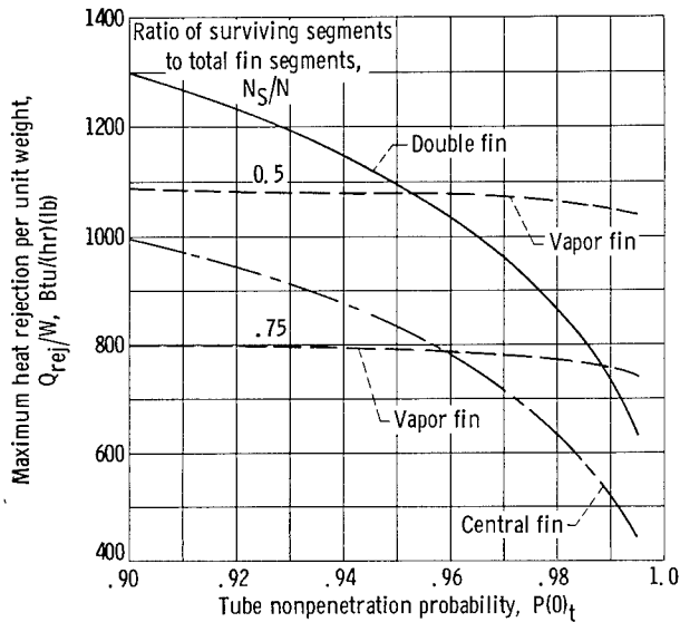
Figure 21. - Comparison of maximum heat rejection per unit weight plotted against radiator tube nonpenetration probability. Fin segment planform area, 80 square inches; capillary weight, 0.1 pound per square foot; h_B = h_C = 10^4 Btu/(hr)(sq ft)(°F); ratio of tube sidewall to tube armor thickness, 0.5; probability of N_S or more segments not punctured, S , 0.90.
