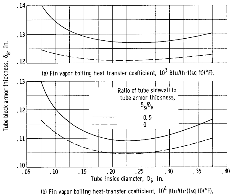
Figure 9. - Variation of tube block-armor thickness at peak heat rejection per unit weight with tube inside diameter vapor-chamber fin tube radiator. Fin segment planform area, 80 square inches; capillary weight, 0.1 pounds per square foot; ratio of fin vapor boiling to fin vapor condensing heat-transfer coefficient, 1.0; tube-header nonpenetration probability, 0.90; ratio of surviving segments to total fin segments, 0.75.
