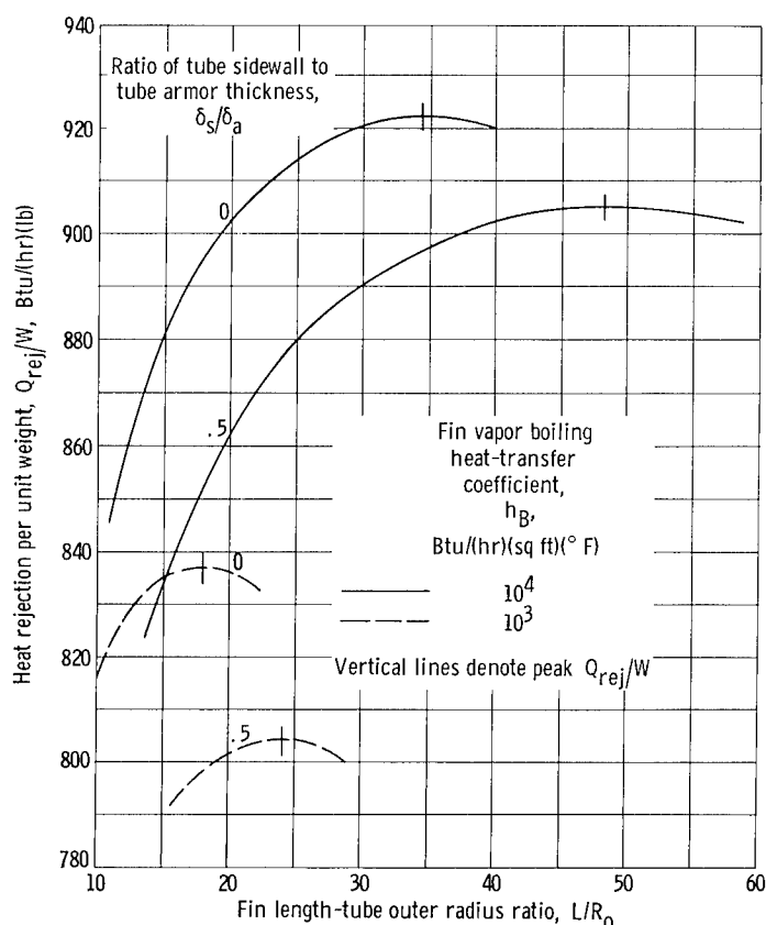
Figure 4. - Variations of heat rejection per unit weight with fin length-tube outer radius ratio for vapor-chamber fin-tube radiator. Fin segment planform area, 80 square inches; tube inside diameter, 0.15 inch; capillary weight, 0.1 pound per square foot; ratio of fin vapor boiling to fin vapor condensing heat-transfer coefficient, 1.0; tube-header nonpenetration probability, 0.90; ratio of surviving segments to total fin segments, 0.75.
