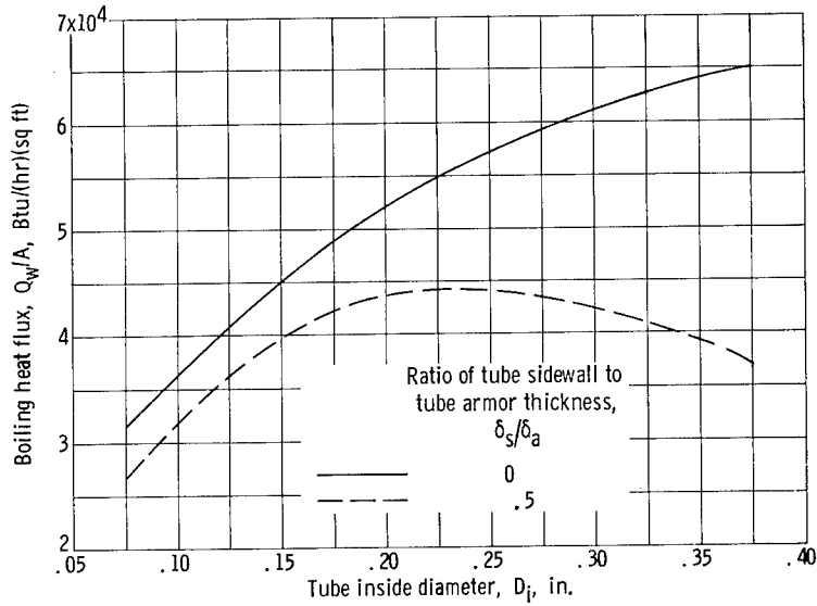
Figure 14. - Capillary fluid boiling heat flux for vapor-chamber fin-tube radiator. Fin segment planform area, 80 square inches; h_B = h_C = 10^4 Btu/(hr)(sq ft)( ^{\circ} F); ratio of surviving segments to total fin segments, 0.75.
