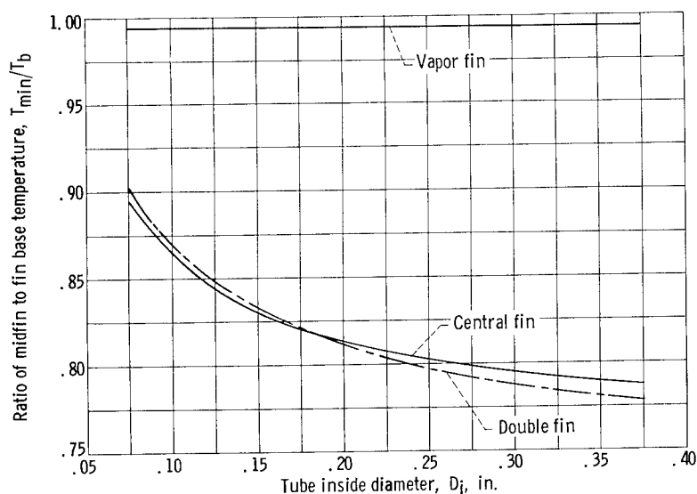
Figure 31. - Comparison of ratio of midfin to fin base temperature at peak heat rejection per unit weight. h_B = h_C = 10^4 Btu/(hr)(sq ft)(°F); tube-header non-penetration probability, 0.90; ratio of surviving segments to total fin segments, 0.75; ratio of tube sidewall to tube armor thickness, 0.5.
