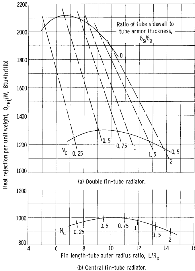
Figure 18. - Variations of heat rejection per unit weight with fin length-tube outer radius ratio L/R_o . Tube-header nonpenetration probability, 0.90; tube inside diameter, 0.125 inch.
