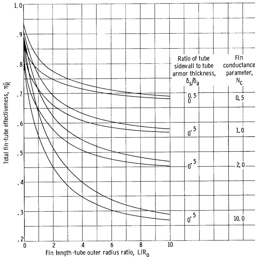
Figure 33. - Total fin-tube effectiveness plotted against fin length-tube outer radius ratio L/R_0 for double fin-tube radiator.
