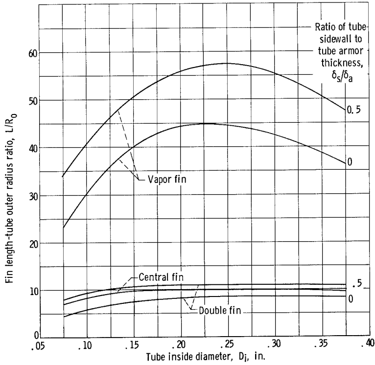
Figure 26. - Comparison of radiator fin length-tube outer radius ratio L/R_0 at peak heat rejection per unit weight. Fin segment planform area, 80 square inches; h_B = h_C = 10^4 Btu/(hr)(sq ft)( ^{\circ} F); ratio of surviving segments to total fin segments, 0.75.
