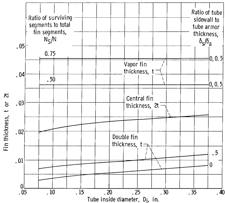
Figure 25. - Comparison of fin thickness at peak heat rejection per unit weight. Fin segment planform area, 80 square inches; h_B = h_C = 10^4 Btu/(hr)(sq ft)(°F); tube-header nonpenetration probability, 0.90.
