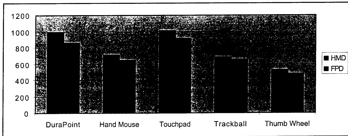
Figure 6.5. Mean homing time (ms) for each device for the last two blocks.
