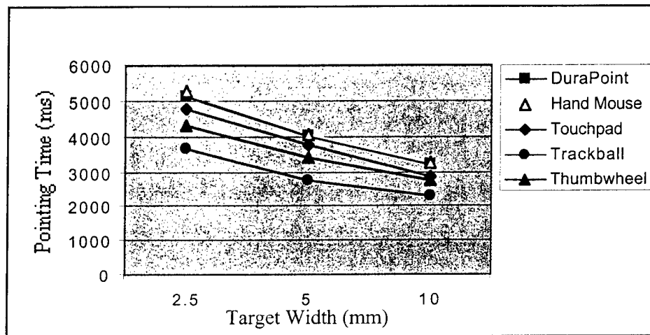
Figure 6.10. Effect of target width on pointing time, n=20.
