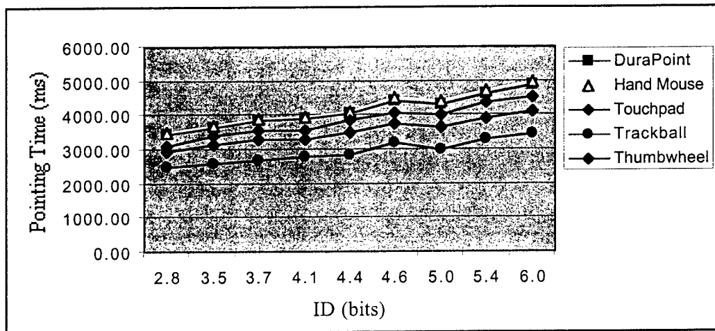
Figure 6.12. Mean pointing time using the MacKenzie ID, n=20.
