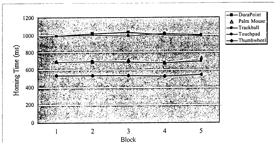
Figure 6.2. Homing Time (ms) with HMD by block across participants. n=10.
