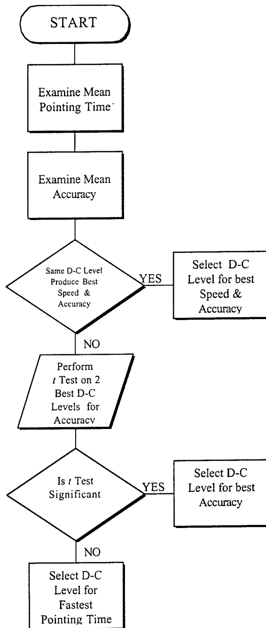
Figure 4.0. Decision process for determining the optimum D-C gain for each pointing device.
