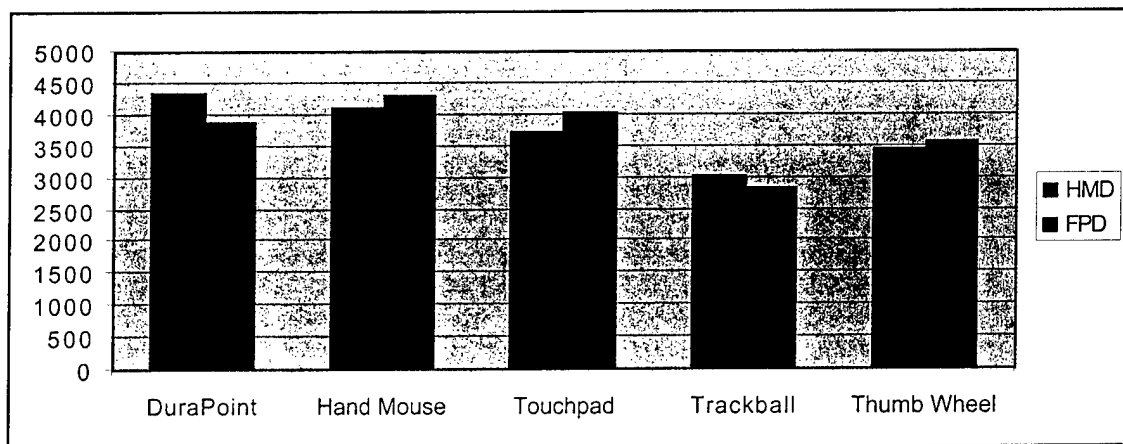
Figure 6.4. Mean pointing time (ms) for each device during last two blocks.
