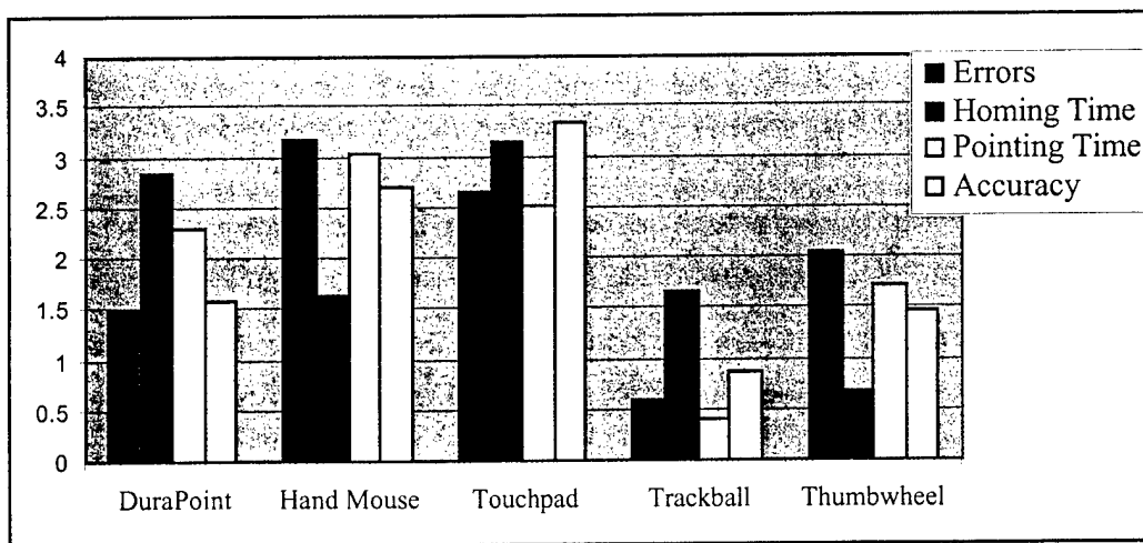
Figure 6.9. Composite results for each device with the FPD.
