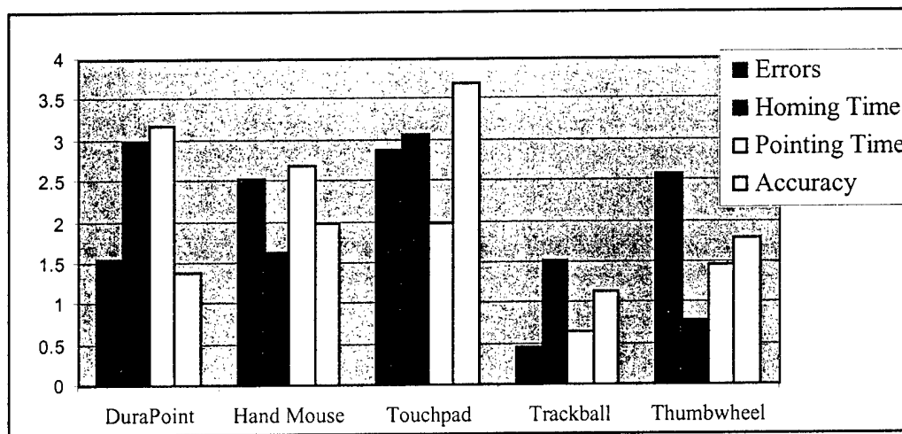
Figure 6.8. Composite results for each device with the HMD.
