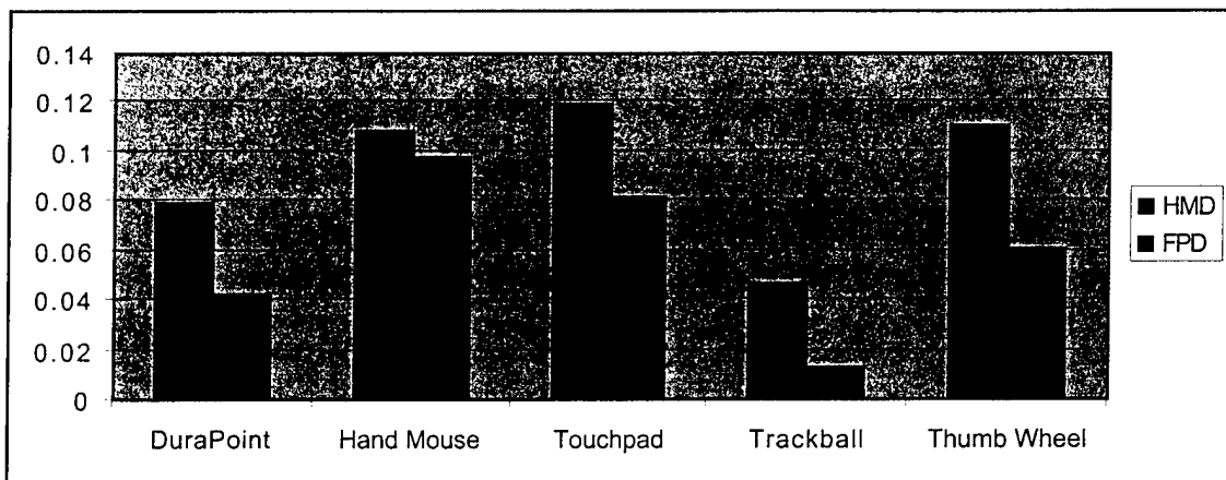
Figure 6.7. Mean number of error for each device for the last two blocks.
