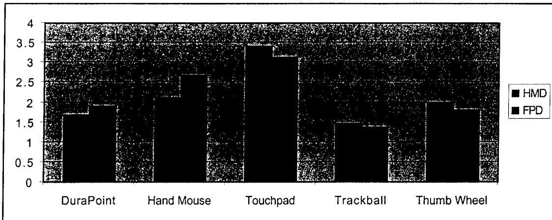
Figure 6.6. Mean accuracy value (mm) for each device for the last two blocks.
