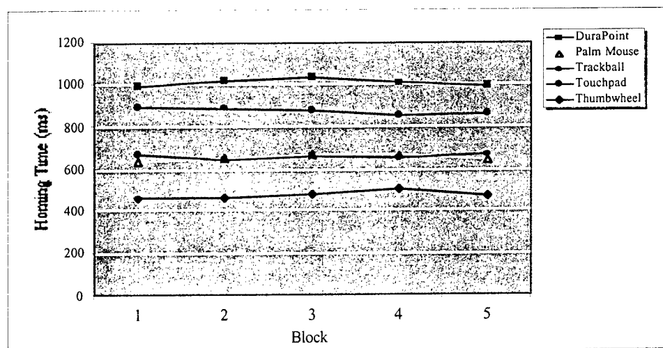
Figure 6.3. Homing Time (ms) with FPD by block across participants. n=10.
