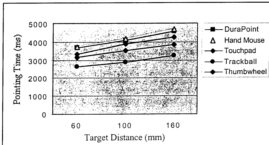
Figure 6.11. Effect of target distance on pointing time, n=20.
