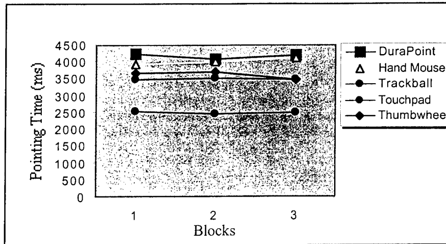
Figure 4.0: Mean Pointing Time (ms) with HMD by block across participants, n=5.
