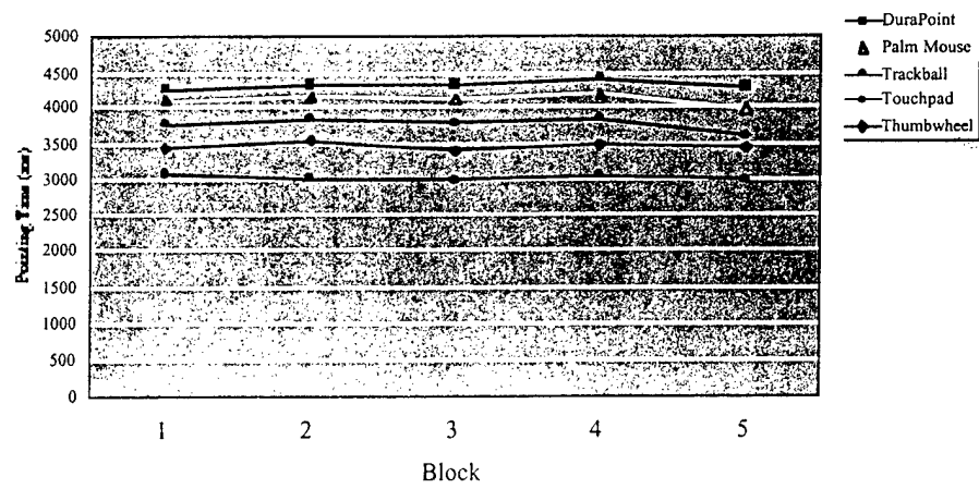
Figure 6.0. Pointing Time (ms) with HMD by block across subjects. n=10.
