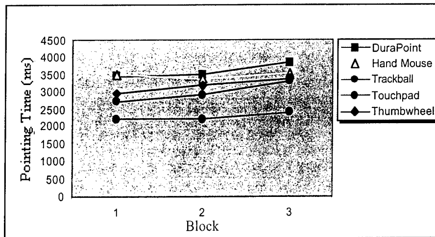
Figure 4.1: Mean Pointing Time (ms) with FPD by block across participants, n=5.
