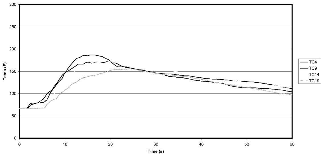
Figure A-62: Test 8 Row 4 Ceiling Temperatures
