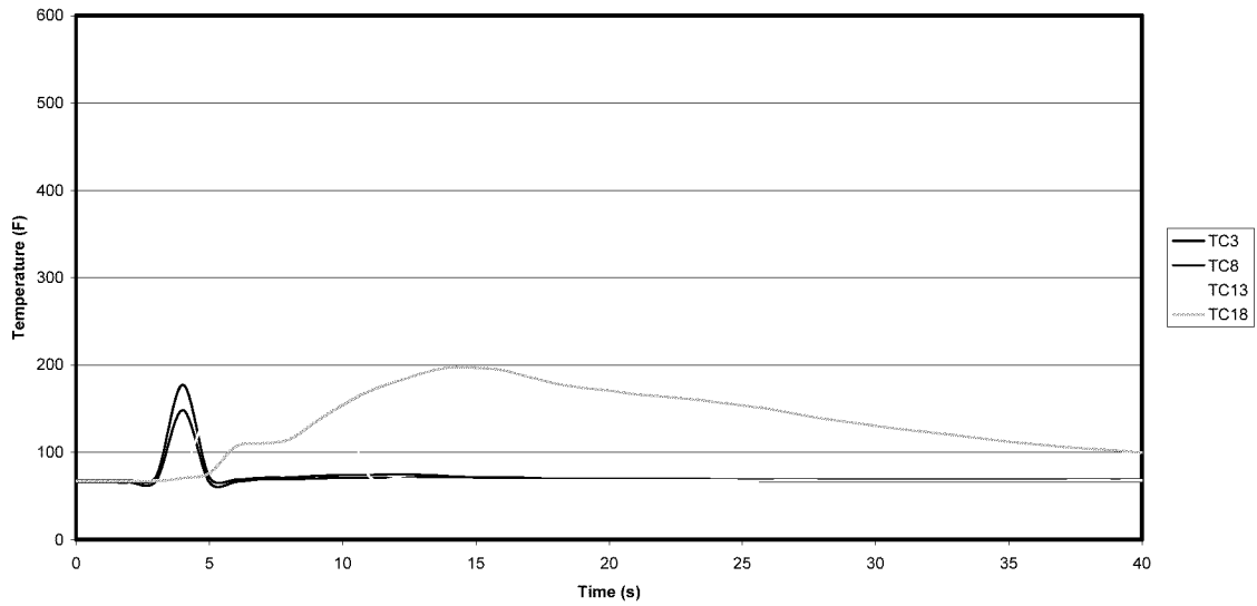
Figure A-33: Test 4 Row 3 Ceiling Temperatures
