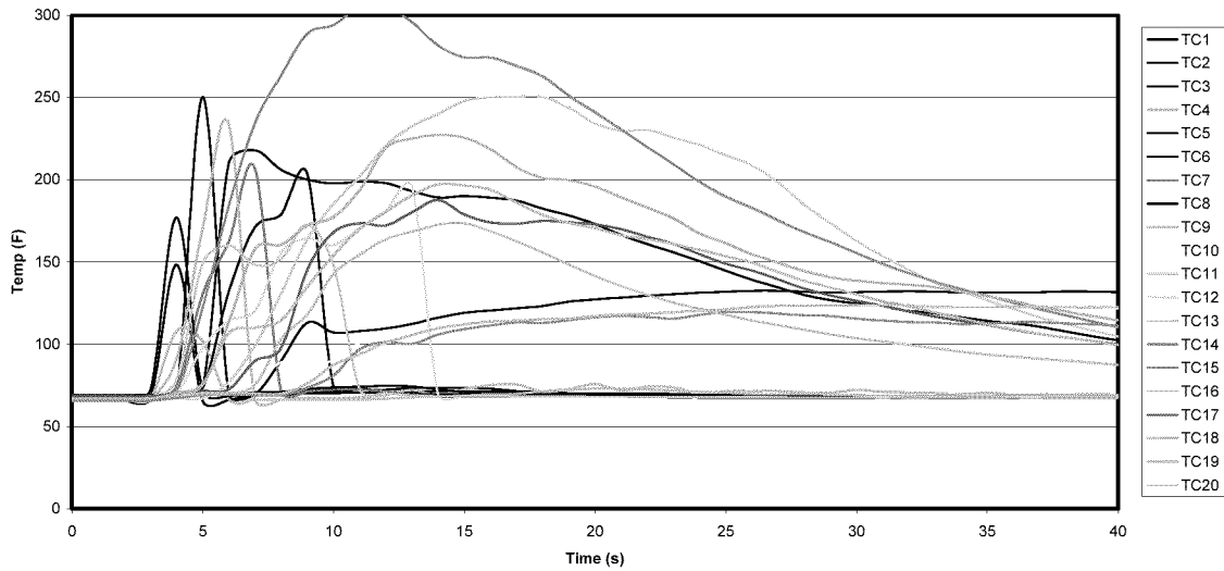
Ceiling Temperatures Spontaneous Combustion Scenario 9 February '01 - Test 4
