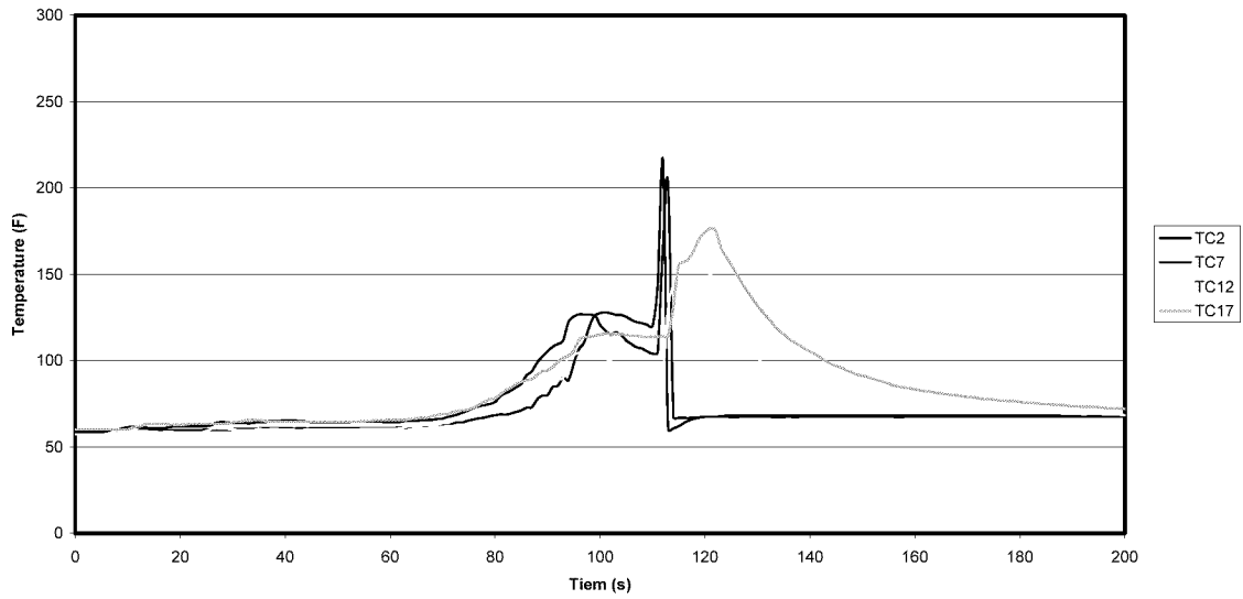
Row 2 Temperature Modified Fuel Spill Scenario 6 February '01 - Test 2
