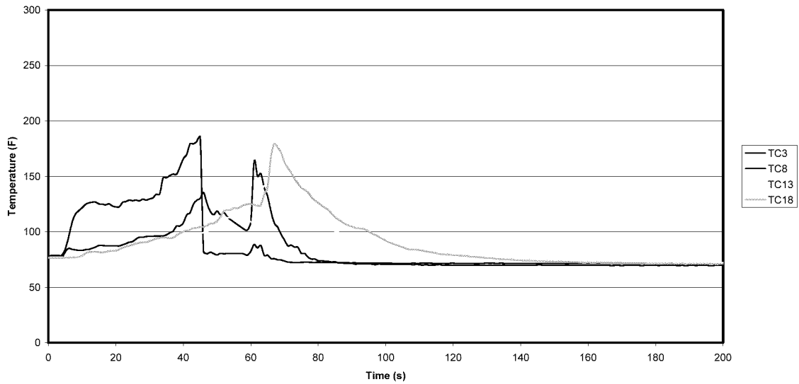
Figure A-26: Test 10 Row 3 Ceiling Temperatures
