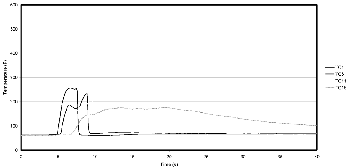
Figure A-38: Test 5 Row 1 Ceiling Temperatures
