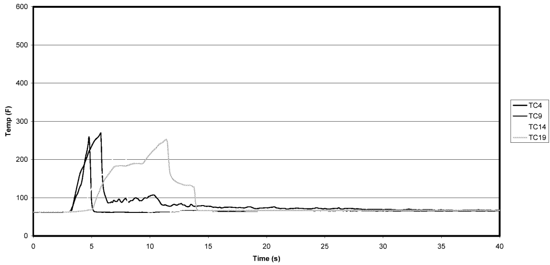
Figure A-41: Test 5 Row 4 Ceiling Temperatures
