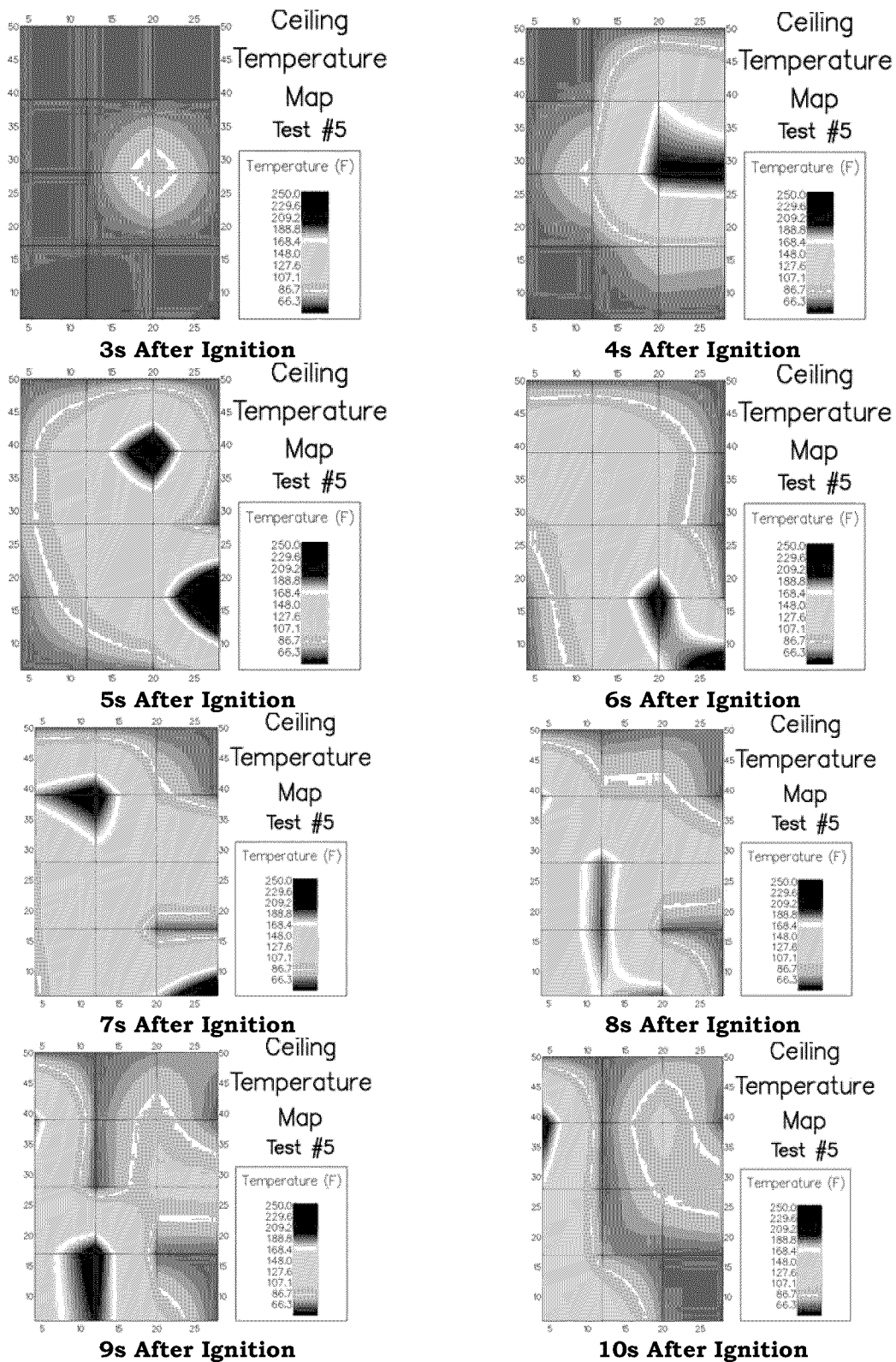
Figure A-43: Test 5 Ceiling Temperatures @ 1 Second Intervals
