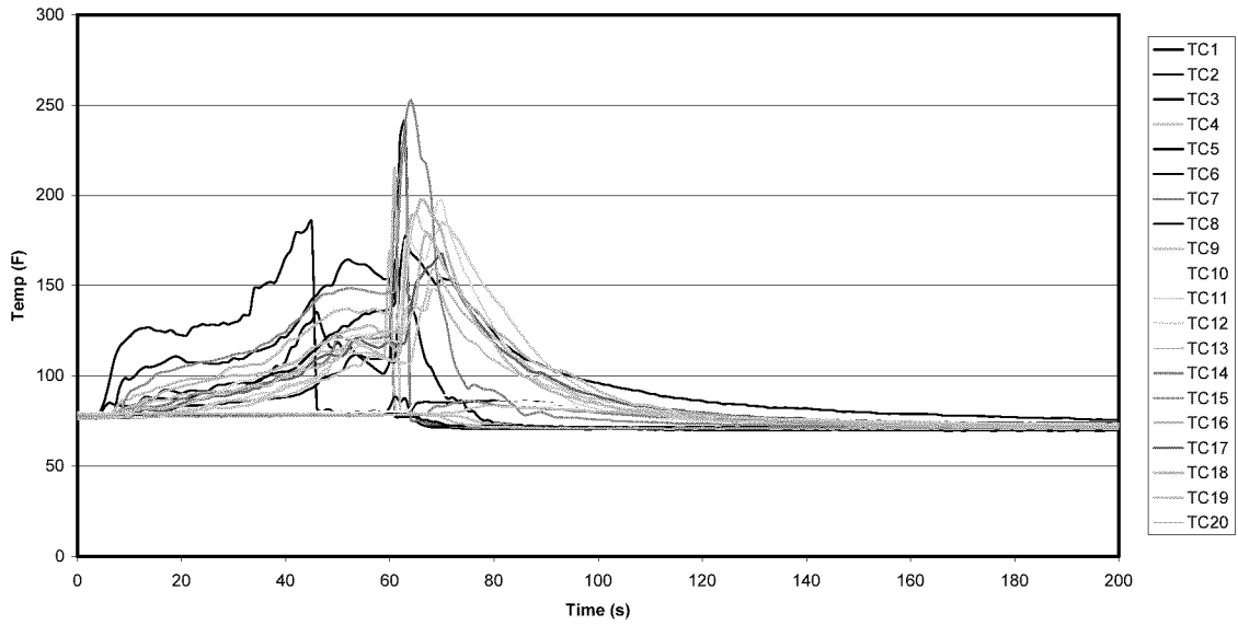
Figure A-23: Test 10 All Ceiling Temperatures
