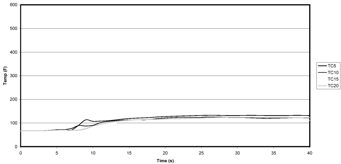
Figure A-35: Test 4 Row 5 Ceiling Temperatures
