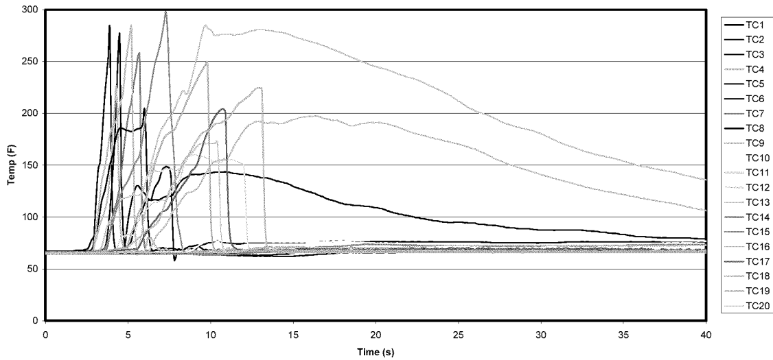
Ceiling Temperatures Spontaneous Combustion Scenario 29 March '01 - Test 6
