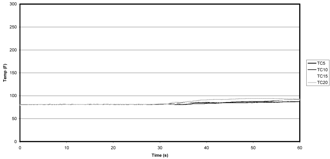
Row 5 Temperature IR Flare Scenario 12 April '01 - Test 7
