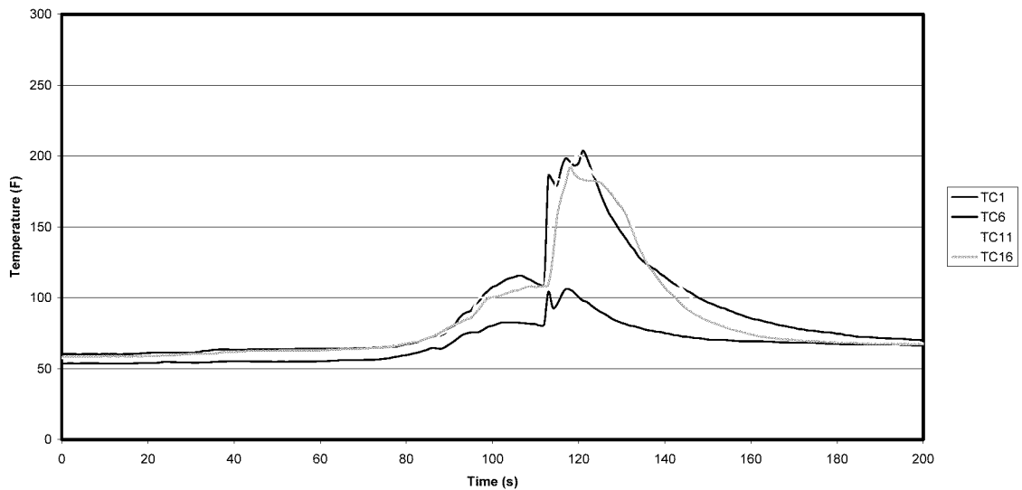
Row 1 Temperature Modified Fuel Spill Scenario 6 February '01 - Test 2
