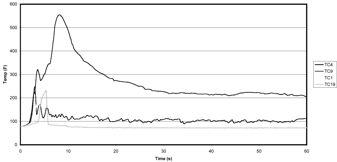
Row 4 Temperature Fire Origin at Base of Stack Scenario 3 May '01 - Test 11
