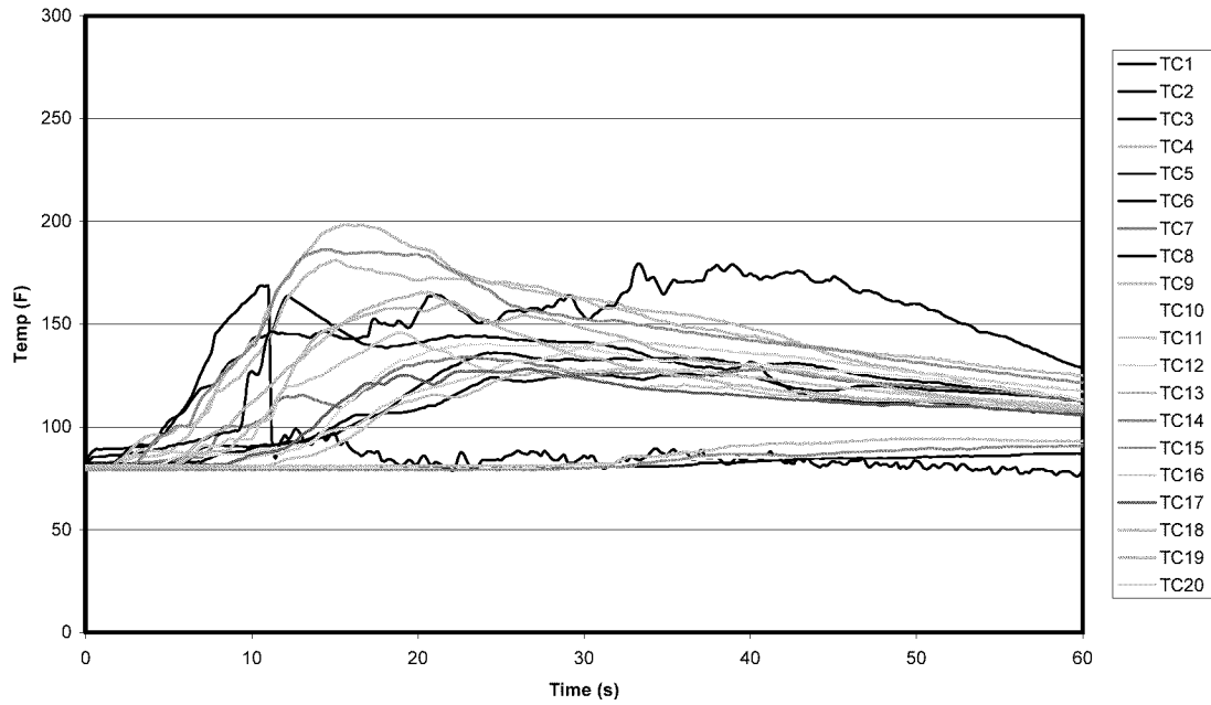
Ceiling Temperatures IR Flare Scenario 12 April '01 - Test 7
