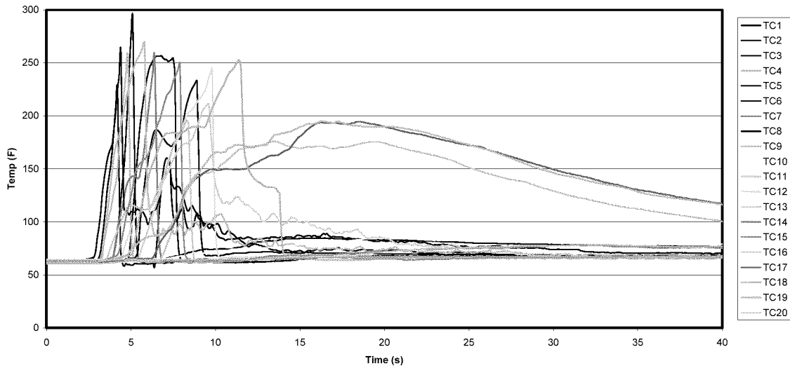
Figure A-37: Test 5 All Ceiling Temperatures
