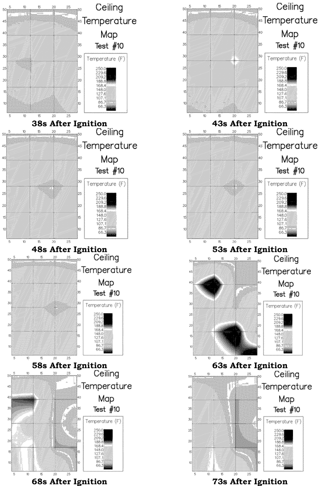
Figure A-29: Test 10 Ceiling Temperatures @ 5 Second Intervals
