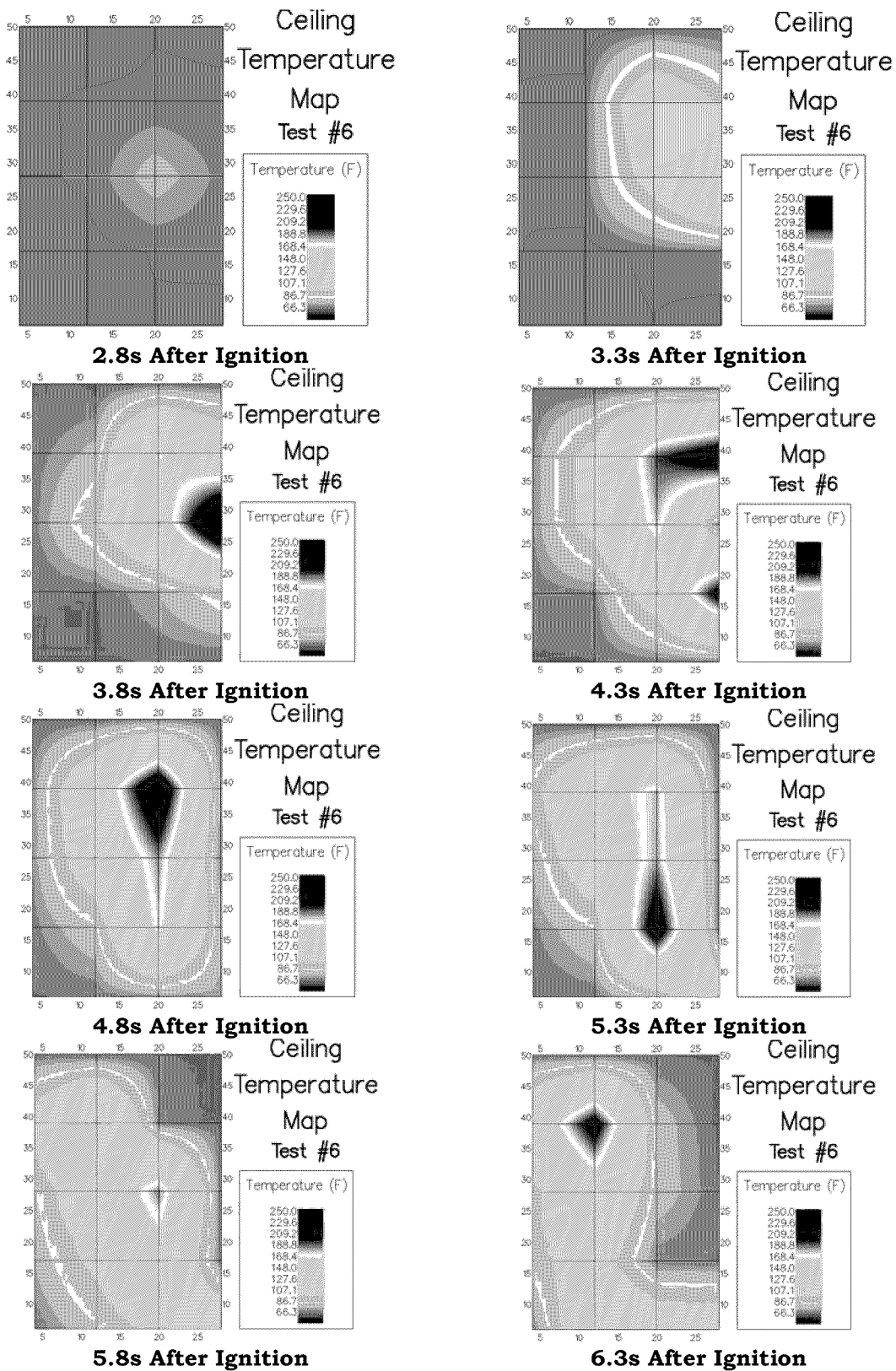
Figure 24: Test 6 Ceiling Temperatures @ 0.5 Second Intervals
