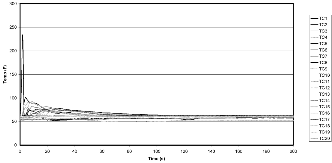
Figure A-2: Test 1 All Ceiling Temperatures
