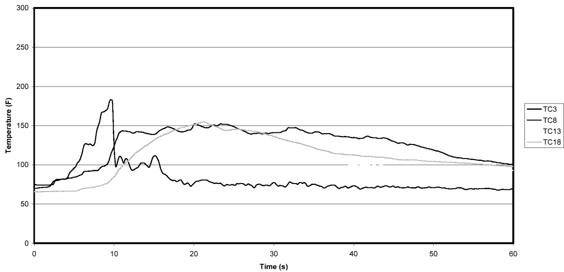
Figure A-61: Test 8 Row 3 Ceiling Temperatures
