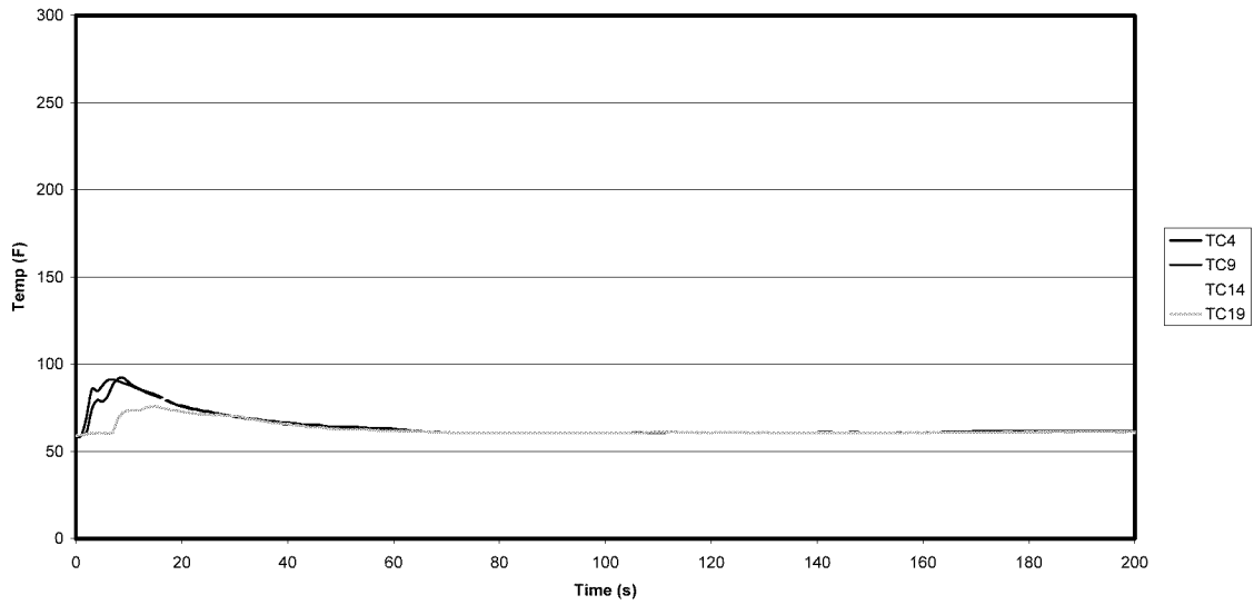
Figure A-6: Test 1 Row 4 Ceiling Temperatures
