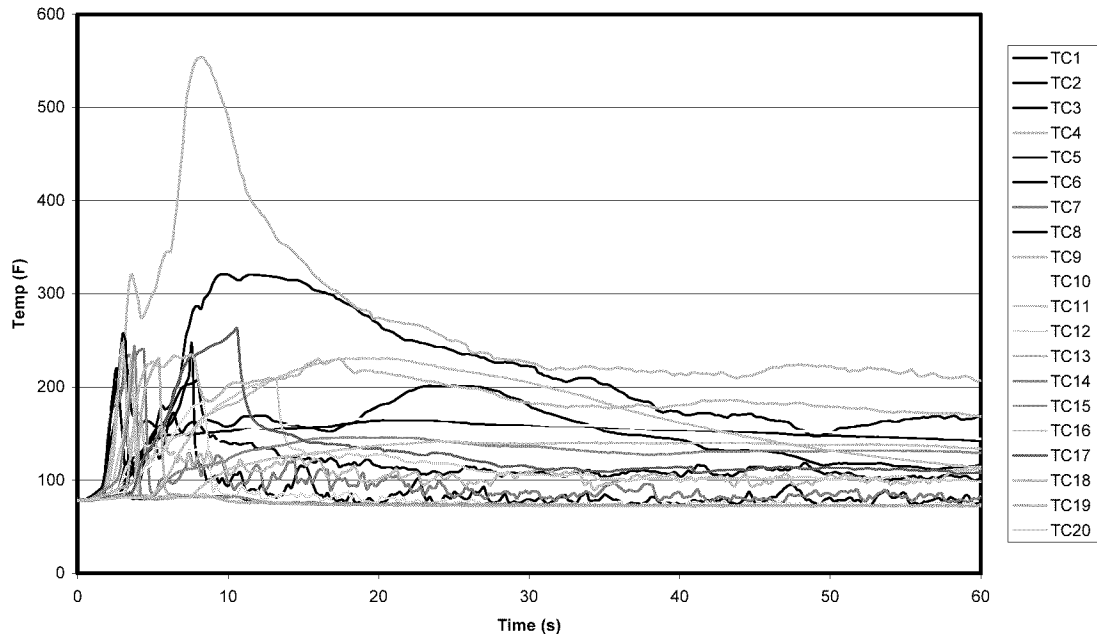
Figure A-72: Test 11 All Ceiling Temperatures
