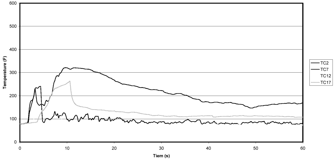
Row 2 Temperature Fire Origin at Base of Stack Scenario 3 May '01 - Test 11
