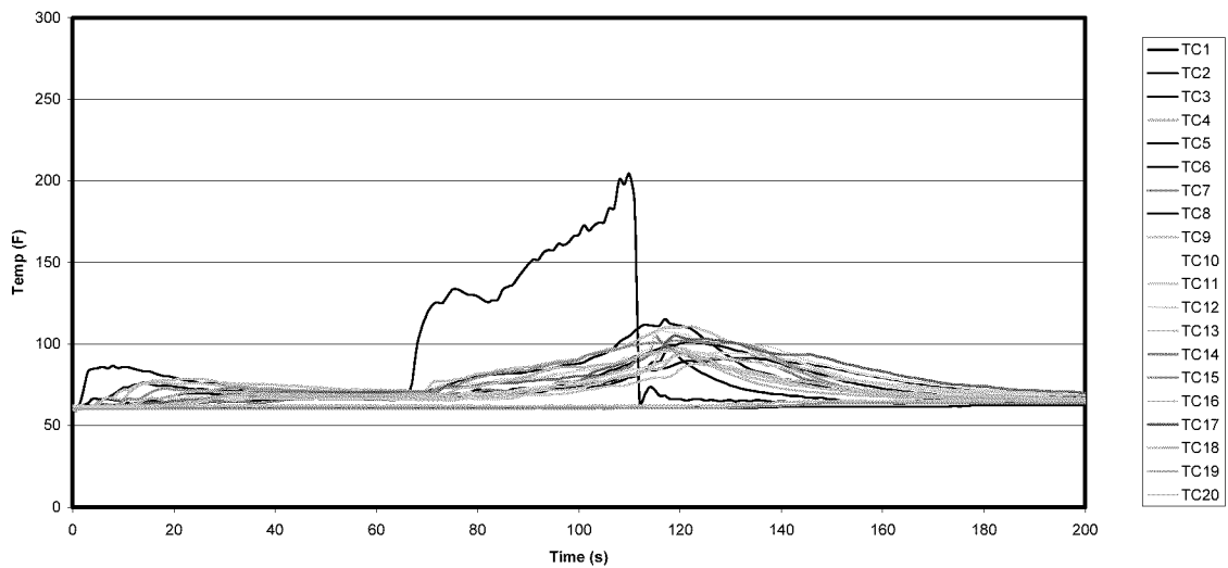
Figure A-9: Test 3 All Ceiling Temperatures
