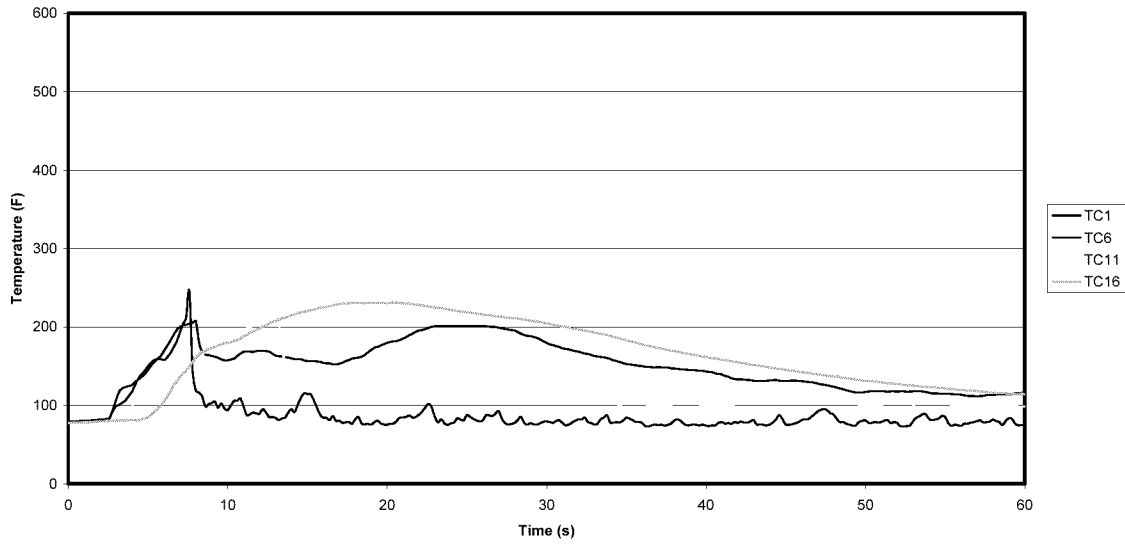
Figure A-73: Test 11 Row 1 Ceiling Temperatures
