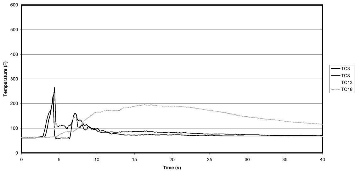
Figure A-40: Test 5 Row 3 Ceiling Temperatures
