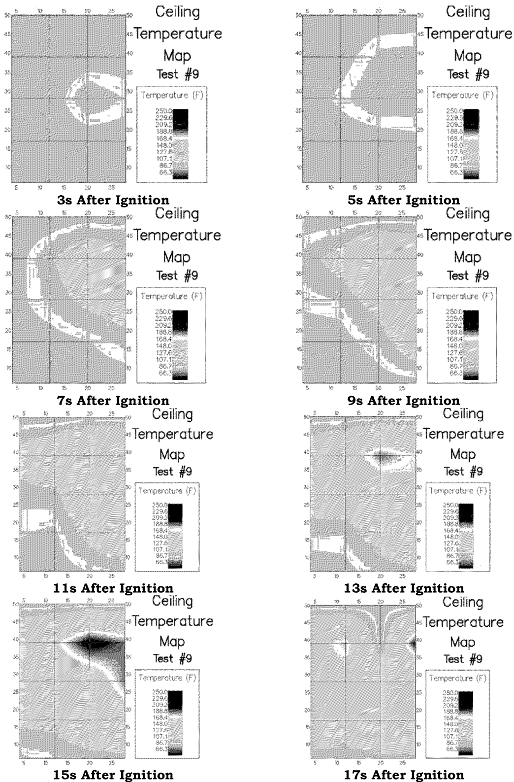
Figure A-71: Test 9 Ceiling Temperatures @ 2 Second Intervals
