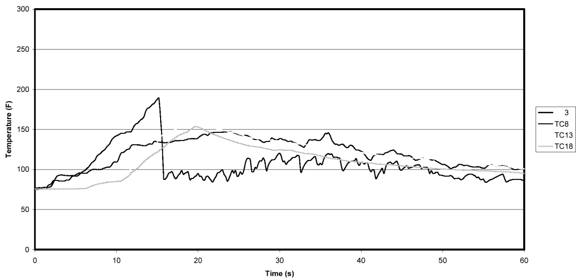
Row 3 Temperature IR Flare Scenario 30 April '01 - Test 9
