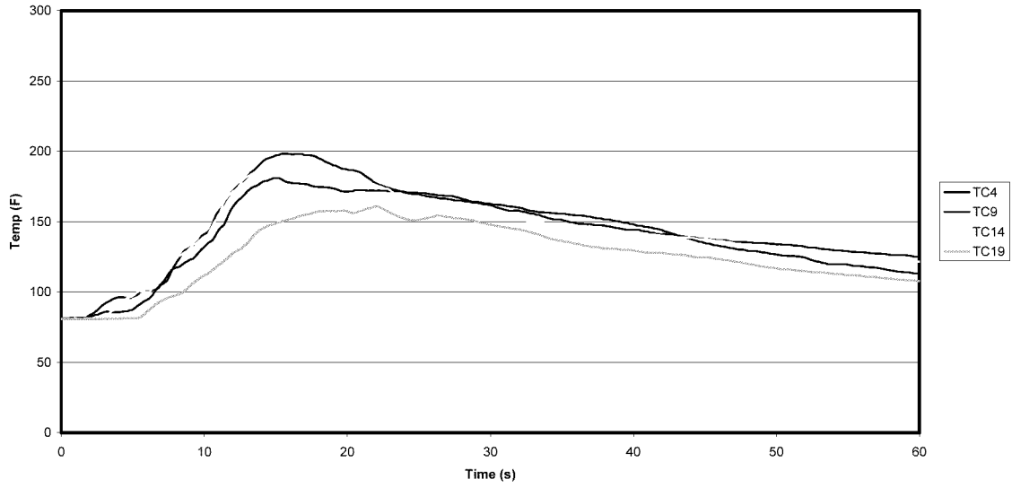
Row 4 Temperature IR Flare Scenario 12 April '01 - Test 7
