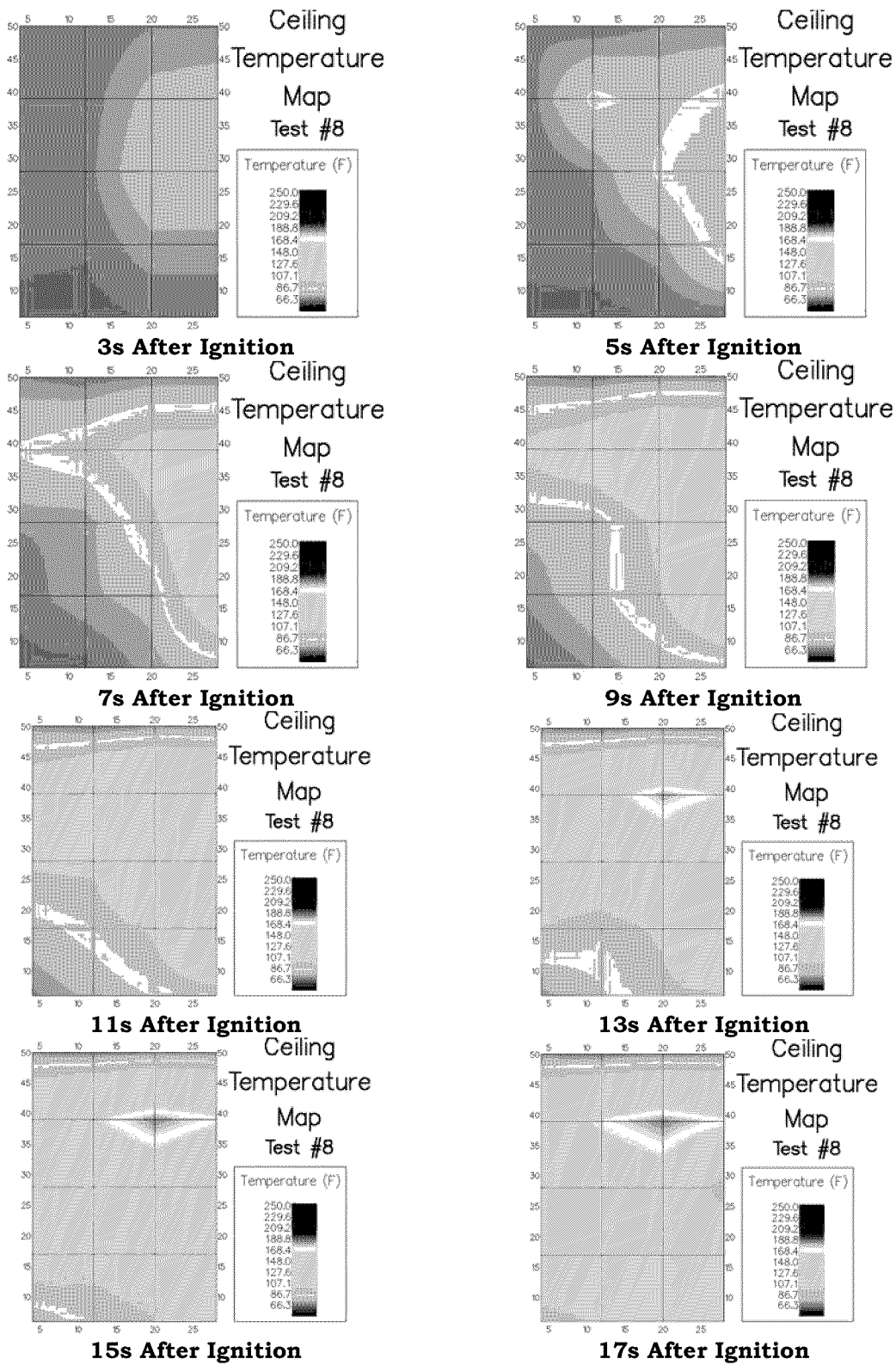
Figure A-64: Test 8 Ceiling Temperatures @ 2 Second Intervals
