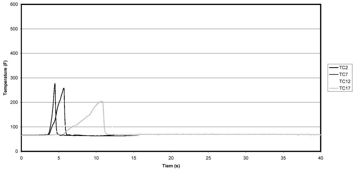
Figure A-46: Test 6 Row 2 Ceiling Temperatures
