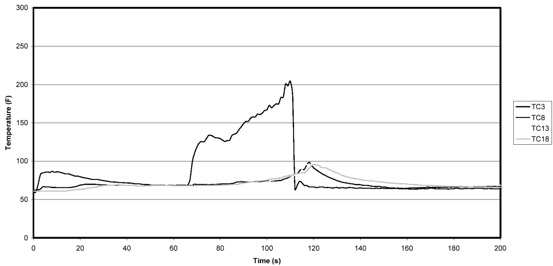
Row 3 Temperature Fuel Spill Scenario 19 March '01 - Test 3
