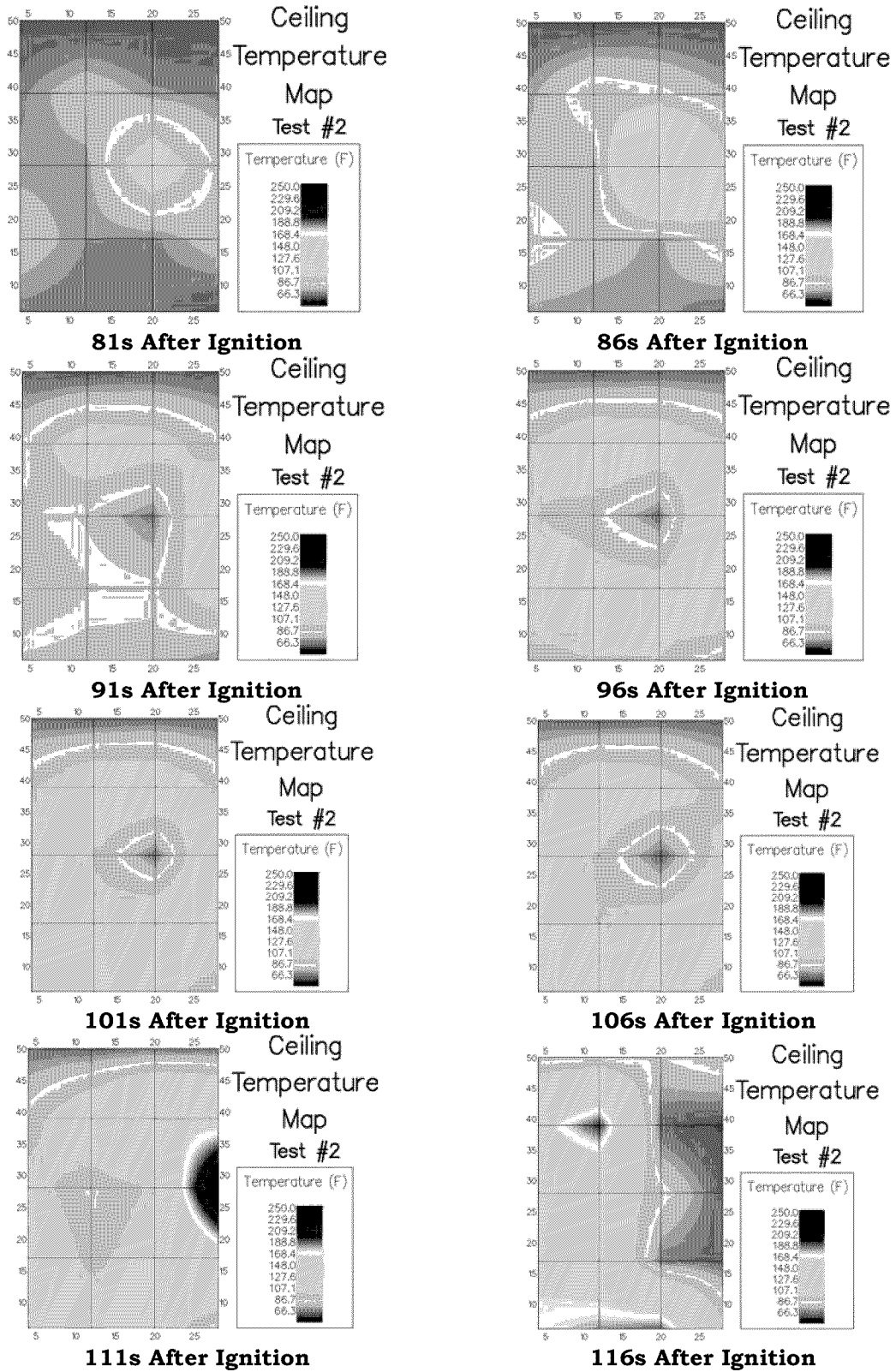
Figure A-22: Test 2 Ceiling Temperatures @ 5 Second Intervals
