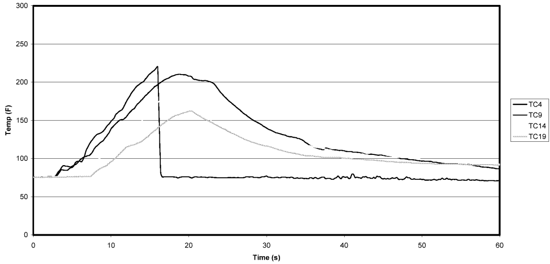
Figure A-69: Test 9 Row 4 Ceiling Temperatures
