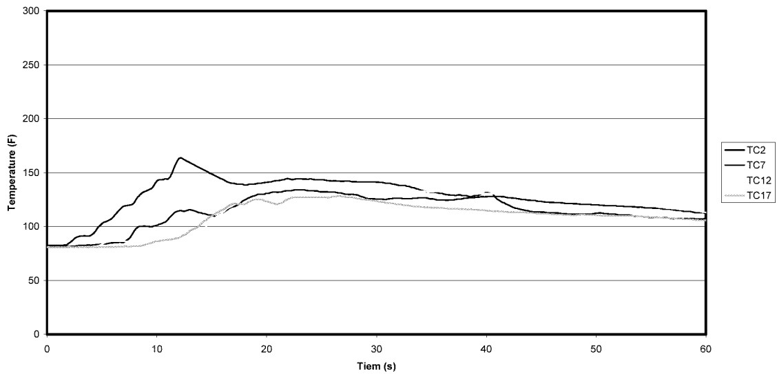
Row 2 Temperature IR Flare Scenario 12 April '01 - Test 7
