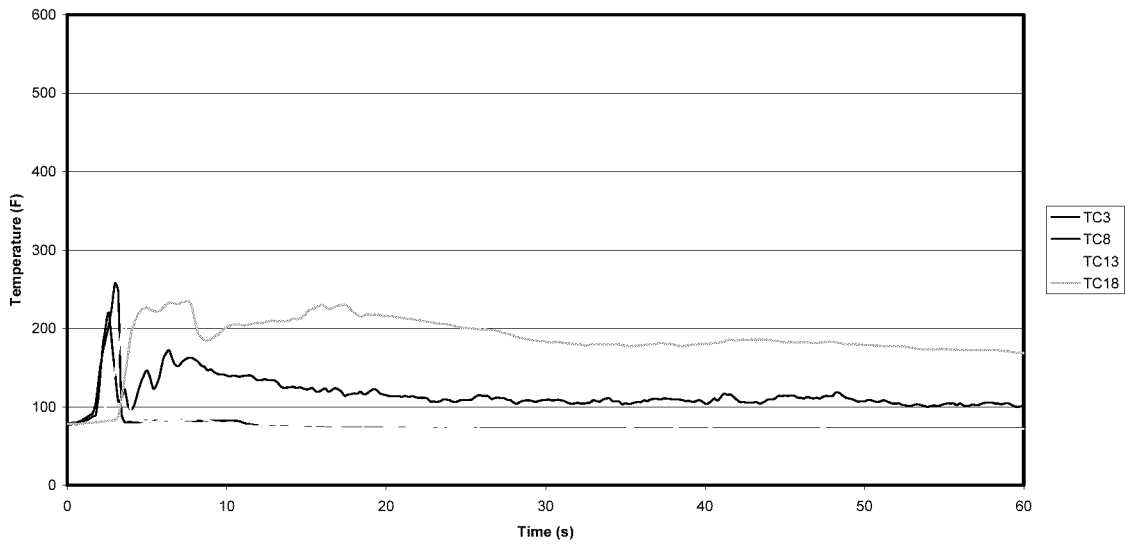
Row 3 Temperature Fire Origin at Base of Stack Scenario 3 May '01 - Test 11
