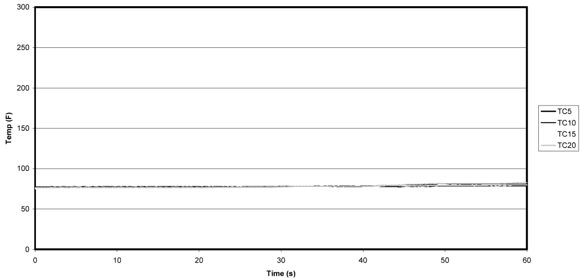
Figure A-70: Test 9 Row 5 Ceiling Temperatures
