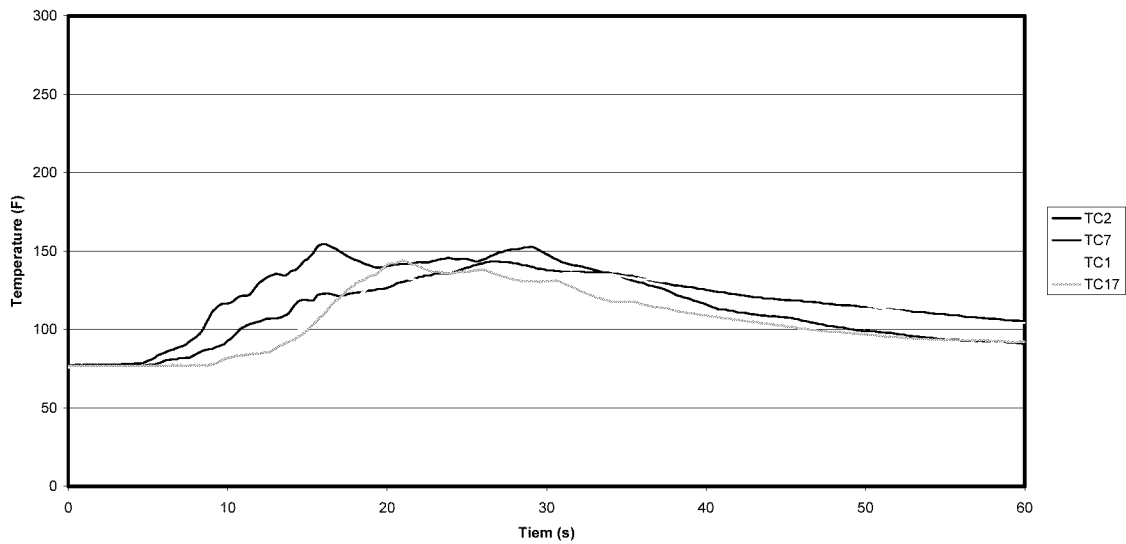
Row 2 Temperature IR Flare Scenario 30 April '01 - Test 9
