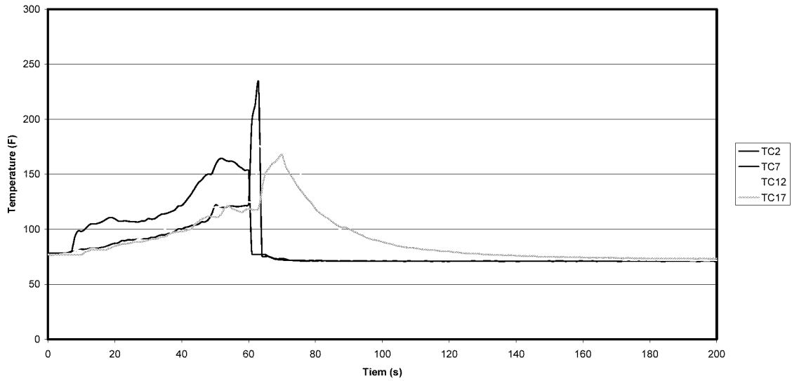
Figure A-25: Test 10 Row 2 Ceiling Temperatures
