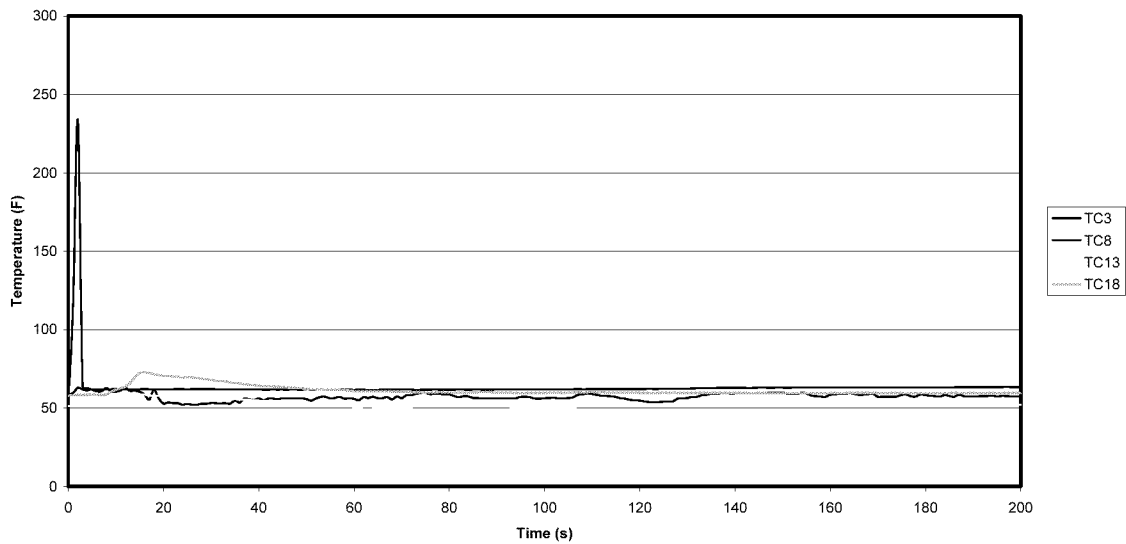
Figure A-5: Test 1 Row 3 Ceiling Temperatures
