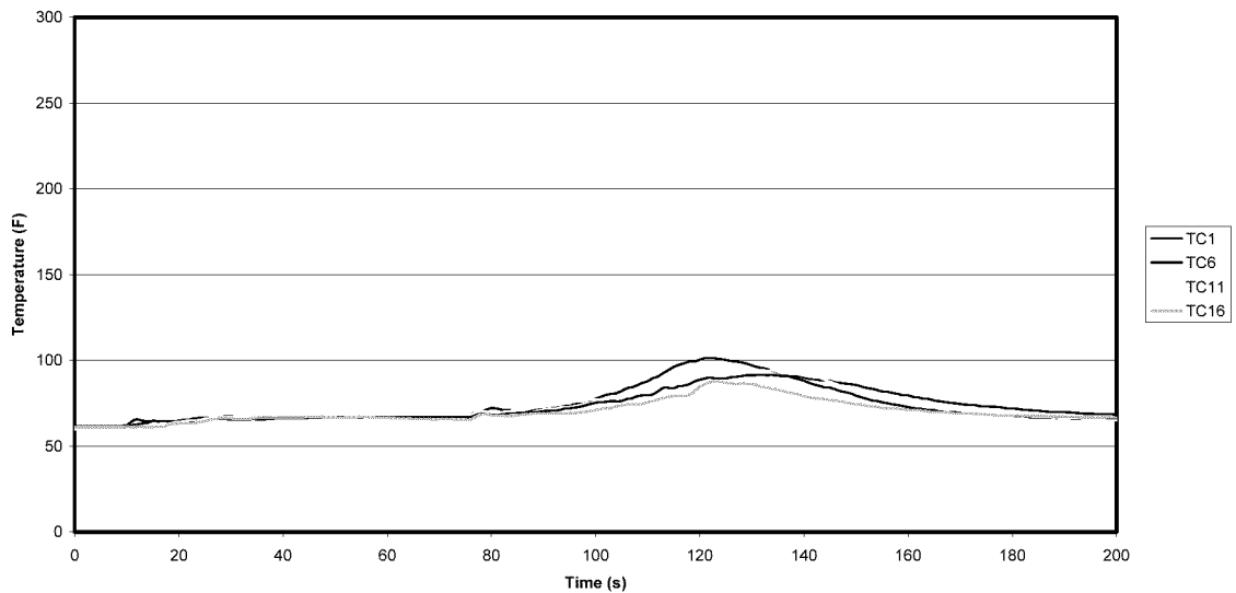
Figure A-10: Test 3 Row 1 Ceiling Temperatures
