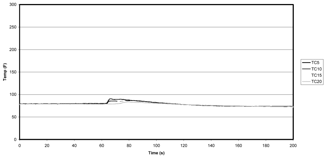
Figure A-28: Test 10 Row 5 Ceiling Temperatures
