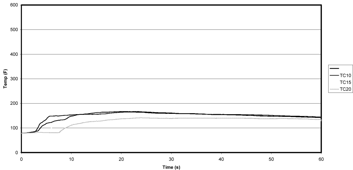
Row 5 Temperature Fire Origin at Base of Stack Scenario 3 May '01 - Test 11
