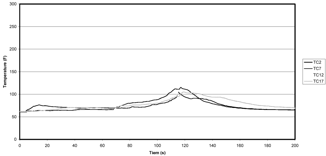
Row 2 Temperature Fuel Spill Scenario 19 March '01 - Test 3
