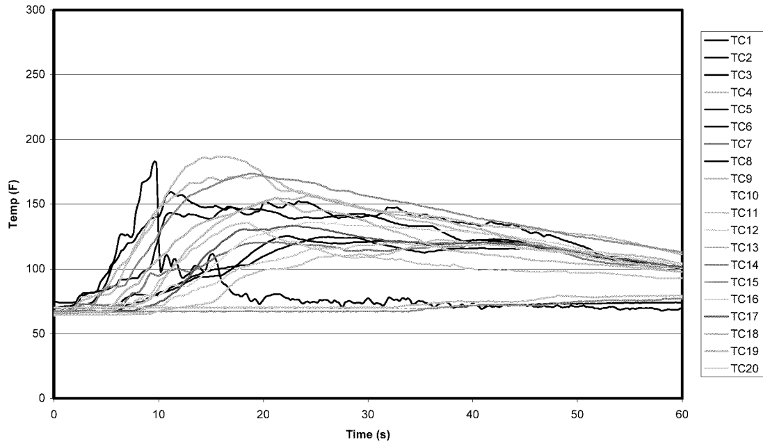
Ceiling Temperatures IR Flare Scenario 19 April '01 - Test 8
