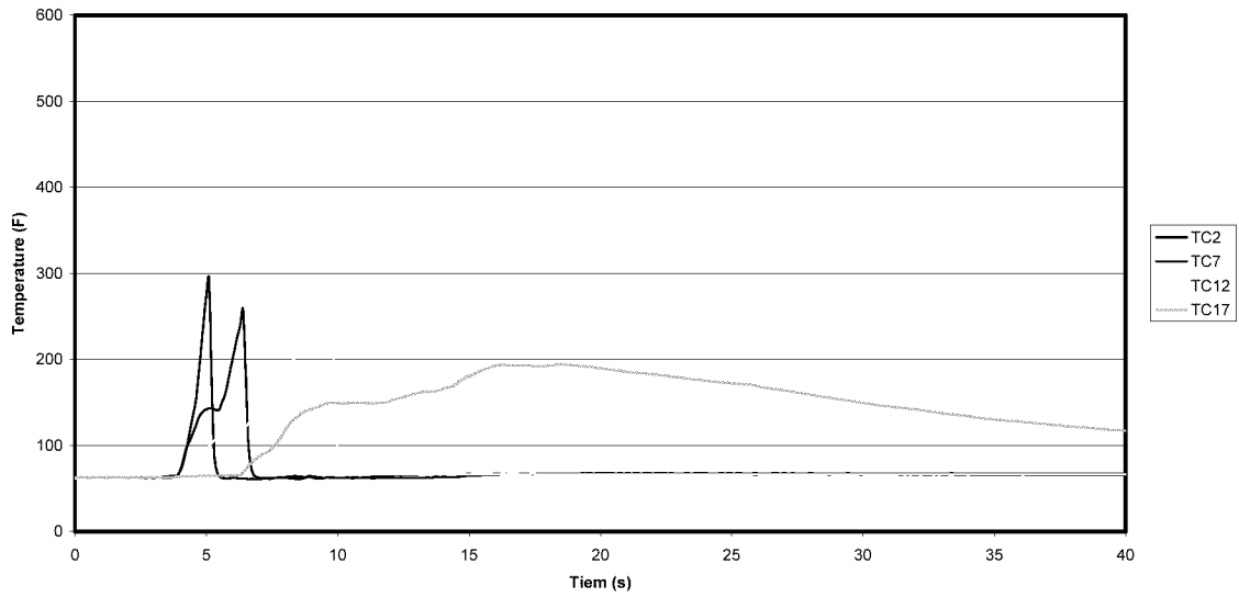
Figure A-39: Test 5 Row 2 Ceiling Temperatures
