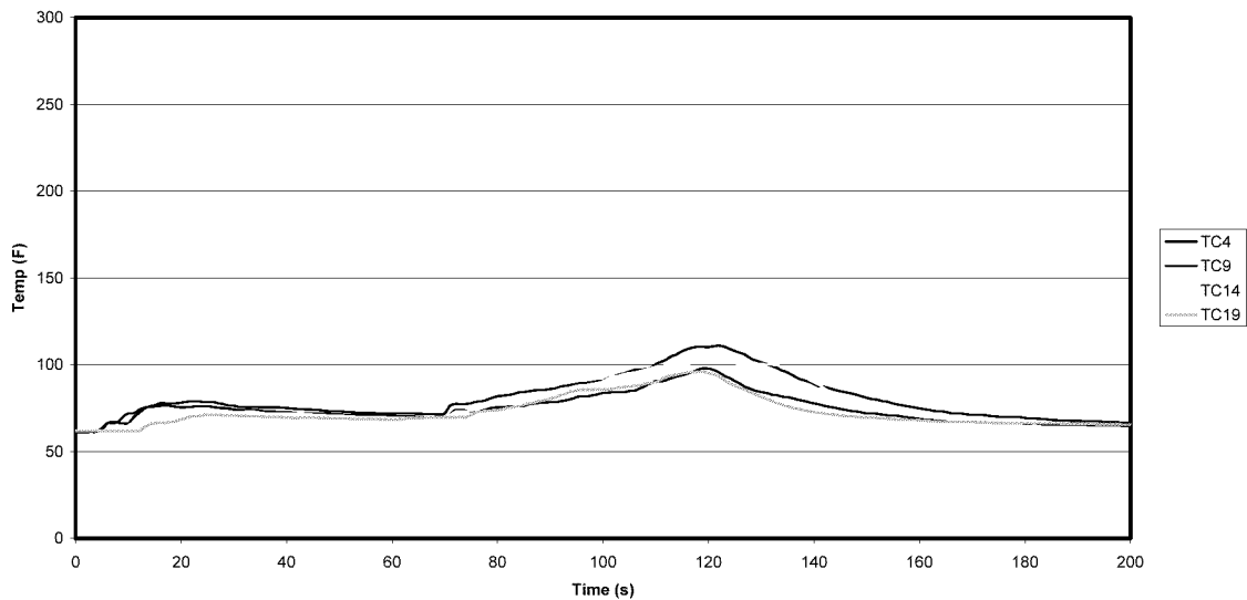
Figure A-13: Test 3 Row 4 Ceiling Temperatures
