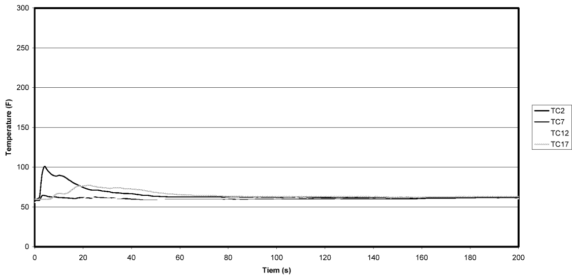
Figure A-4: Test 1 Row 2 Ceiling Temperatures
