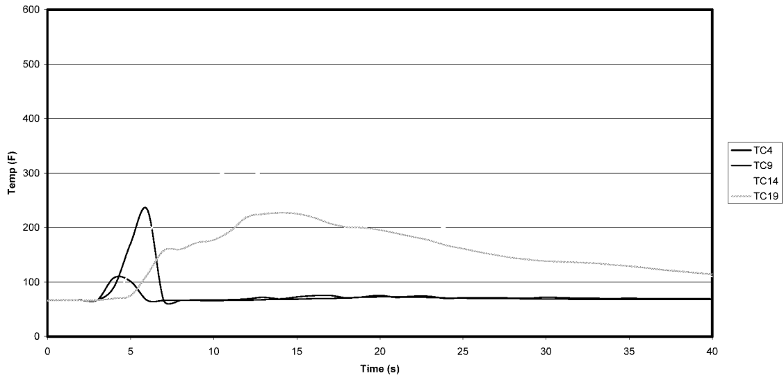
Figure A-34: Test 4 Row 4 Ceiling Temperatures
