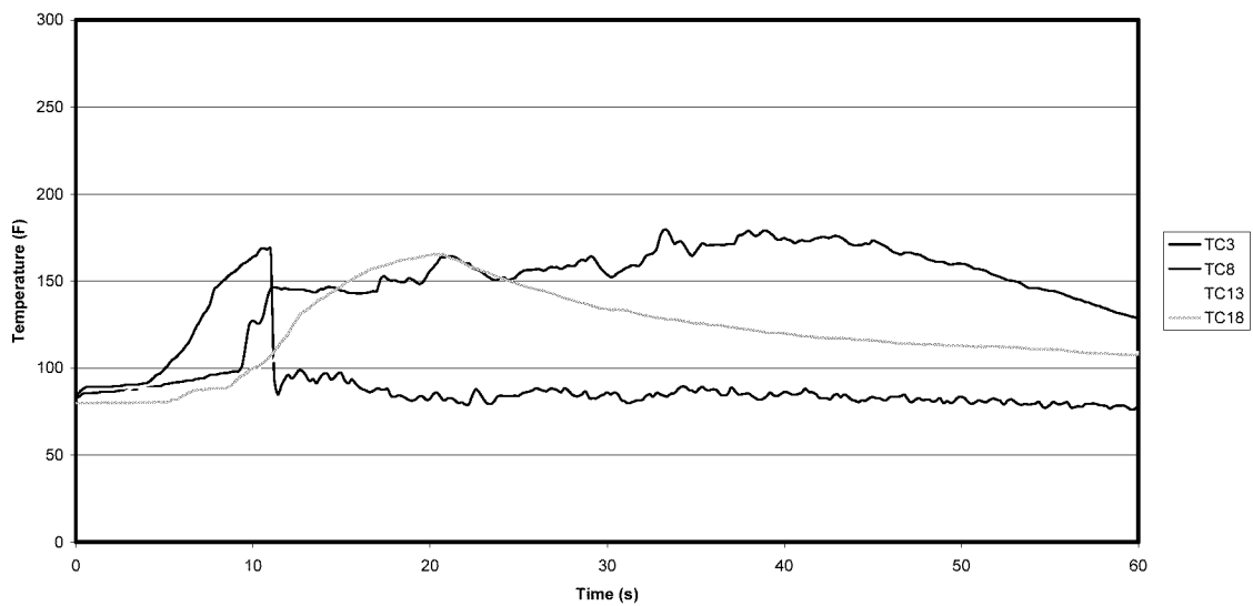
Row 3 Temperature IR Flare Scenario 12 April '01 - Test 7
