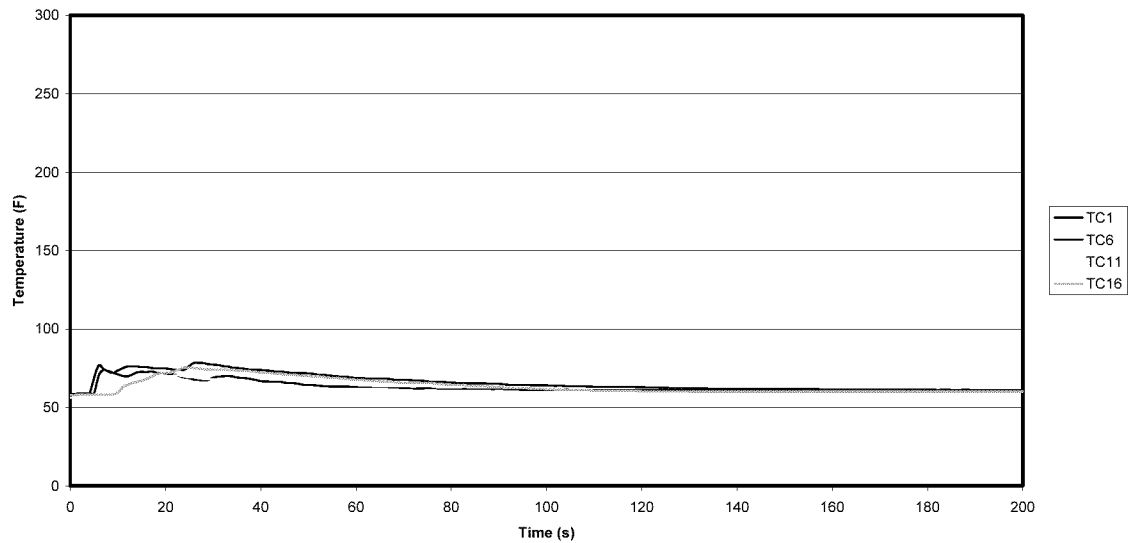
Figure A-3: Test 1 Row 1 Ceiling Temperatures
