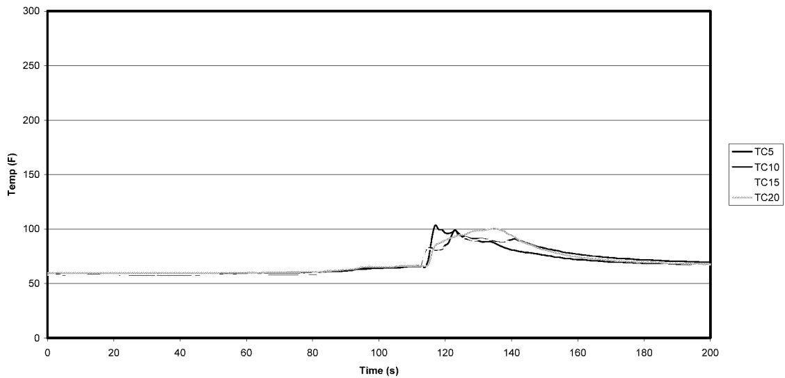
Row 5 Temperature Modified Fuel Spill Scenario 6 February '01 - Test 2
