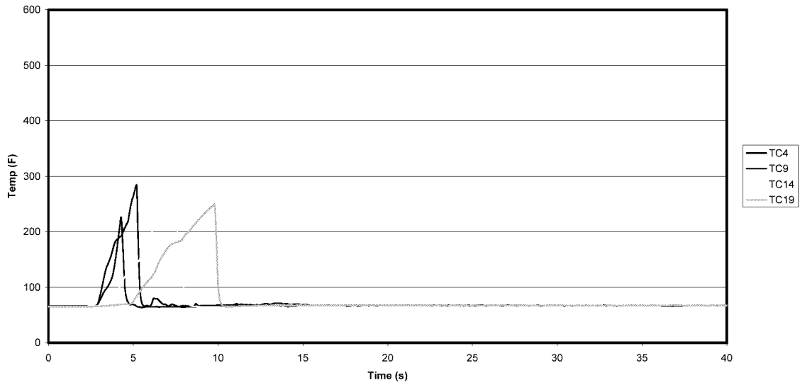
Figure A-48: Test 6 Row 4 Ceiling Temperatures
