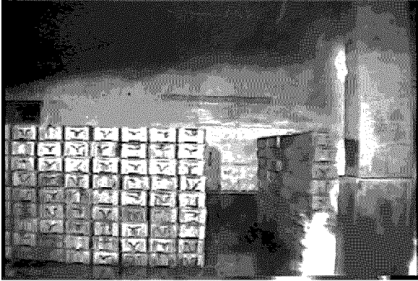
Figure 14: Test 2 Fire, 9 Seconds Before Sprinkler Activation
