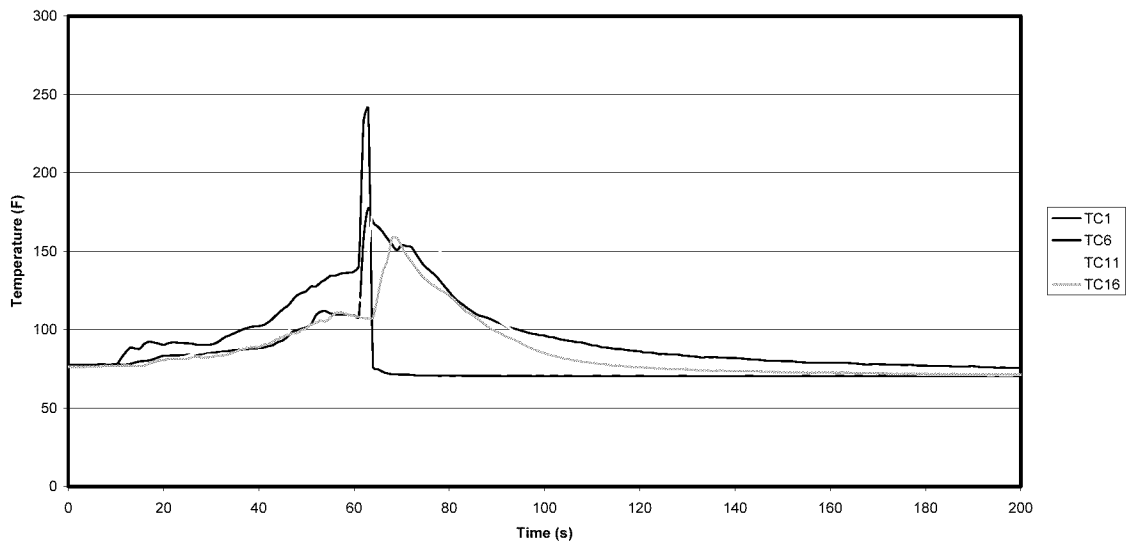
Figure A-24: Test 10 Row 1 Ceiling Temperatures
