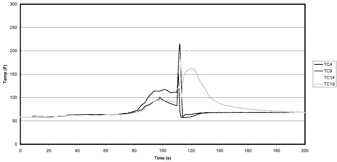
Row 4 Temperature Modified Fuel Spill Scenario 6 February '01 - Test 2
