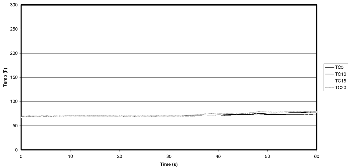
Figure A-63: Test 8 Row 5 Ceiling Temperatures
