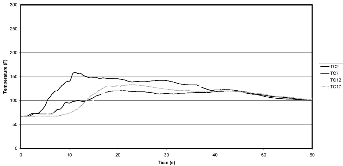
Figure A-60: Test 8 Row 2 Ceiling Temperatures
