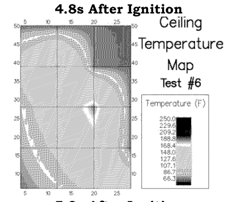
Figure A-50: Test 6 Ceiling Temperatures @ 0.5 Second Intervals
