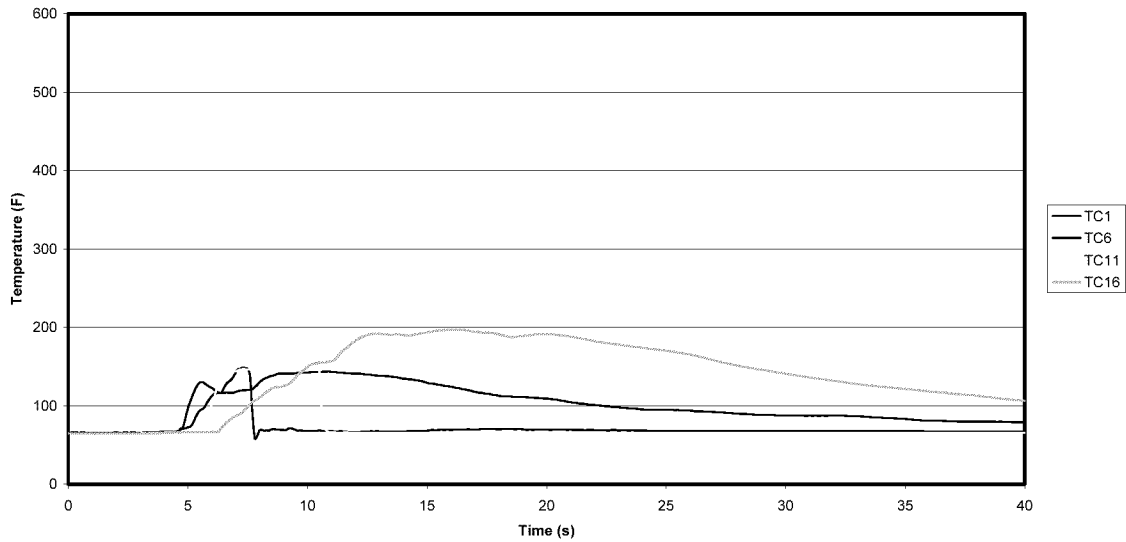
Row 1 Temperature Spontaneous Combustion Scenario 29 March '01 - Test 6
