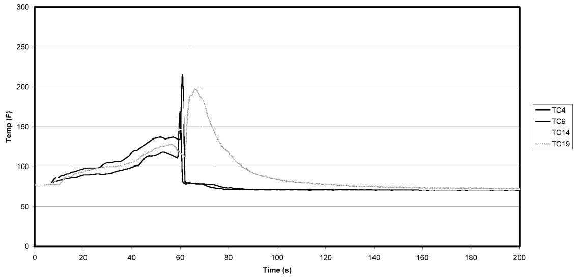
Figure A-27: Test 10 Row 4 Ceiling Temperatures
