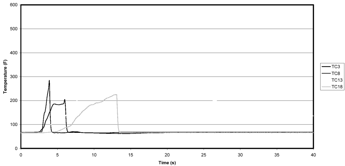
Figure A-47: Test 6 Row 3 Ceiling Temperatures
