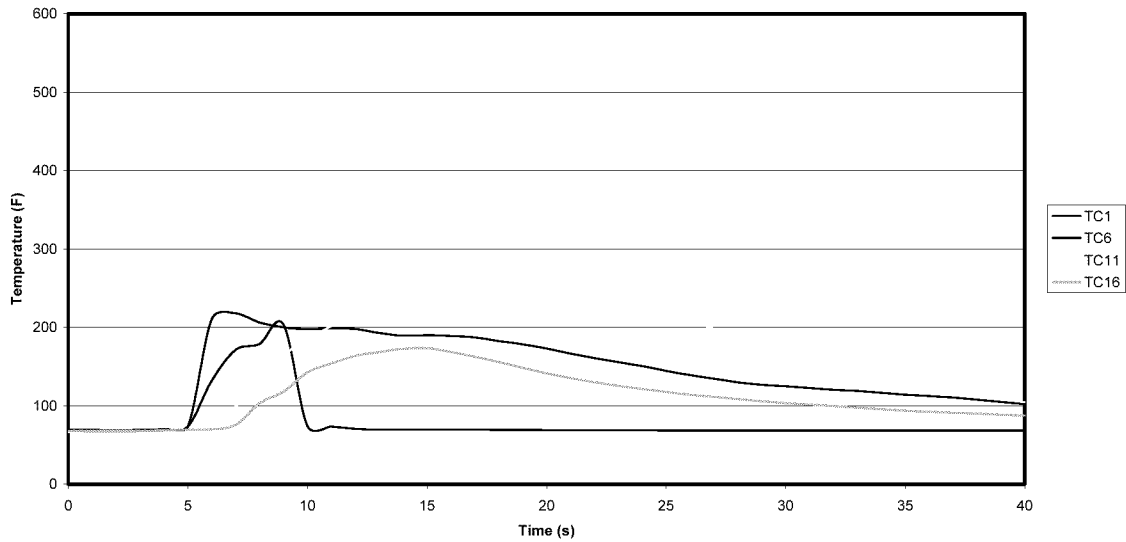
Row 1 Temperature Spontaneous Combustion Scenario 9 February '01 - Test 4
