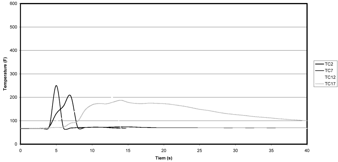
Figure A-32: Test 4 Row 2 Ceiling Temperatures
