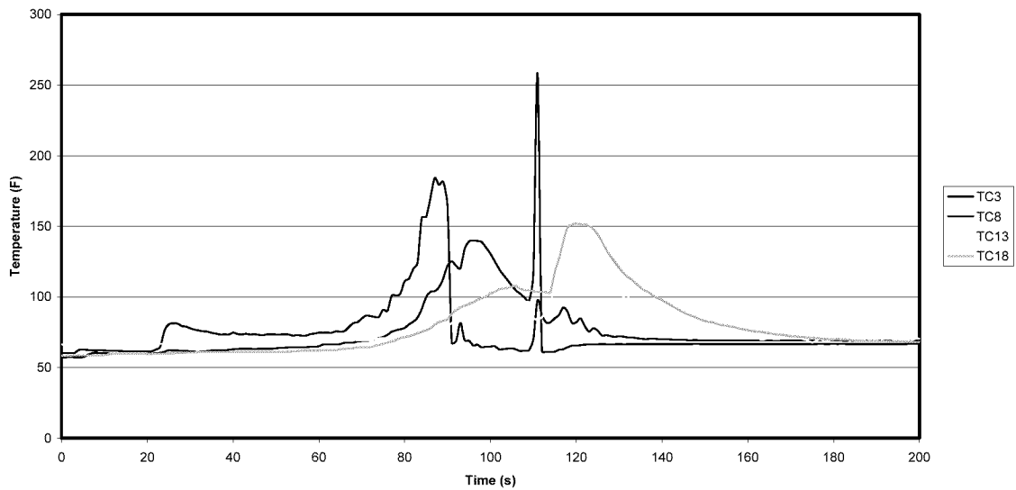
Row 3 Temperature Modified Fuel Spill Scenario 6 February '01 - Test 2
