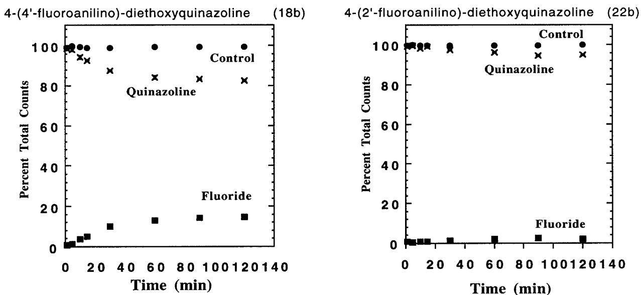
Figure 13. Hepatocyte metabolism kinetic profile of para- ( 18b ) versus ortho- ( 22b ) [ ^{18}\text{F} ]fluoroanilindiethoxyquinazoline analogs. Control contained no hepatocytes.
