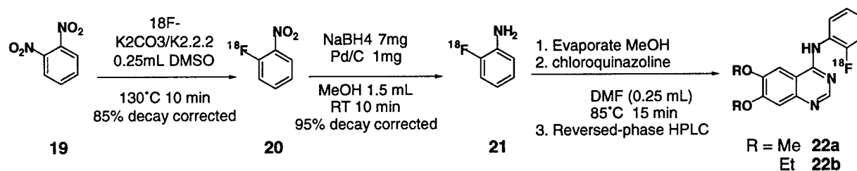
Figure 8. Synthesis of 4-(2'-[ ^{18}\text{F} ]fluoroanilino)-6,7-dimethoxy- and 4-(2'-[ ^{18}\text{F} ]fluoroanilino)-6,7-diethoxy- quinazoline
