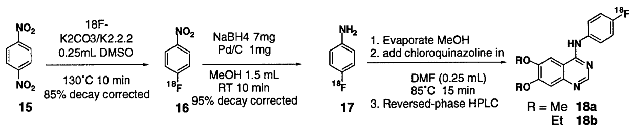
Figure 7. Synthesis of 4-(4'-[ ^{18}\text{F} ]fluoroanilino)-6,7-dimethoxy- and 4-(4'-[ ^{18}\text{F} ]fluoroanilino)-6,7-diethoxy- quinazoline.
