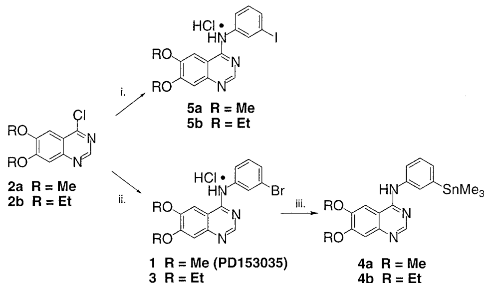
Figure 2. Synthetic routes for the iodoanilino- and trimethylstannylanilino-dialkoxiquinazolines. (i.) 3-iodoaniline, DMF, \Delta ; (ii.) 3-bromoaniline, DMF, \Delta ; (iii.) (\text{SnMe}_3)_2 , \text{Pd}(\text{Ph}_3)_4 , dioxane.
