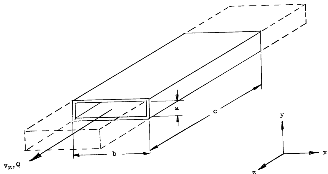
Figure 2. Flat Duct.
