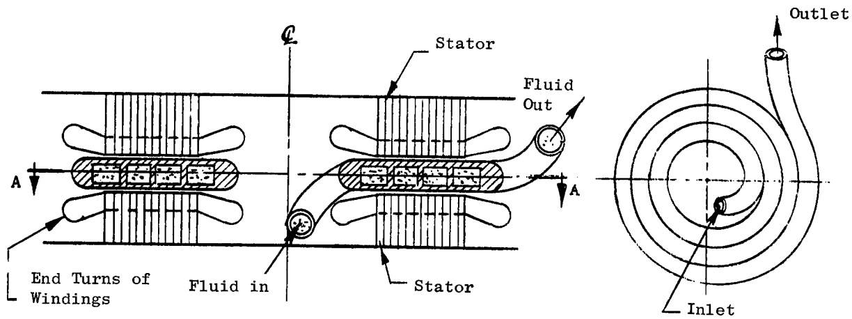
Figure 23. Spiral Induction Pump.
