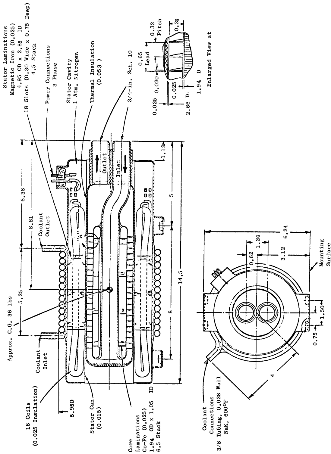
Figure 76. Helical Induction Pump: Center Return.
