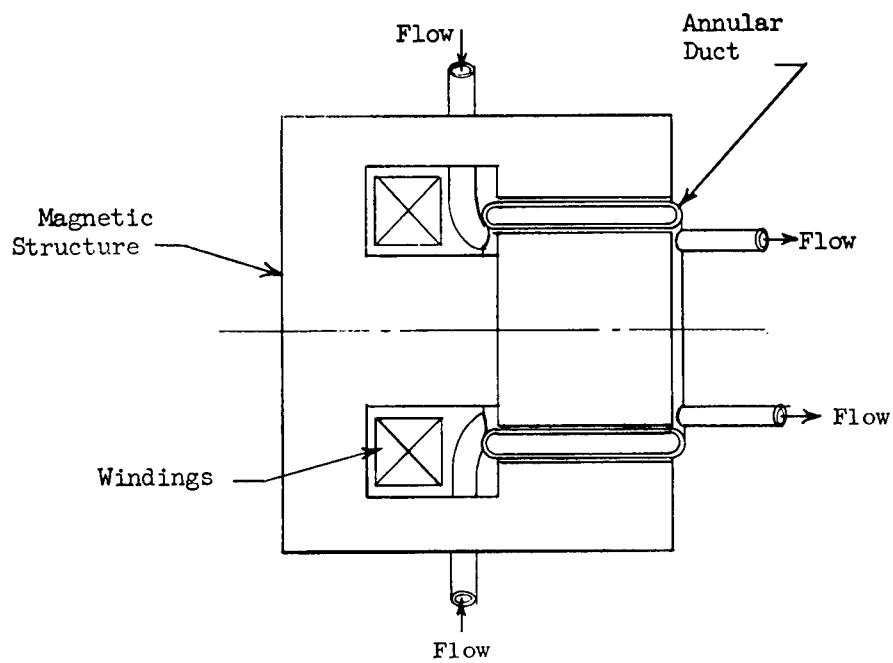
Figure 42. Single Phase Induction Pump Type B.
