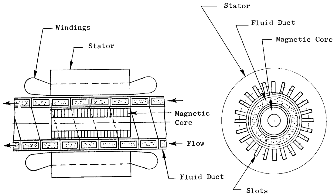
Figure 21. Helical Induction Pump.
