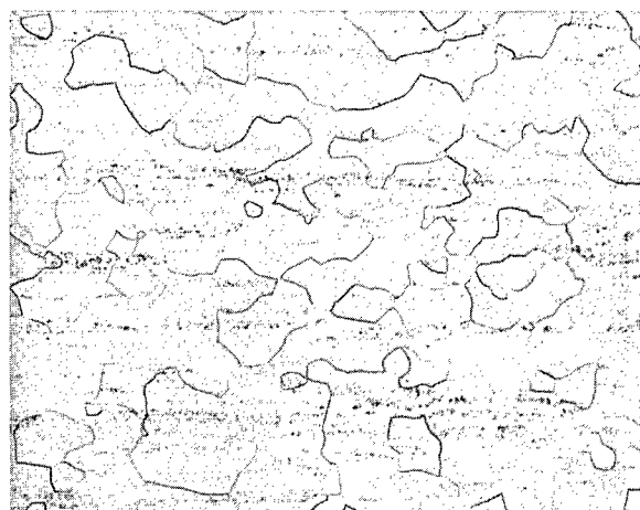
Figure 35. Longitudinal Microstructure of V-20w/oTi Cold-worked 25% and Vacuum-annealed for 1 hr at Various Temperatures (Etchant: 5% HF, 2% AgNO 3 )
