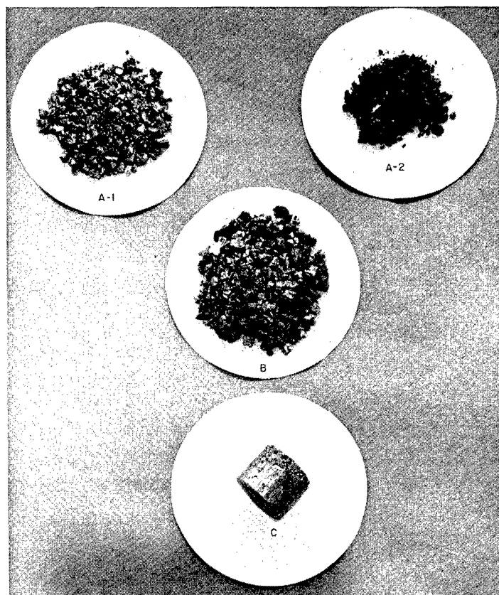
Figure 6 Vanadium Chips (A-1) and Titanium Sponge (A-2) after Blending (B) and Pressing into Briquet Form (C)
