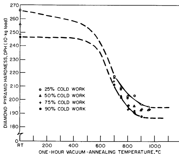
Figure 34 Diamond-pyramid-hardness Data on Heat-treated V-20w/oTi Having Var- ious Amounts of Cold Work
