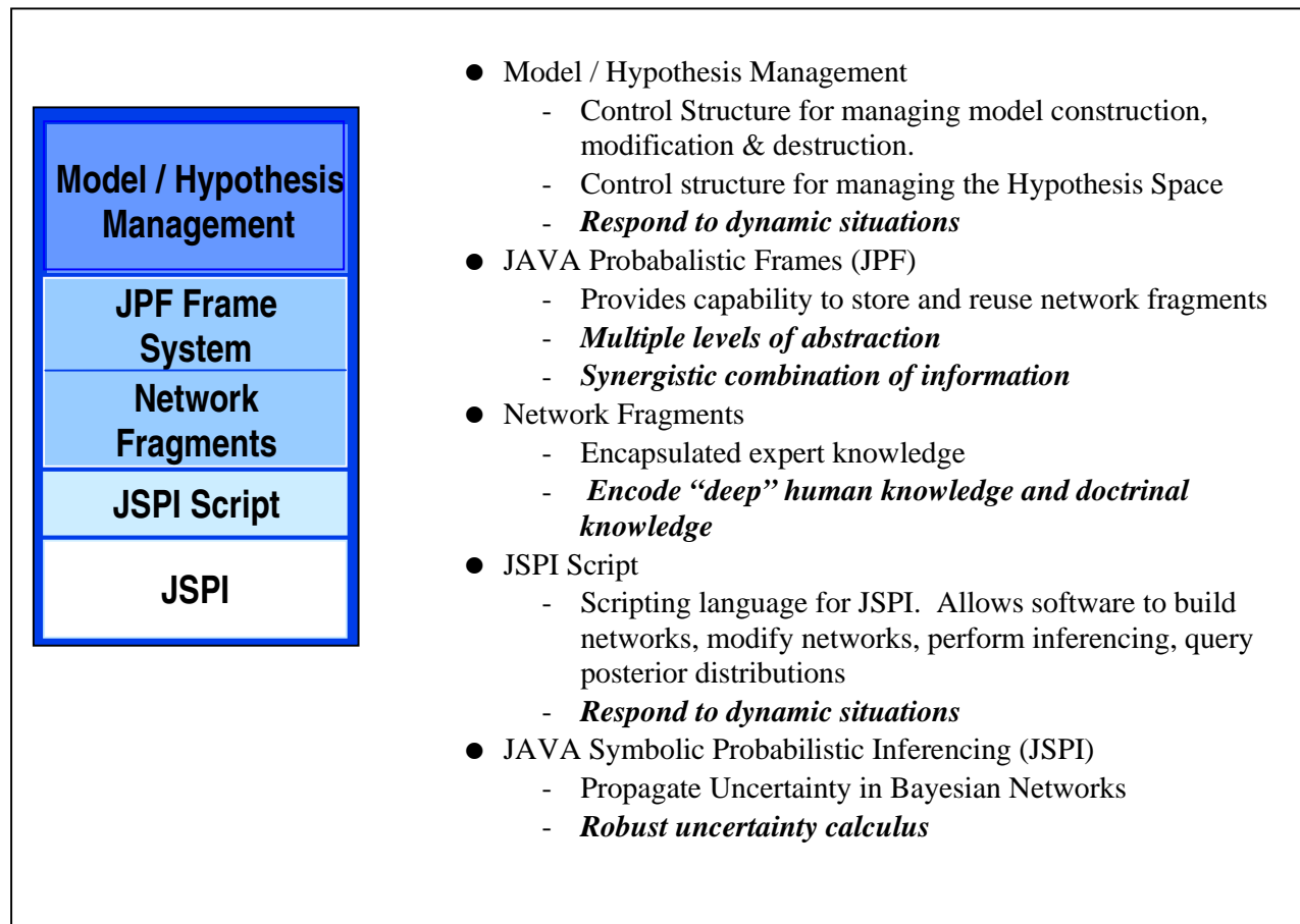
Figure 1. TSGUDA Architecture
