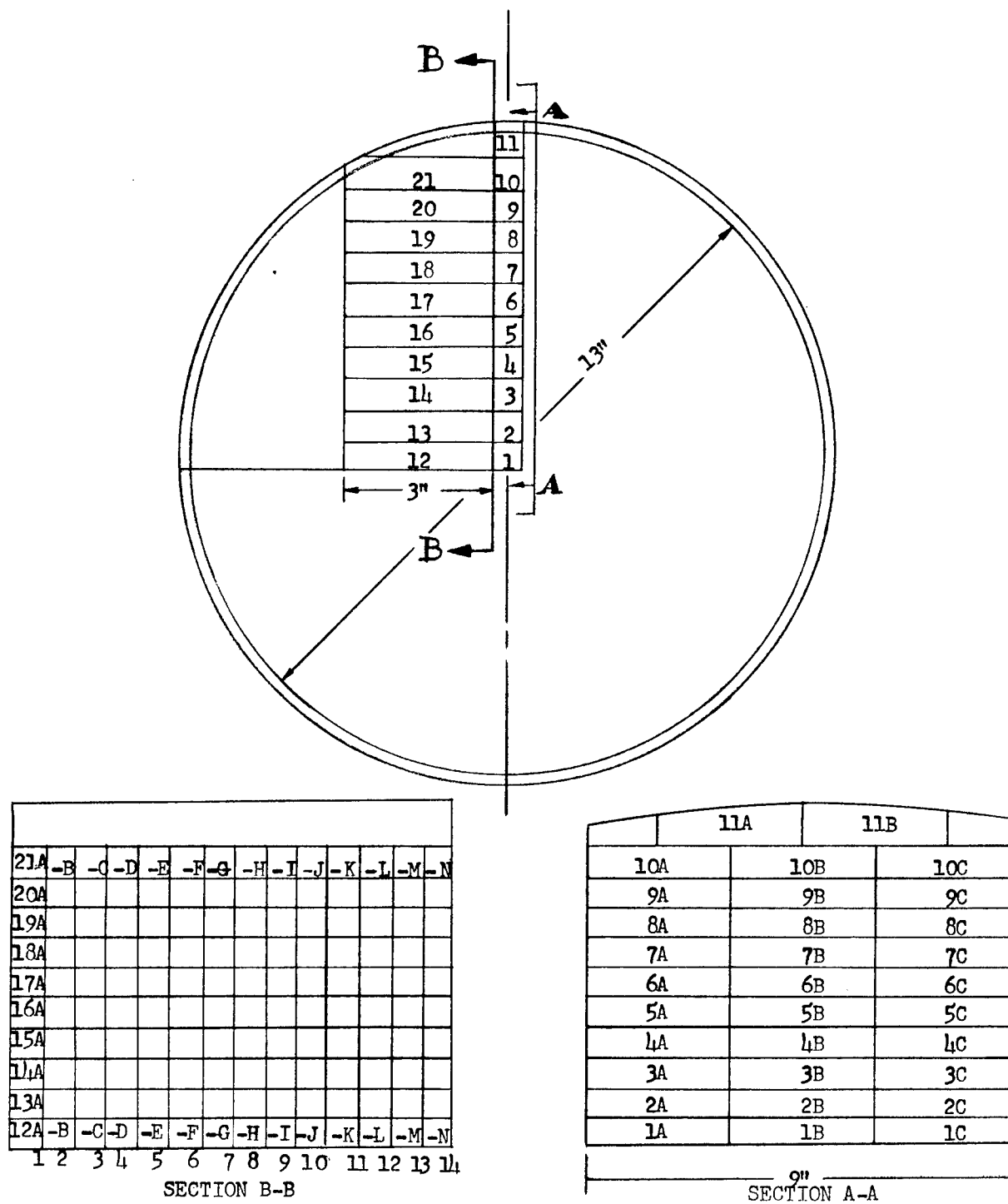
Figure 1 Specimen Locations of Standard 7075-T6 and Special Product 7079-T6 Hand Forgings
