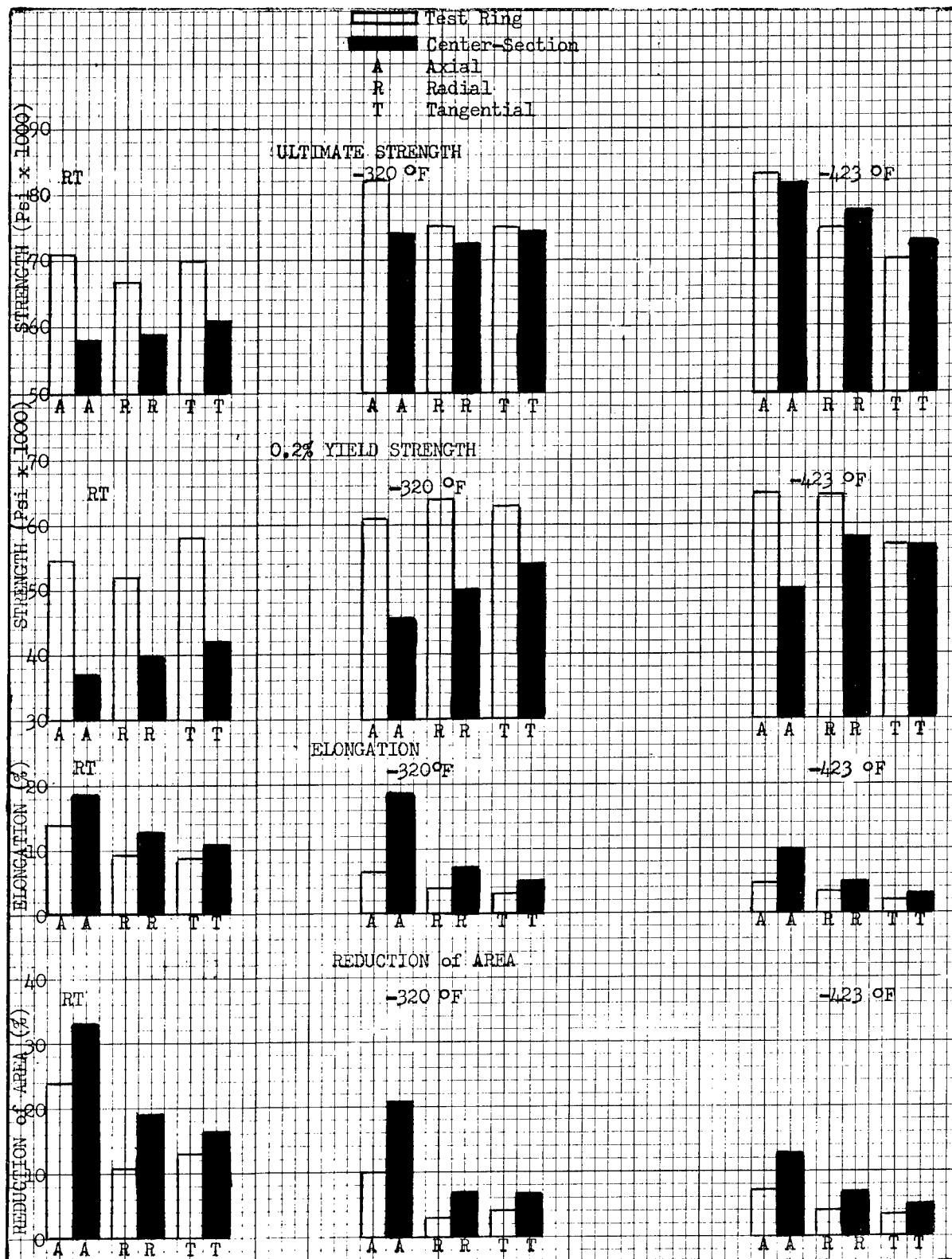
Figure 19 Comparison of Forging "A" Test Ring and Center Section Mechanical Properties
