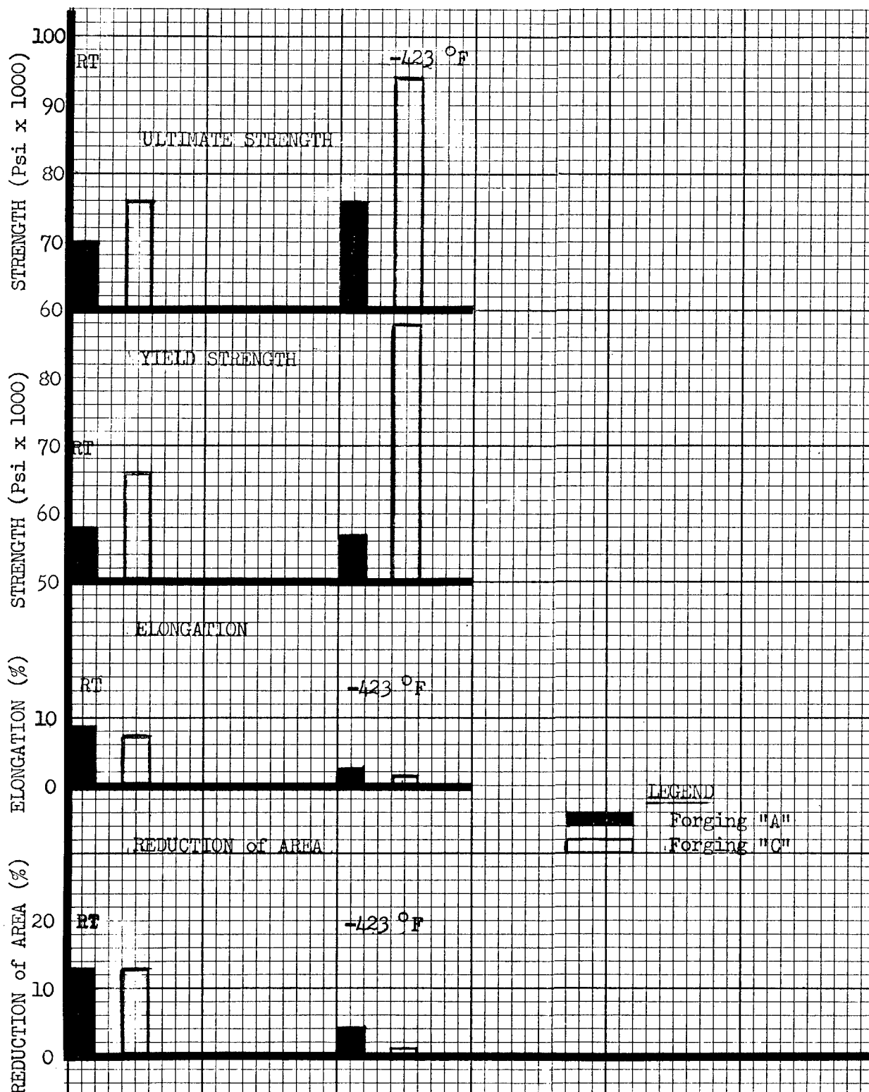
Figure 26 Comparative Forging "C" Test Ring Mechanical Properties
