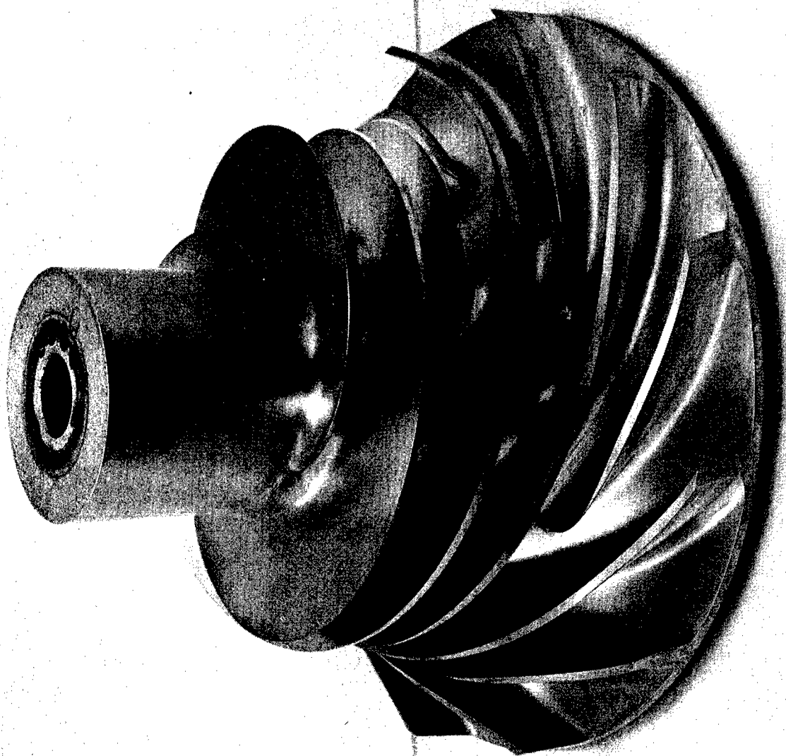
Figure 36 Machined Fuel Pump Inducer Blank
