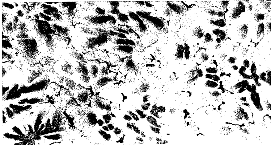
Figure 30 Microstructure of Forging C (One-Half Radius Location) Magnification: 100S Etchant: Flick's
