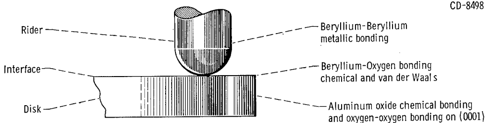
Figure 10. - Nature of surface interaction and bonding of beryllium to sapphire (0001) plane.
