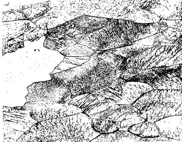
(b) Annealed for 1 hour at 2300° F; 73 percent recrystallized.
