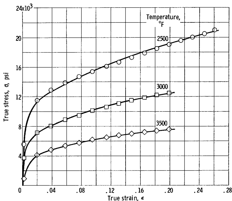
Figure 8. - Effect of temperature on tensile flow curves of electron-beam-melted tungsten at 2500^\circ to 3500^\circ\text{F} (lot EB-43, annealed for 1 hr at 3600^\circ\text{F} ).
