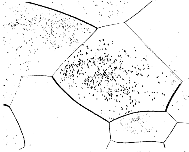
(d) Annealed for 1 hour at 2800° F; fully recrystallized; average grain diameter, 0.0321 centimeter.
