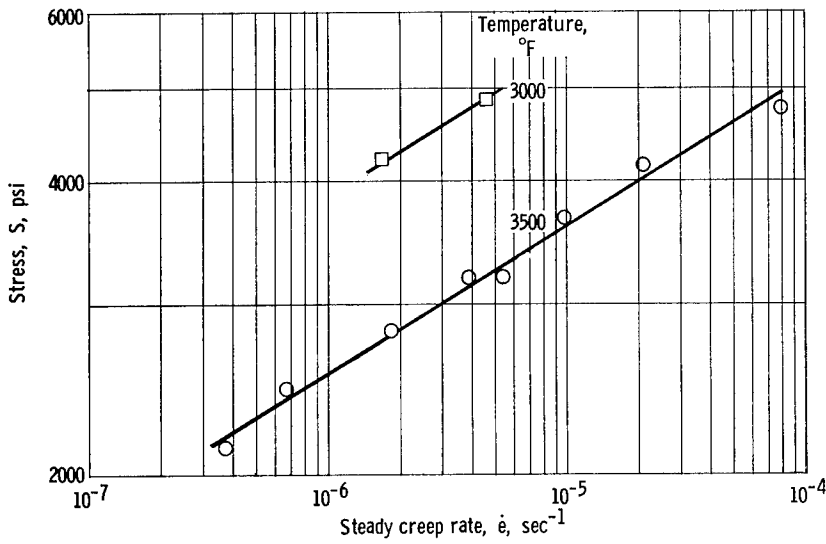
Figure 12. - Steady creep rate plotted against stress for electron-beam-melted tungsten.
