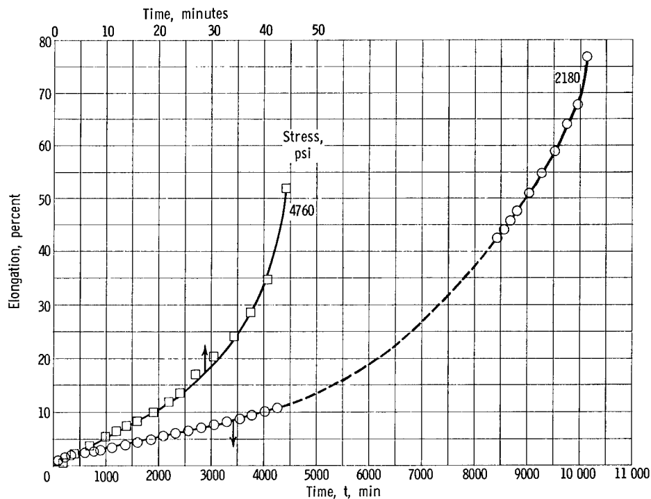
Figure 11. - Constant-load creep curves for electron-beam-melted tungsten at 3500° F.
