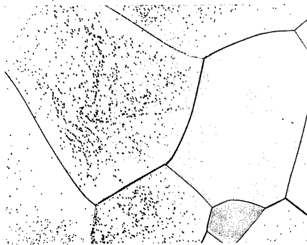
(e) Annealed for 1 hour at 3200° F; fully recrystallized; average grain diameter, 0.0731 centimeter.
