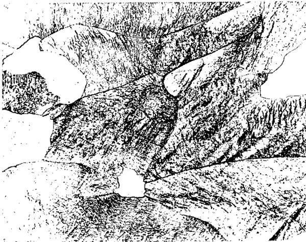
(a) Annealed for 1/2 hour at 2300° F; 46 percent recrystallized.
