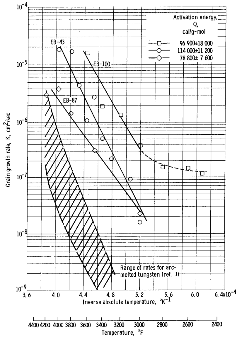
Figure 3. - Grain growth rates of electron-beam-melted tungsten.
