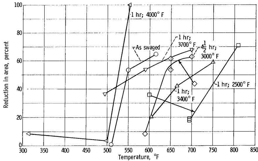
Figure 4. - Low-temperature tensile ductility of electron-beam-melted tungsten after various annealing treatments (lot EB-43).
