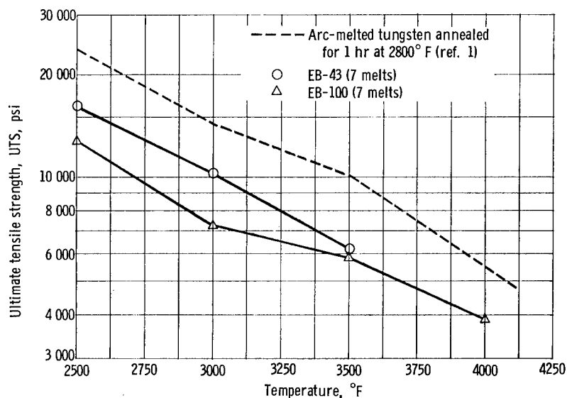
Figure 6. - Ultimate tensile strength of electron-beam-melted tungsten (annealed at 3600° F) and arc-melted tungsten (annealed at 2800° F) at 2500° to 4140° F.
