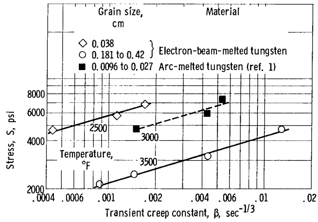
Figure 16. - Transient creep constant as function of stress.
