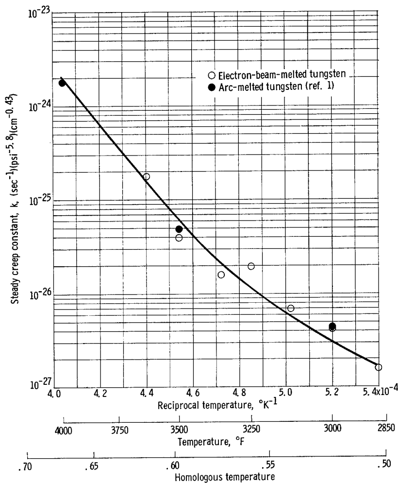
Figure 15. - Temperature dependence of steady creep constant. Activation energy, 141\,000 \pm 4\,000 calories per gram mol.
