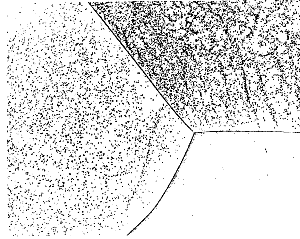
(f) Annealed for 1 hour at 3600° F; fully recrystallized; average grain diameter, 0.2147 centimeter.
