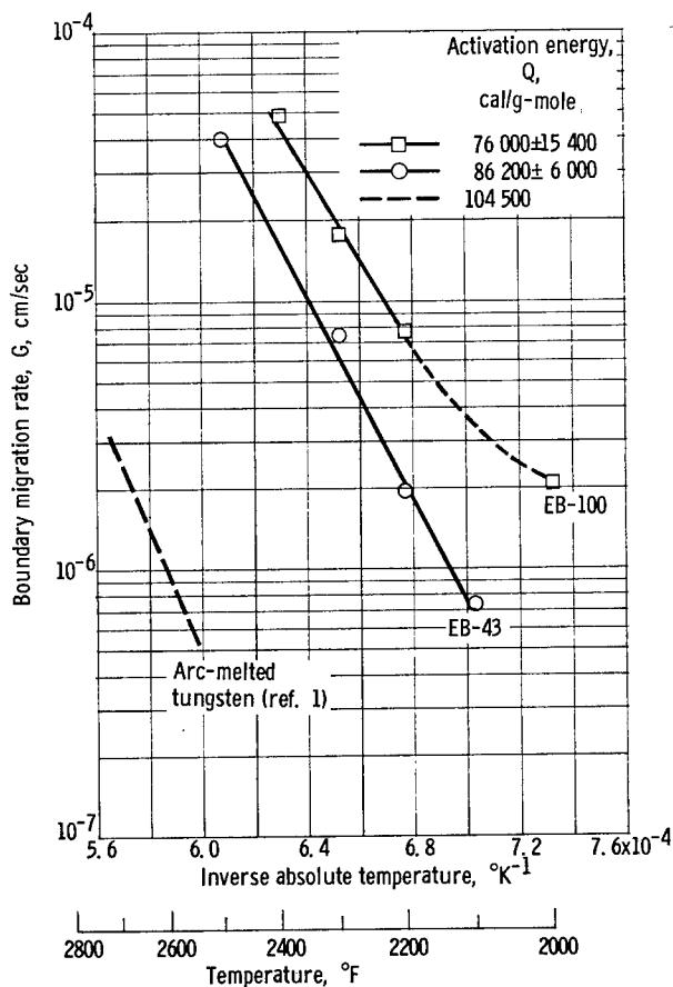
Figure 2. - Temperature dependence of strain-induced boundary migration rates of electron-beam- and arc-melted tungsten.
