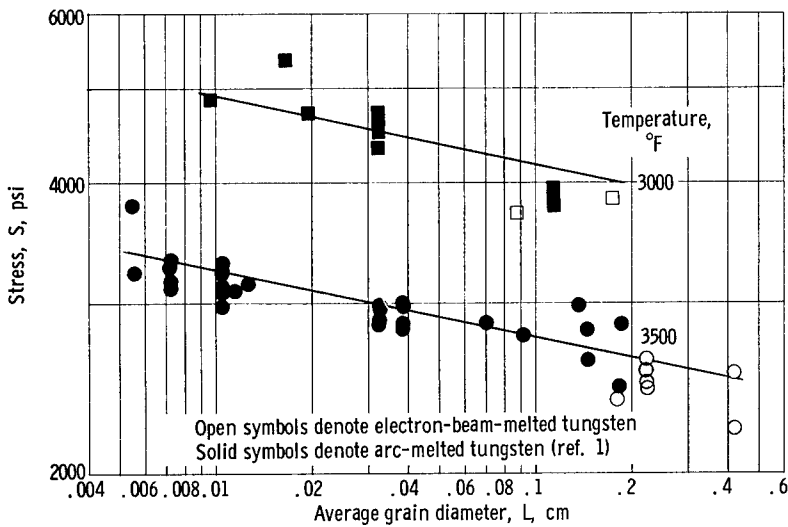
Figure 13. - Grain-size dependency of stress for steady creep rate of 10^{-6} per second.
