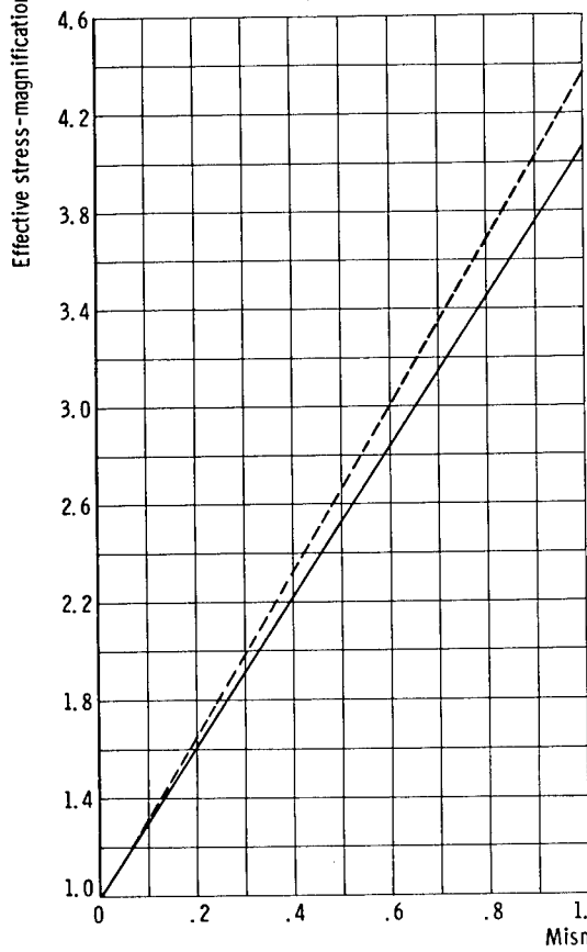
(c) Longitudinal joint in cylindrical pressure vessel (stress ratio, 2).
