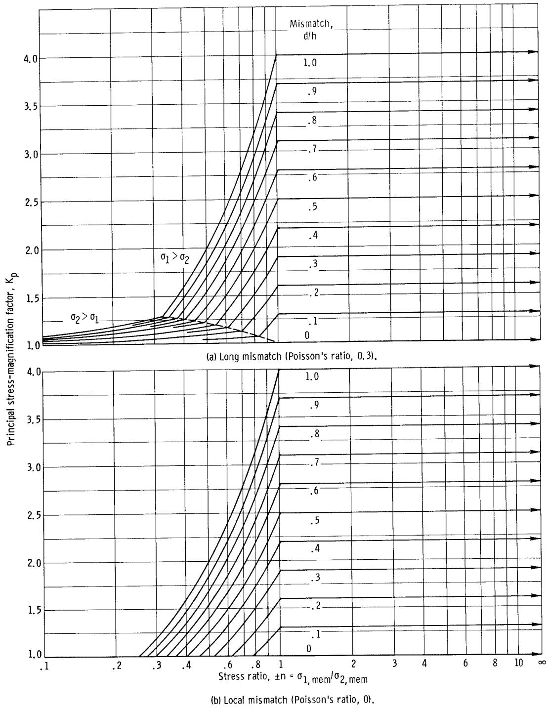
Figure 3. - Principal stress-magnification factors for mismatch.
