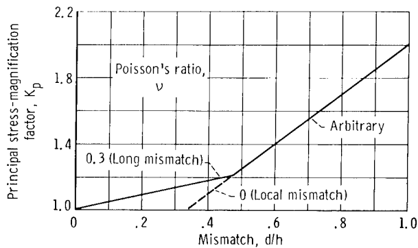
Figure 4. - Principal stress-magnification factors for circumferential joint in cylindrical pressure vessel. Stress ratio, 1/2.
