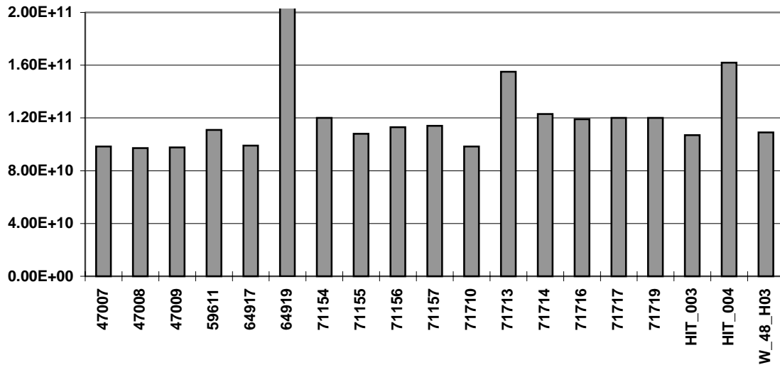
Figure 18 - Noise Equivalent Irradiance of EKV IR2 (VLWIR) FPAs.
