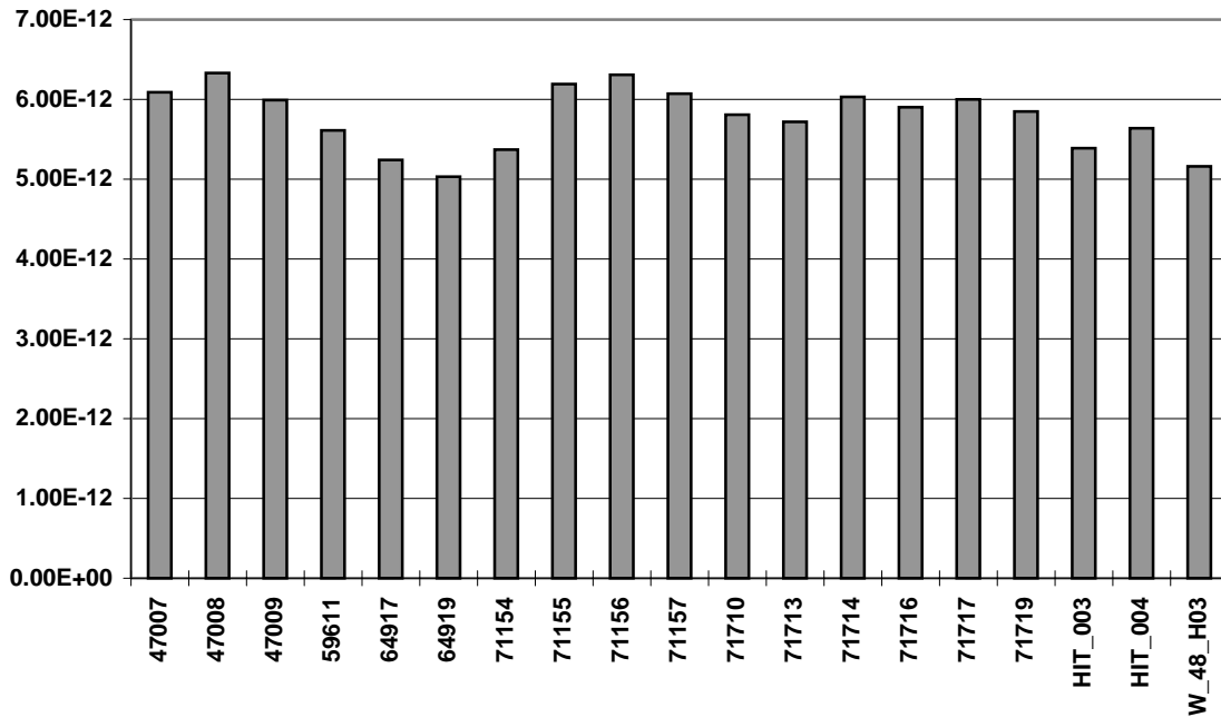
Figure 16 - Responsivity of EKV IR2 (VLWIR) FPAs.
