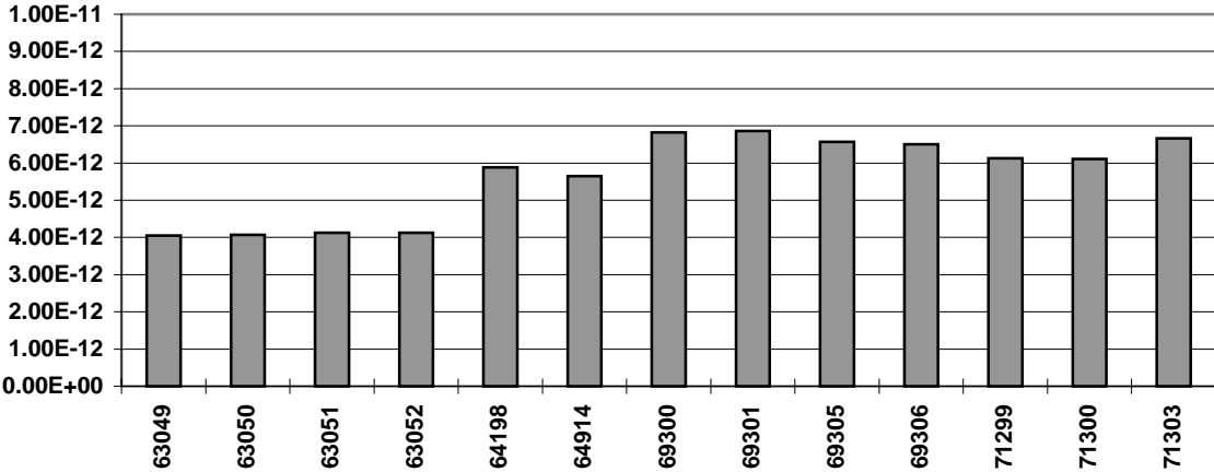
Figure 11 - Responsivity of EKV IR1 (LWIR) FPAs.
