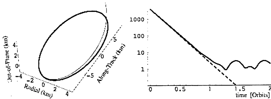
a) Relative Orbit shown in Chief LVLH Frame b) Tracking Error (m) Fig 6 Simulation Results using Hybrid Feedback control
