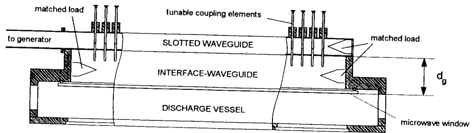
Fig.1.11. Scheme of the side view of a long planar plasma source with the modified slotted waveguide applicator described in Fig.1.10 [61].
