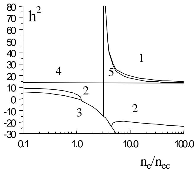
Fig. 2.4. The waves in system a plasma - dielectric waveguide in absence of collisions. 1 - The surface wave existing in an area \epsilon_p < -\epsilon_D ; 2 - dielectric waveguide wave existing in an area \epsilon_p > \epsilon_D ; 3 - boundary infinite spectrum, 4 - k_0^2 \epsilon_D ; 5 - calculation under the equation (2.7) ( \epsilon_D = 5 , antenna thickness L=8 mm, microwave length \lambda=2.4 cm, n_C = m\omega^2/4\pi e^2 ).
