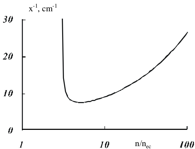
Fig. 2.5. Inverse penetration depth x^{-1} of a surface wave as a function of electron density at v/\omega=0 .
