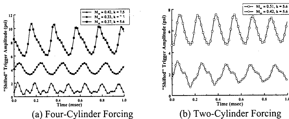
Figure 18: Vertically-Shifted Trigger Signals: Four-Cylinder and Two-Cylinder Forcing.
