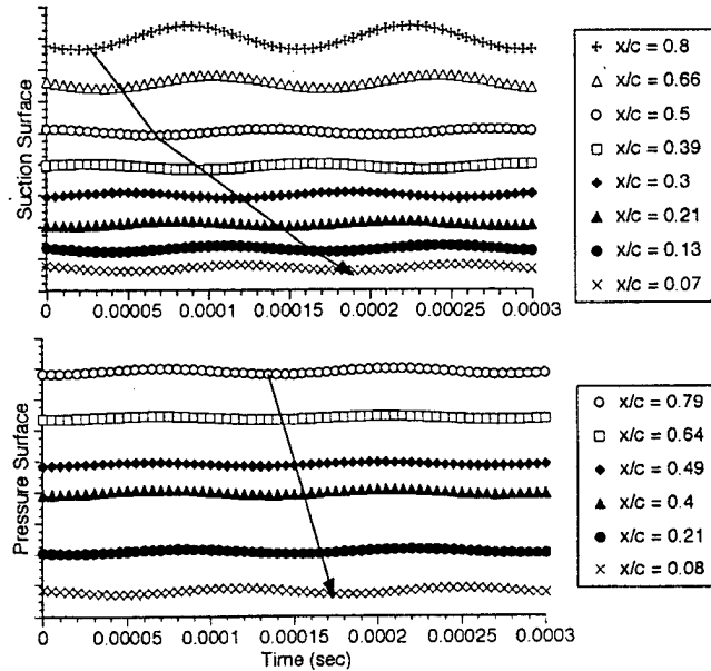
Figure A6. Primary-Frequency Component Time Series
