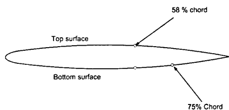
Figure 5. Schematic of Vane Showing the Location of the Three Operable Transducers.
