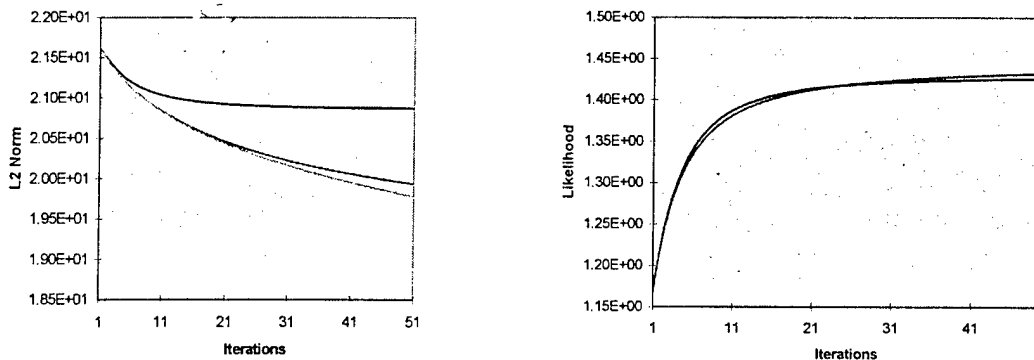
Fig. 5a. Convergence of restoration error Fig. 5b. Likelihood increase with progress of iterations
