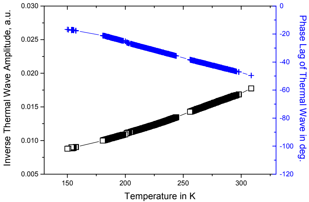
Fig. 5.5. Temperature dependencies of the phase lag (crosses) and the inverse value of the amplitude (squares) of the thermal wave transmitted through the \text{BaWO}_4 sample at the frequency 2Hz in AC experiment.
