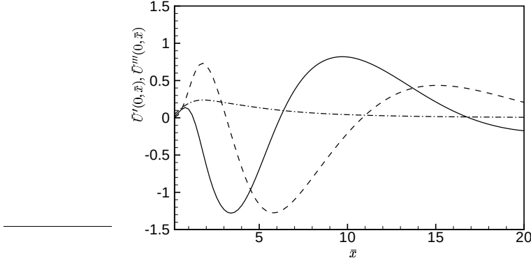
FIG. 2.1. Variation of U'''(0, \bar{x}) (solid line: real part, dashed line: imaginary part) and |U'(0, \bar{x})| (— · — · —) with \bar{x} .
