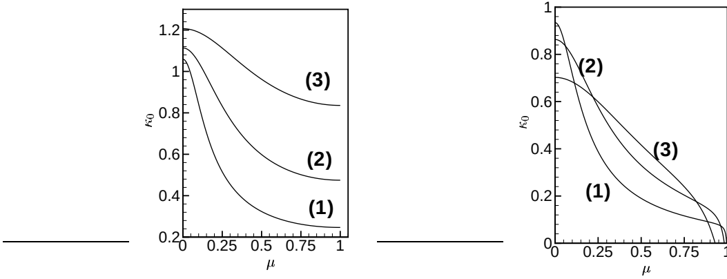
FIG. 5.1. ‘Unit growth rates’ of Floquet modes v.s. \mu . Left: branch-I modes; Right: Branch-II modes. Curves (1)-(3) in each figure correspond to B_0 = 0.5, 1, 2 .
