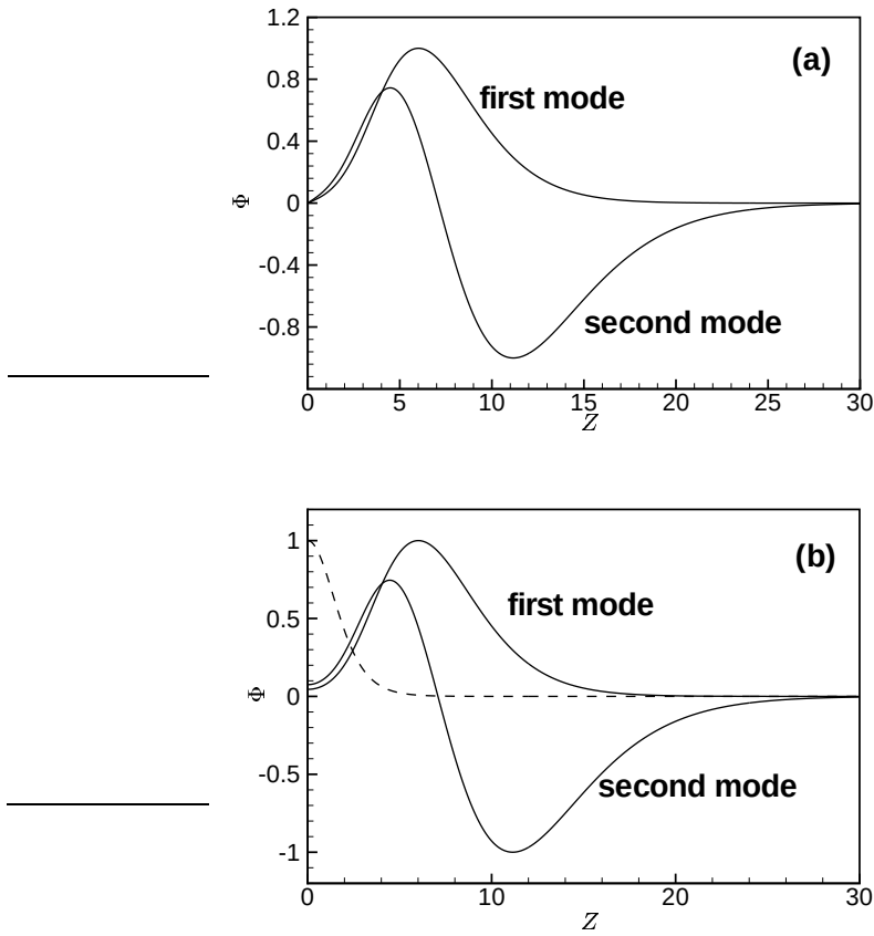
FIG. 3.3. Eigenfunctions of the first and second modes for the localised Klebanoff distortion defined by (3.36): sinuous mode (a) and varicose mode (b) for d = 4 and B_0 = -1 . For comparison, the dashed line represents the eigenfunction of the varicose mode for d = 4 and B_0 = 1 .
