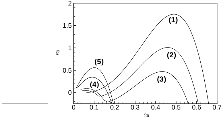
FIG. 5.2. Growth rates of Goldstein-Wundrow modes. The parameters B_0 = 4 , \bar{x} = 1.2 and \bar{t} \approx -1.498 . Curves (1)-(5) correspond to \beta = 0.063, 0.125, 0.16, 0.18, 0.44 .
