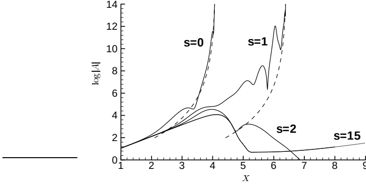
FIG. 4.1. Nonlinear evolution of the most unstable (sinuous) mode in figure 3.6b ( B_0 = 1.4 , \hat{x} = 1.2 , \omega = 0.65 ) for viscosity parameter s = 0, 1.0, 2.0 and 15.0 . The dashed line represents the local singular solution (4.5).
