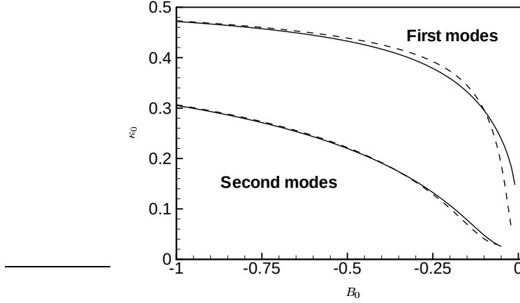
FIG. 3.4. Variation of the ‘unit growth rate’ with B_0 . Solid line: varicose modes; dashed line: sinuous modes.
