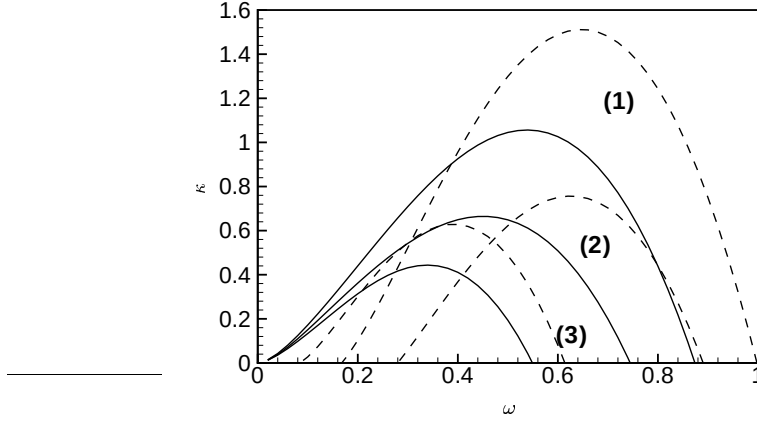
FIG. 3.5. Instability caused by a Klebanoff distortion. The streamwise location is fixed at \bar{x} = 2.0 and B_0 = 1.4 . The figure shows the growth rates of varicose (solid line) and sinuous modes (dashed line) at three instants: (1) \bar{t} = \phi(x) - \frac{3}{4}\pi ; (2) \bar{t} = \phi(x) - \frac{7}{8}\pi ; (3) \bar{t} = \phi(x) - \frac{29}{32}\pi , where \phi(\bar{x}) \approx 2.31 denotes the local phase of the wall torsion \bar{U}'''(0, \bar{x}) .
