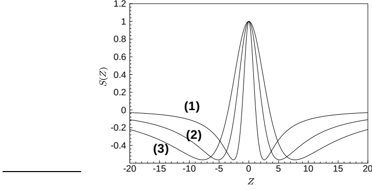
FIG. 3.1. The shape of the distortion. Curves (1)-(3) correspond to d = 2, 4, 6
