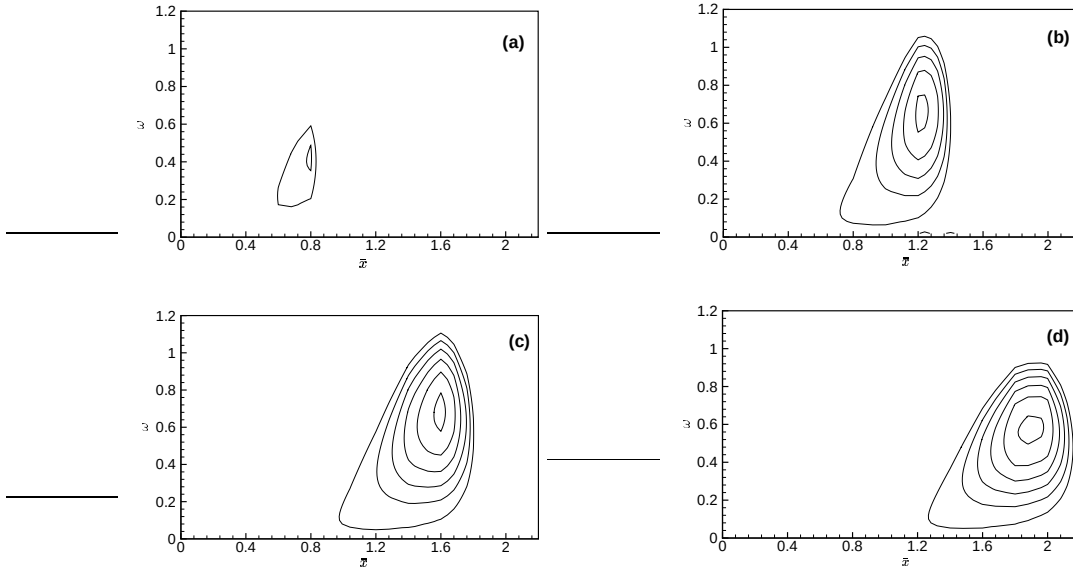
FIG. 3.6. Contours of growth rates of the local instability induced by a Klebanoff mode ( B_0 = 1.4 ). Figures (a)-(d) correspond to the instants \bar{t} = -1.8, -1.25, -0.82, -0.44 .
