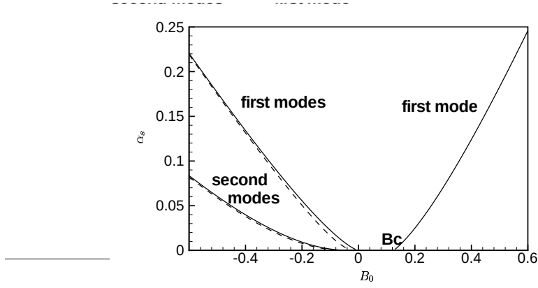
FIG. 3.2. Eigenvalues \alpha_s versus B_0 : solid line: varicose modes, dashed line: sinuous modes.
