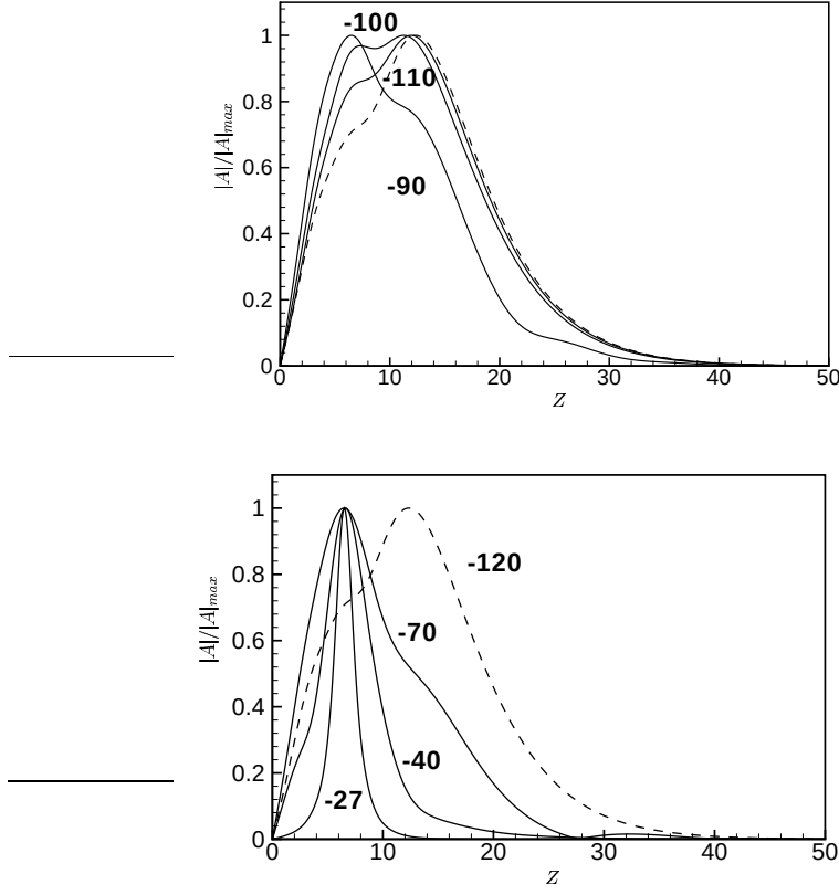
FIG. 4.3. Spanwise distribution of |A| at different values of \tilde{X} .
