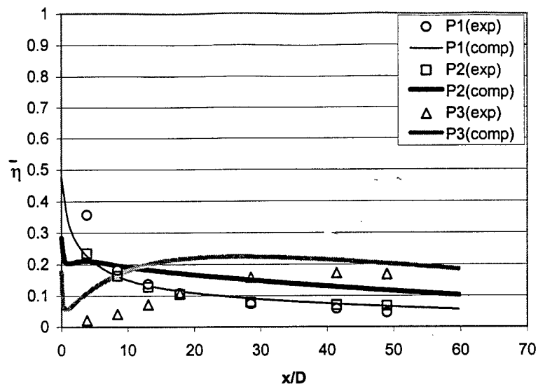
Figure 9. Laterally-averaged adiabatic effectiveness for the three PS cases show agreement with experimental trends, but significant overprediction as M increases.
