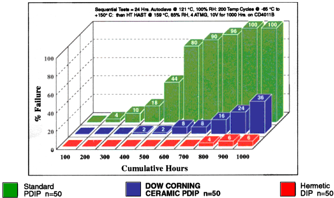
Figure 6. Sequential HAST Test Results for Ceramic-Coated/Plastic Encapsulated CD4011 CMOS Devices
