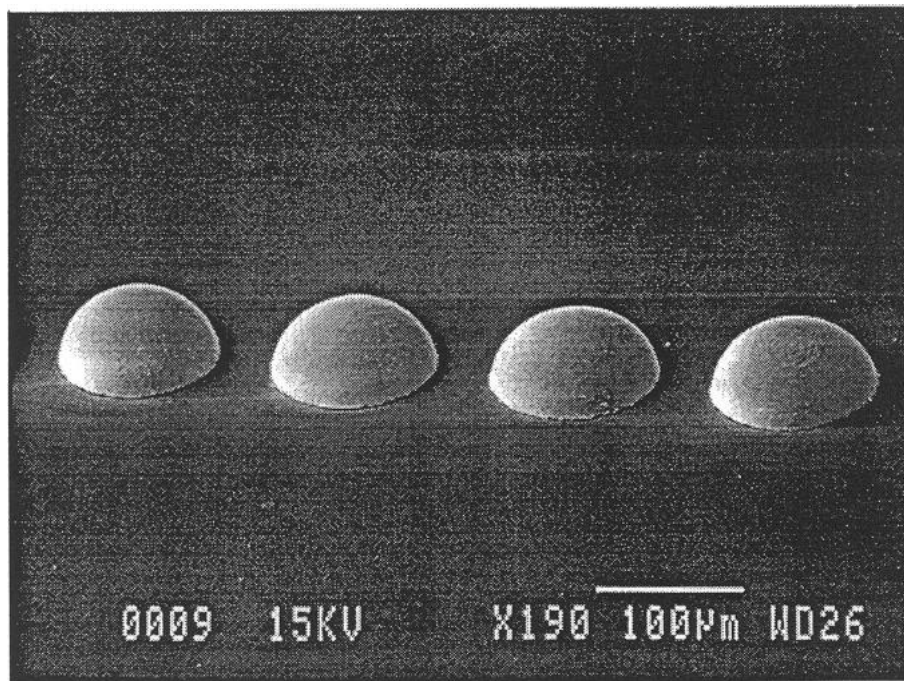
Figure 39. Photomicrograph of 100 \mu\text{m} Diameter Solder Bumps
