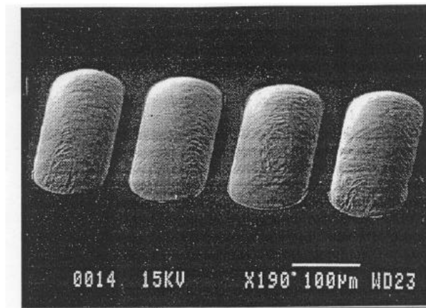
Figure 40. Photomicrograph of 100 by 300 \mu\text{m} Bump Designs
