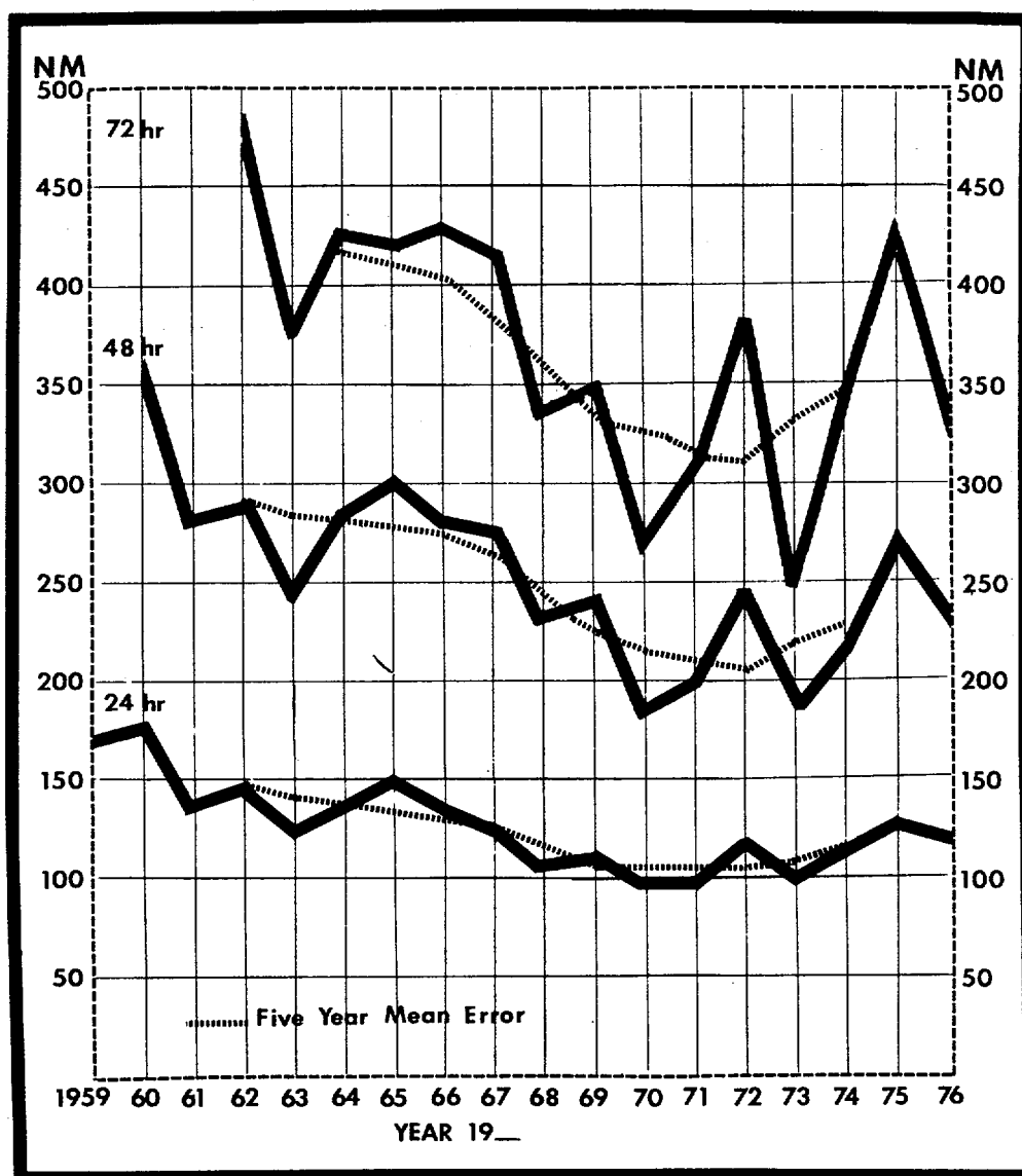
FIGURE 5-1. Mean vector error for the Pacific Area.
