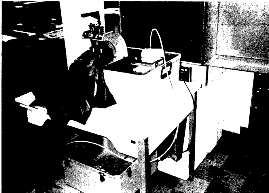
Figure 5. The nondestructive cell mounted in the portable tester.
