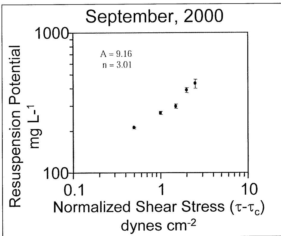
Figure 16. Relationships between calculated shear stress minus critical shear stress ( \tau_c ) and net TSS resuspension. See text for explanation of calculation of net TSS resuspension
