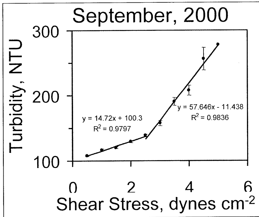
Figure 13. Relationships between mean turbidity ( \pm 1 S.E.) and calculated shear stress at the resuspension station for September 2000. Shear stress was calculated using Equation 3
