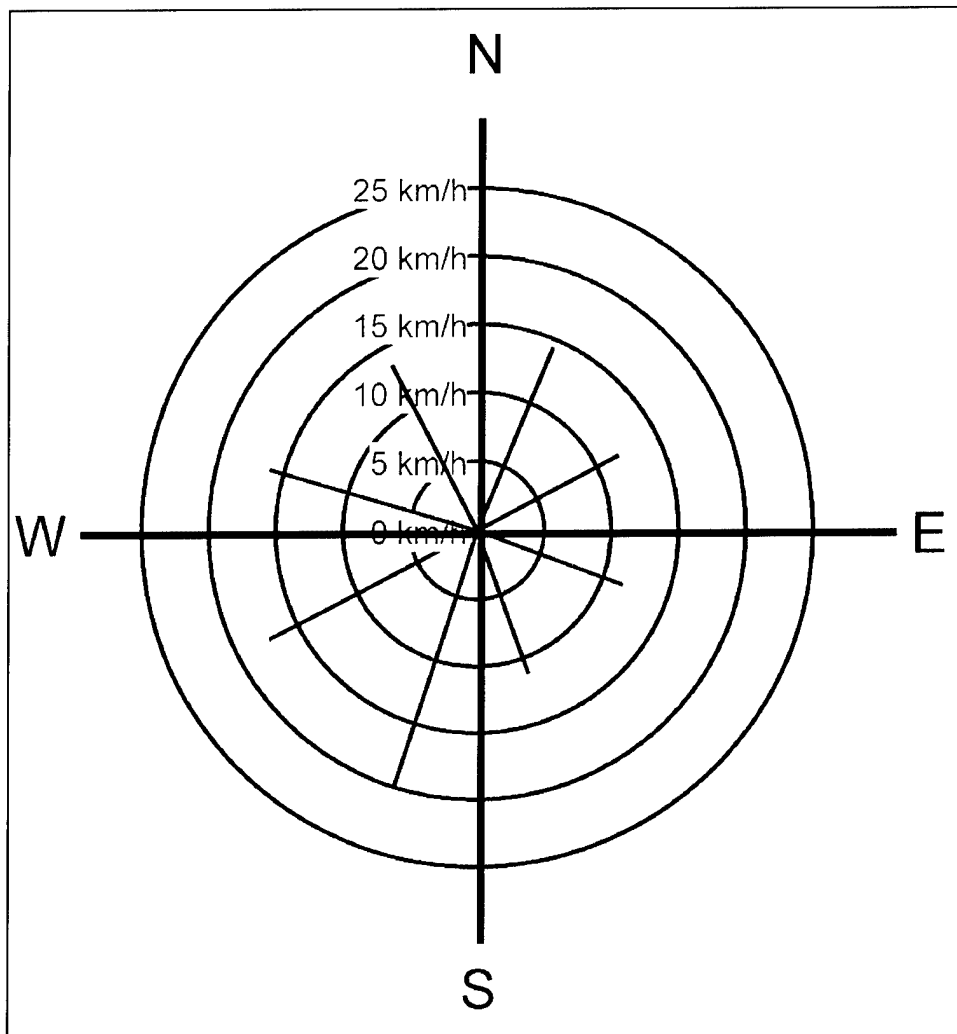
Figure 10. Variations in the average wind speed of winds blowing out of the NNE, ENE, ESE, SSE, SSW, WSW, WNW, and NNW at the resuspension station, Peoria Lake
