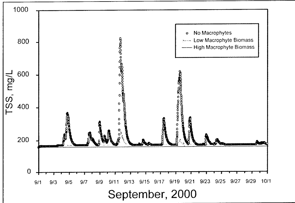
Figure 27. Variations in simulated TSS concentrations at the resuspension station, Peoria Lake, in the absence of submersed macrophytes and in the presence of low ( < 20 \text{ g m}^{-2} ) and high ( > 200 \text{ g m}^{-2} ) macrophyte biomass
