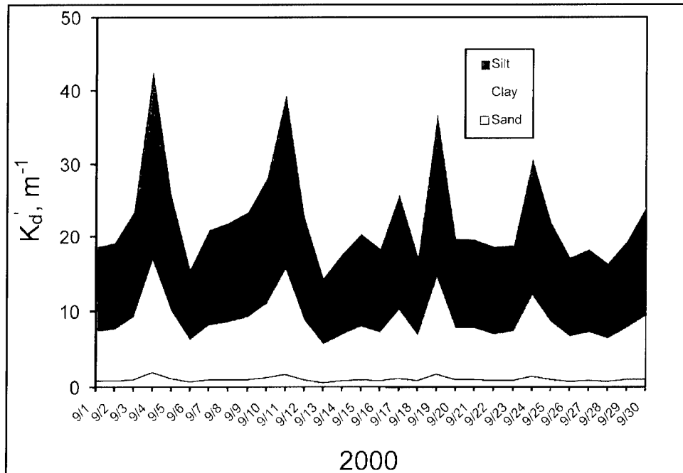
Figure 26. Variations in the daily calculated light attenuation coefficient ( K_d' ) for the month of September. K_d' (representing the sum of the sand, silt, and clay fractions) was determined via empirical conversion of the beam attenuation coefficient ( \epsilon , m^{-1} ; Figure 24) for the sand, silt, and clay fractions.
