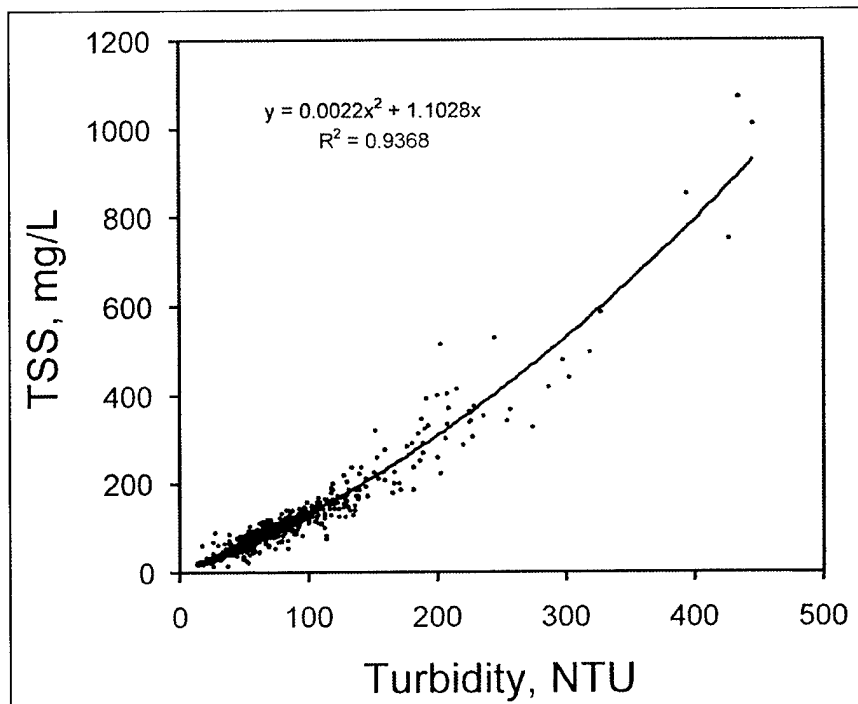
Figure 14. Relationships between turbidity and TSS
