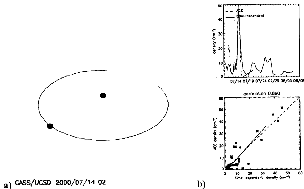
Fig. 8. a) Remote observer view of the heliosphere on July 14, 2000 from 30^\circ above the ecliptic plane and 45^\circ west of the Sun-Earth line. b) Time-series correlation during the event sequence.
