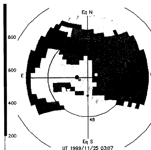
Fig. 9a. A recent sample sky sweep map showing the ambient solar wind velocities as observed from Earth with the IPS sources observed over the most recent 24-hour period superposed. The color of the source is the velocity observed for that source and the size of the source depicts the difference of the source from the nominal velocity at that location.
