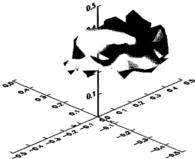
Fig. 3. Three dimensional density plot of the deconvolved 24 May 1979 CME as derived from SOLWIND coronagraph and HELIOS photometer data. The perspective view is from 30^\circ above the ecliptic plane and 135^\circ to the east of the Sun-Earth line. Distances on the axes are in AU. The contoured surface is a density level of 50 \text{ electrons cm}^{-3} or greater.
