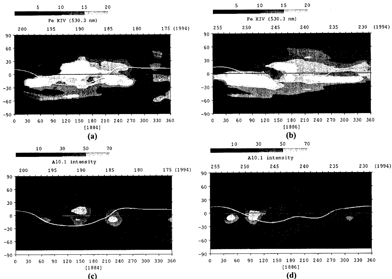
Fig. 6. Carrington synoptic map presentations of quiet Sun structure for rotation 1884 and 1886. (a), (b) Sacramento Peak Observatory coronagraph data from Fe XIV limb scans at 1.15 R_s . (c), (d) YOHKOH SXT central limb data (assumed at a height of 1.15 R_s degraded to a 10^\circ \times 10^\circ resolution).
