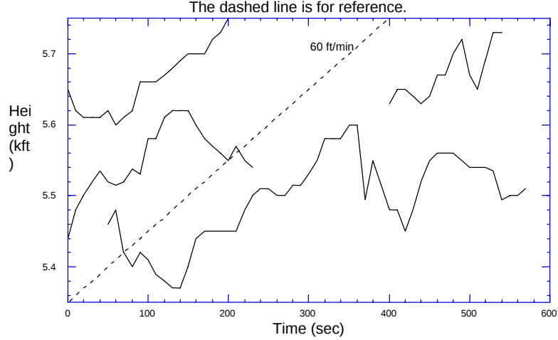
Figure 11: Four altitude drift records during Cessna flight with manual pilot control during smooth to light chop conditions.
