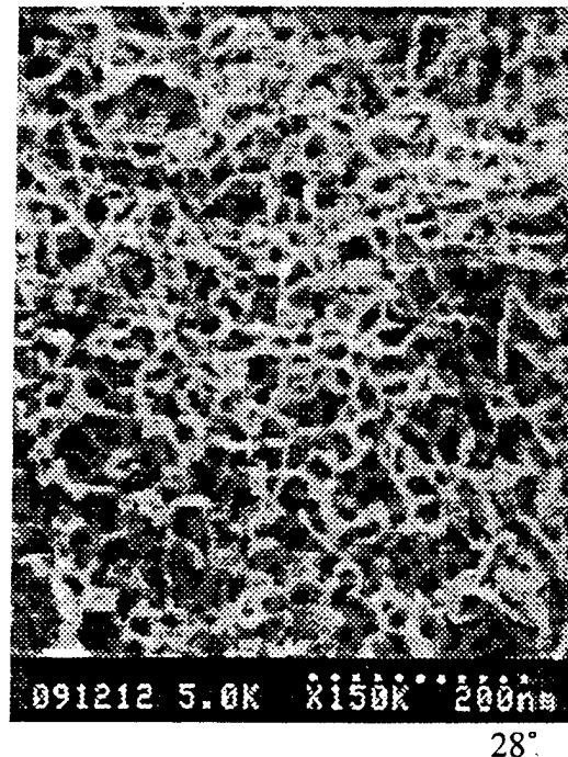
(b) Anodized with PACS Procedure
