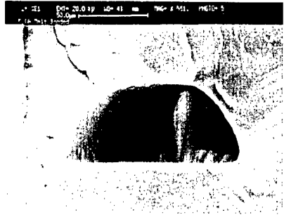
Figure 5 – SEM of 100 micron isotropic channel patterned PLGA bonded to a flat piece of PLGA.
