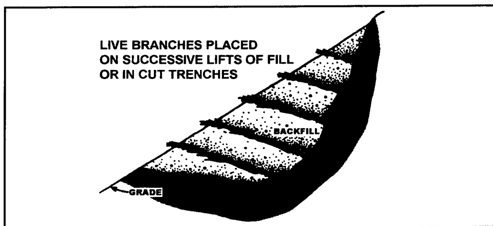
Figure 4. Schematic diagram of brushlayering (from Leiser 1983)
