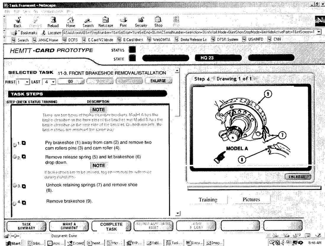
Figure 3-11. Integrated Technical Data in the AMS
