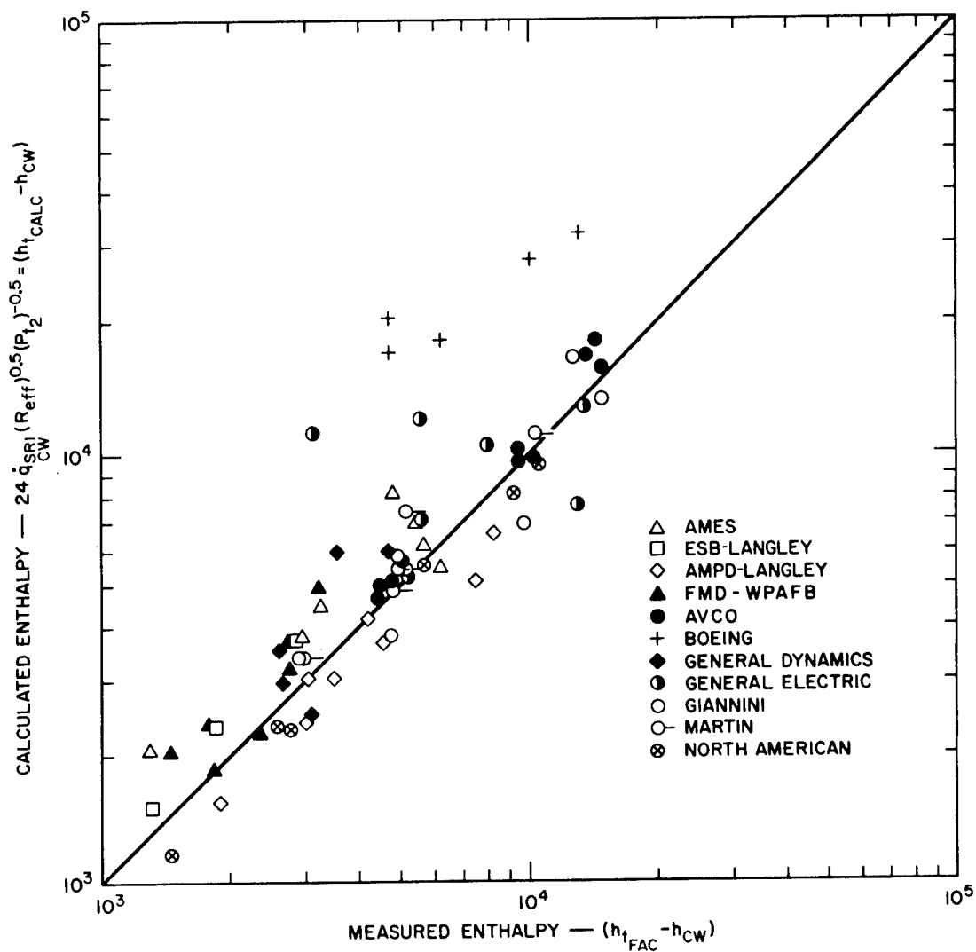
FIG. 21 ENTHALPY CALCULATED FROM HEATING RATE VERSUS ENTHALPY MEASURED BY THE FACILITY
