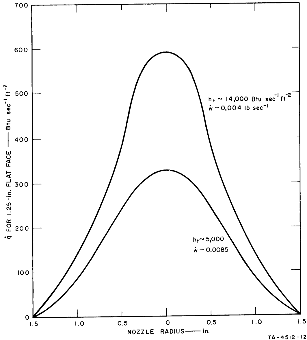
FIG. 18 THE BOEING COMPANY HEATING RATE PROFILE
