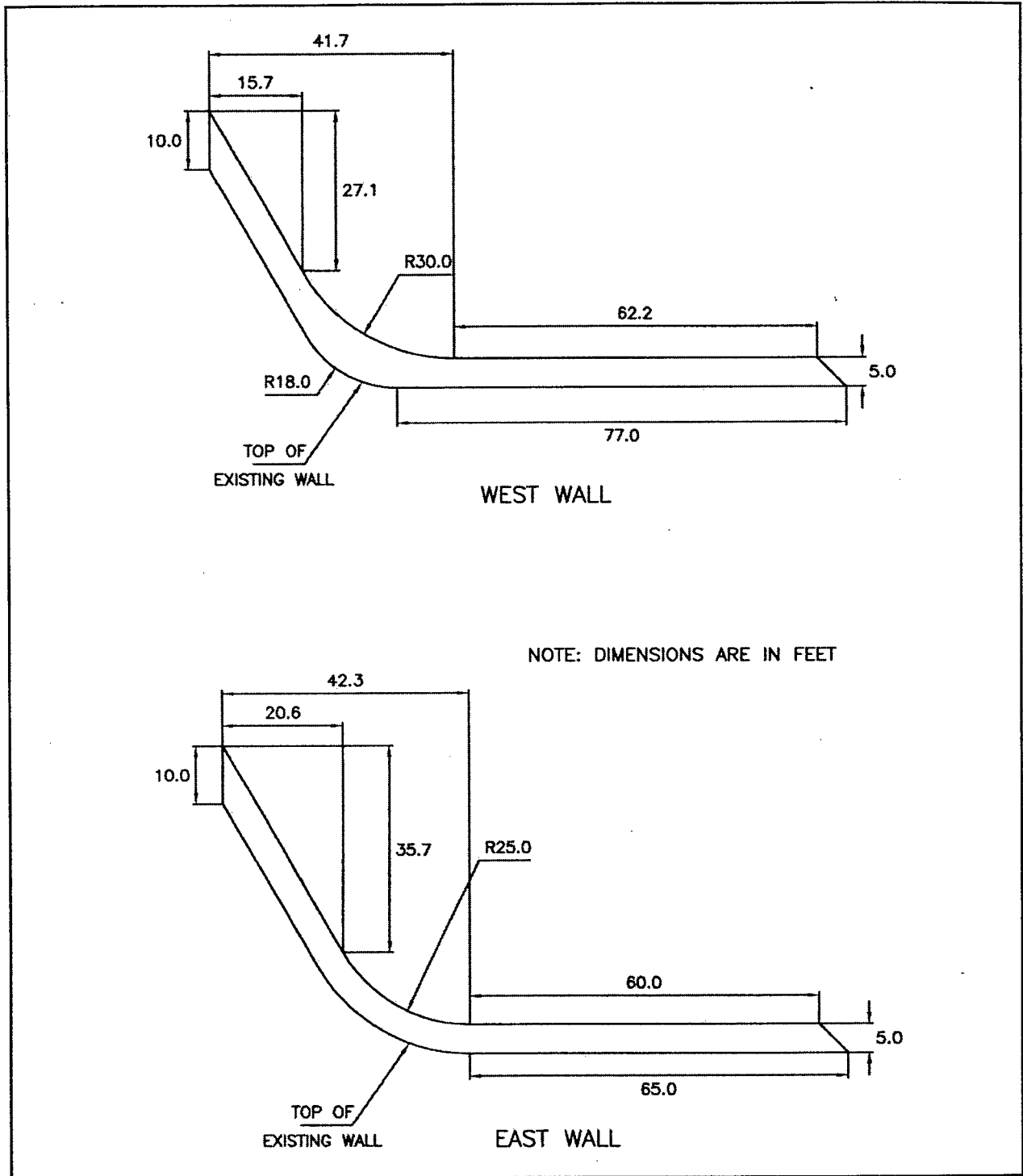
Figure 32. Final training wall designs
