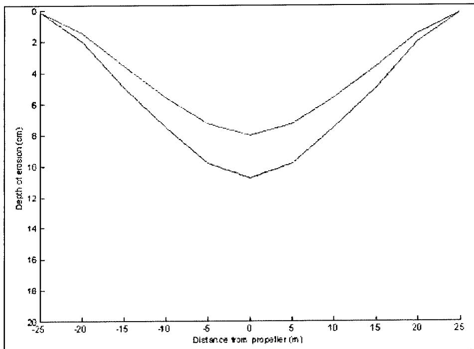
Figure 56. Scenario 2 (ship speed = 1.5 m/sec, water level elevation = 3.4 ft (mllw)) maximum depth of erosion (blue line) and change in depth after 700 sec (red line) perpendicular to the direction of ship movement, for midchannel sediments (after Gailani 2001)
