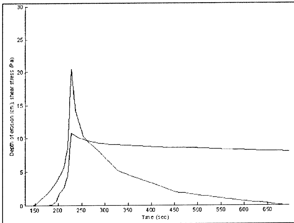
Figure 55. Scenario 2 (ship speed = 1.5 m/sec, water level elevation = 3.4 ft (mllw)) shear stress (red line) and depth of erosion (blue line) time-history under propeller for midchannel sediments (after Gailani 2001)
