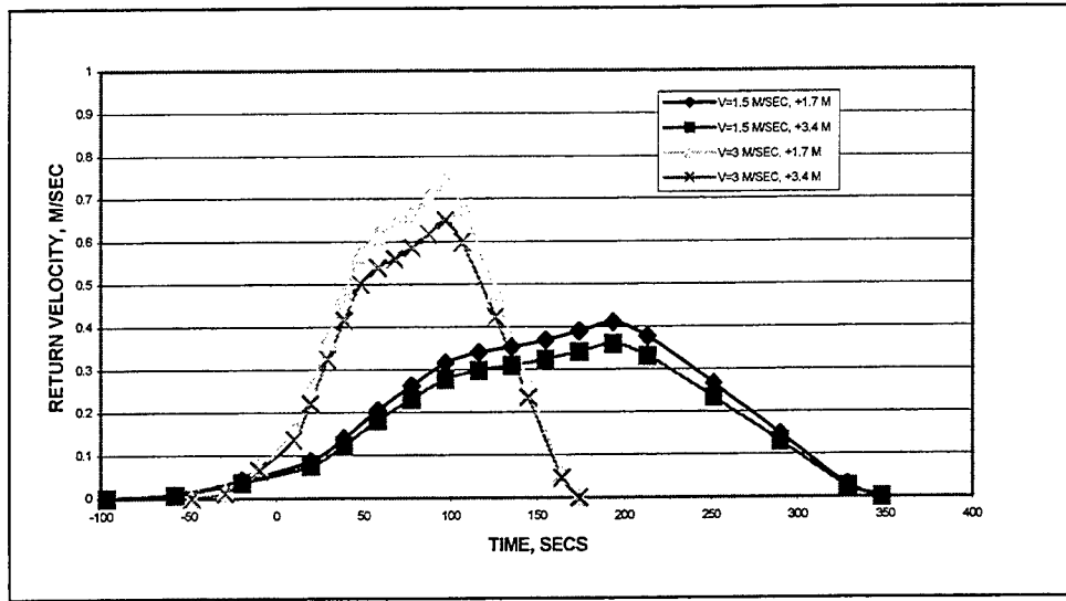
Figure 28. Return velocity time-history, MV Matthew (return velocity computed for south side of ship) (after Maynard 2001)
