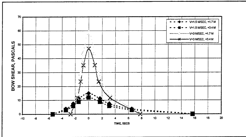
Figure 30. Bow shear time-history, MV Matthew (after Maynard 2001)
