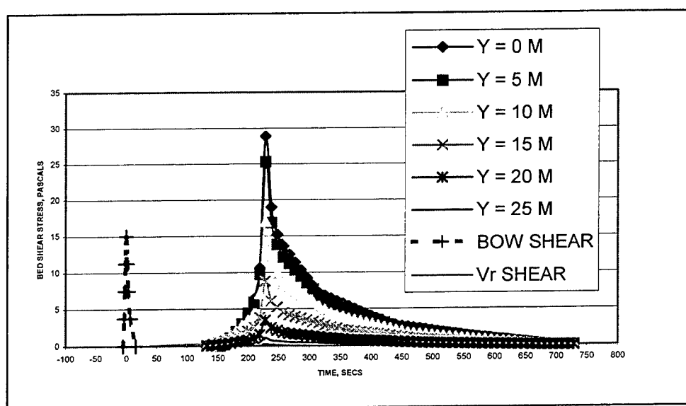
Figure 35. All shear sources versus time, MV Matthew (water level = +1.7 m (mllw); ship speed = 1.3 m/sec for propeller, and ship speed = 1.5 m/sec for return velocity, shear, and bow shear) (after Maynard 2001)
