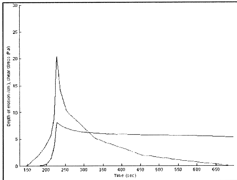
Figure 57. Scenario 2 (ship speed = 1.5 m/sec, water level elevation = 3.4 ft (mllw)) shear stress (red line) and depth of erosion (blue line) time-history under propeller for open cell sediments (after Gailani 2001)
