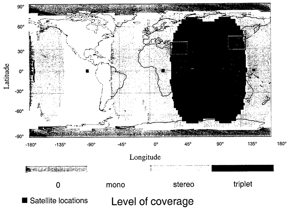
Figure 13. Line-of-sight coverage of two theaters by five “pinched” geostationary satellites.
