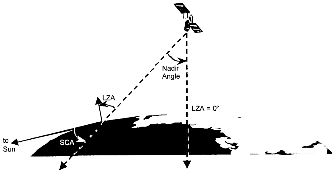
Figure 8. Solar scatter geometry: as the sensor line of sight shifts from nadir to the limb, both the range to target and the path length through the atmosphere increase while the minimum possible solar scatter angle (SCA) decreases.
