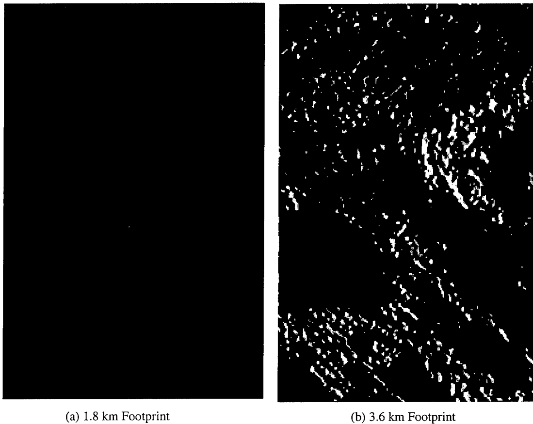
Figure 11. Simulation of an IR scanner: outputs thresholded at 6 kW/sr for the stressing background scene.
