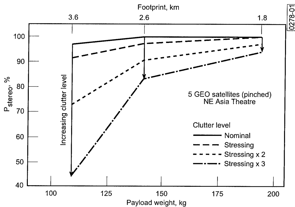
Figure 16. Weight and performance sensitivity to sensor footprint and clutter.
