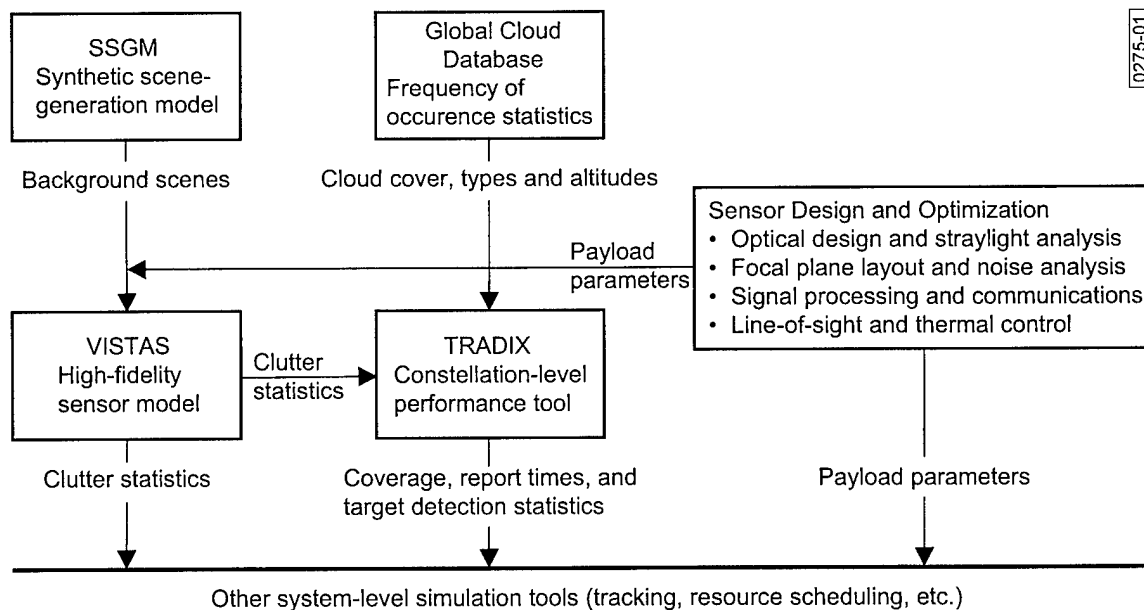
Figure 4. Flowchart of integrated electro-optical sensor design and simulation.
