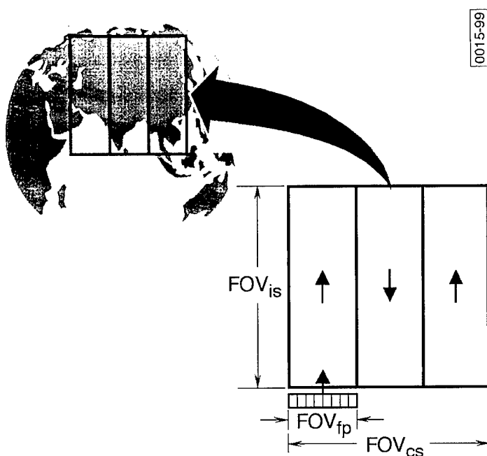
Figure 1. Scan pattern of conceptual sensor for theater missile surveillance.
