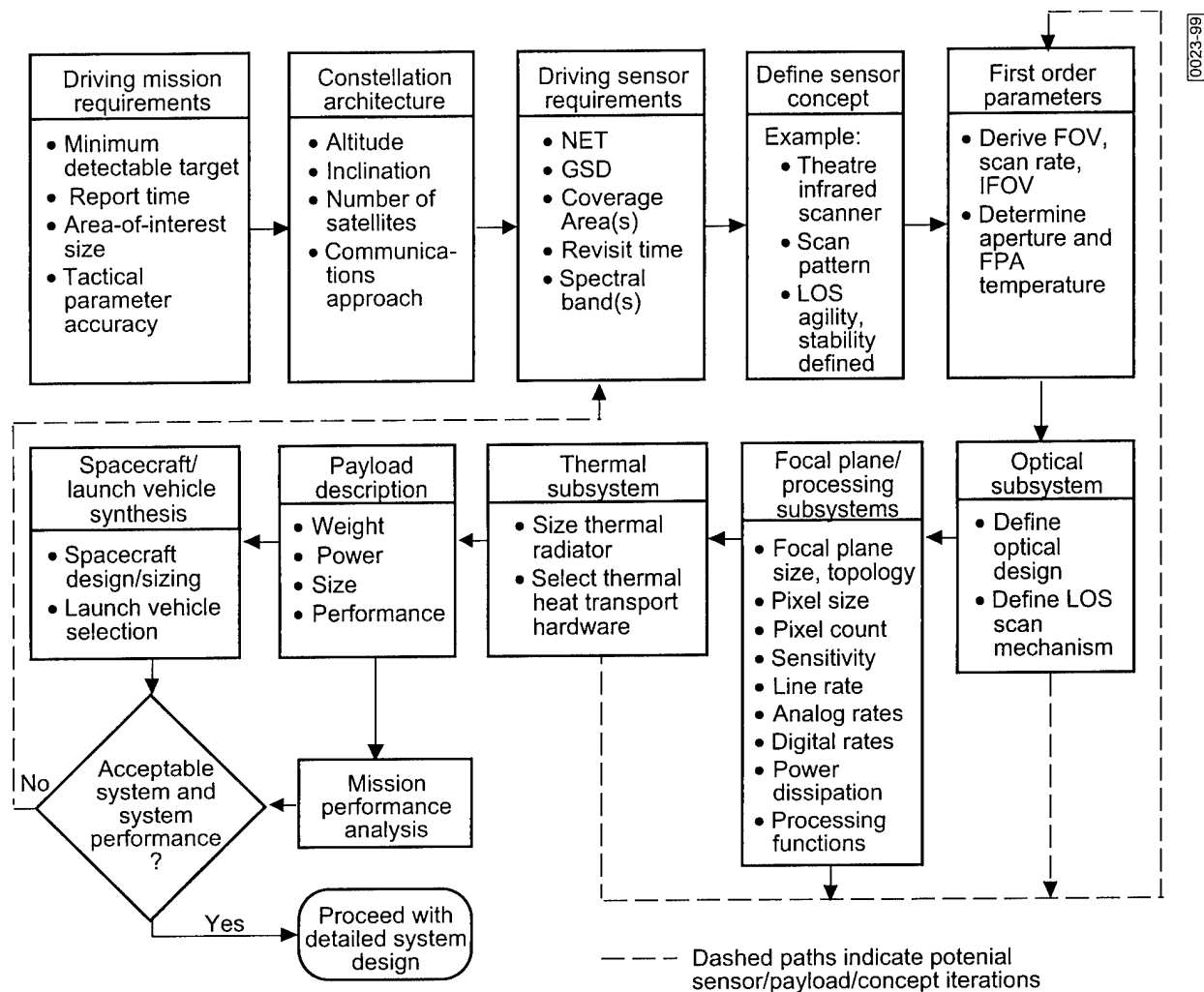
Figure 2. Flowdown of mission requirements to payload sizing and launch vehicle selection for an infrared scanner.
