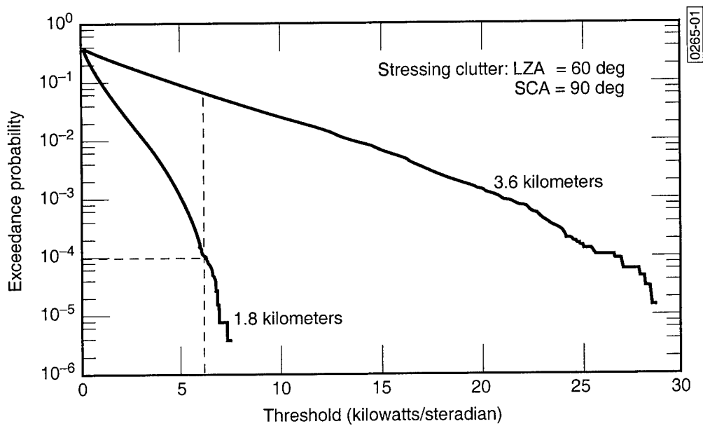
Figure 10. Probability of False Exceedance vs. threshold intensity for IR scanners viewing the stressing background scene.
