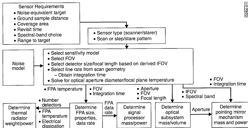
Figure 3. Driving sensor requirements for a hypothetical theater missile surveillance system.
