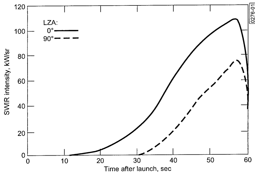
Figure 12. Theater missile SWIR intensity vs. time after launch when viewed at nadir and the limb; includes attenuation by the atmosphere.
