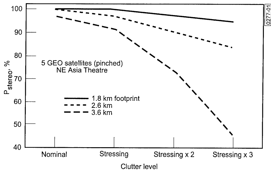
Figure 15. TMW stereo performance sensitivity to sensor footprint and clutter.
