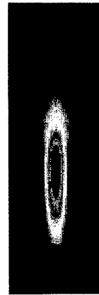
Fig. 3. Evolution of the system. The vertical axis is the magnitude of the order parameter.
