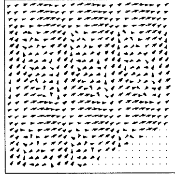
velocity field
