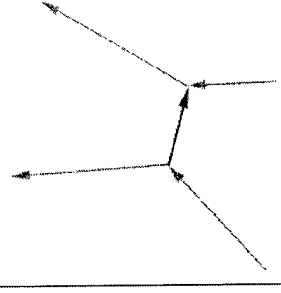
bubble chamber
