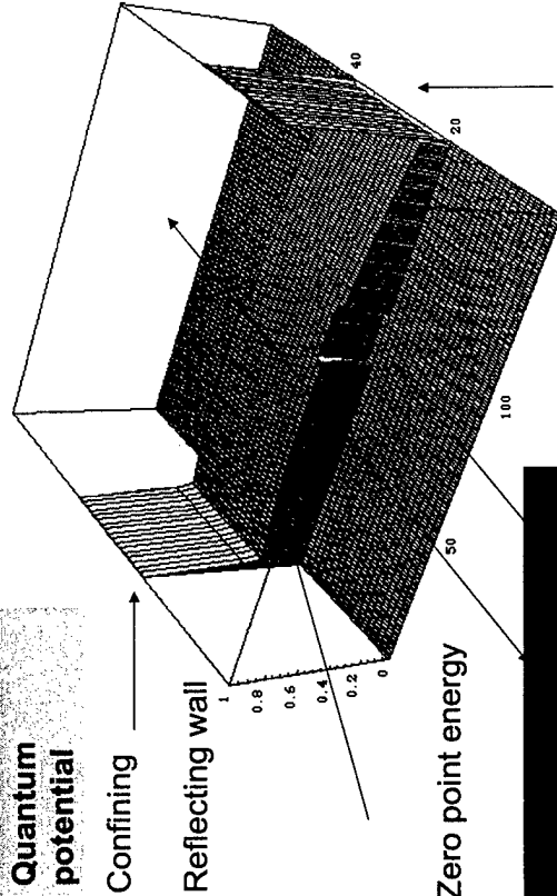
Note long range of V_Q
