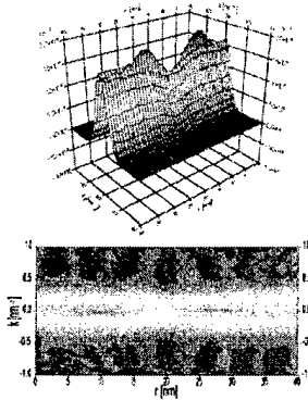
Obtained by means of W . Paths with potential scattering in a Monte Carlo approach
