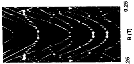
Tunneling conductance of closed dot
