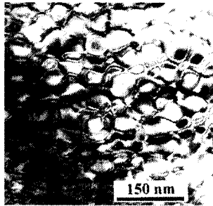
Fig. 17 TEM image of Y(\text{Co,Fe,Cu,Zr})_z compounds
