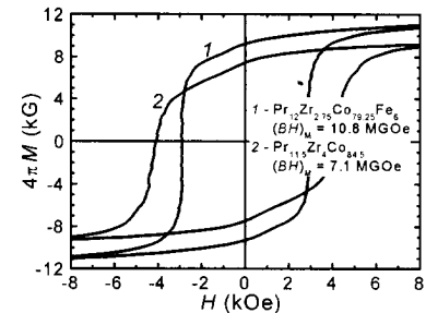
Fig. 19 Hysteresis loop of \text{Pr}(\text{Co,Fe,Zr})_z compounds
