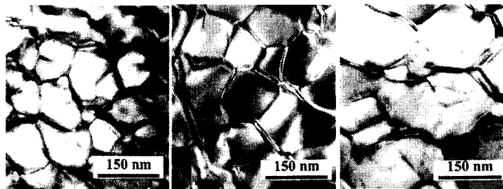
Fig. 4 Cellular microstructure of \text{Sm}(\text{Co}_{\text{bal}}\text{Fe}_{0.224}\text{Cu}_{0.08}\text{Zr}_{0.033})_z magnets with (a) z=7.0 , H_{ci}=15 kOe, (b) z=8.5 , H_{ci}=35 kOe and z=9.1 , H_{ci}=8 kOe.
