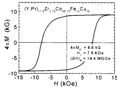
Fig. 18 Hysteresis loop of Y(\text{Co,Fe,Cu,Zr})_z compounds
