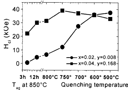
Fig. 13. Development of H_c with aging of \text{Sm}(\text{Co}_{\text{bal}}\text{Fe}_{0.1}\text{Cu}_{0.168}\text{Zr}_{0.04})_{8.5} magnets
