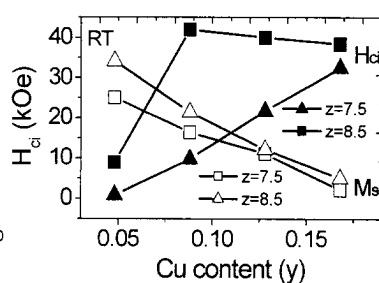
Fig. 6 M_s and H_{ci} of \text{Sm}(\text{Co}_{\text{bal}}\text{Fe}_{0.1}\text{Cu}_y\text{Zr}_{0.04})_z magnets ( y=0.048-0.168 , z=7.5 and 8.5 ) on the Cu content
