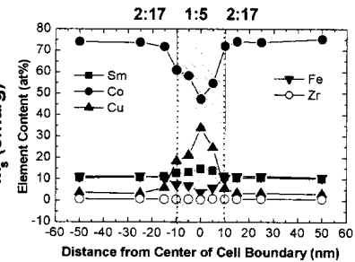
Fig. 7 Element profile in the 1:5 cell boundary
