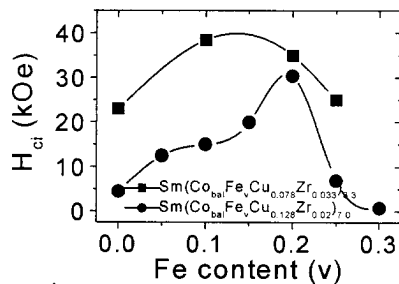
Fig. 10 H_c as a function of Fe content
