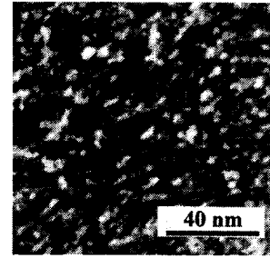
Fig. 14 TEM image of solutionized \text{Sm}(\text{Co}_{\text{bal}}\text{Fe}_{0.1}\text{Cu}_{0.168}\text{Zr}_{0.04})_{8.5} magnet
