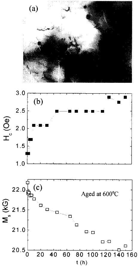
Fig. 3. Lorenz microscopy graph of magnetic domains pinned by second phases (a), and the effect of aging time on the magnetic properties of Hipercor 50 alloys (b and c).
