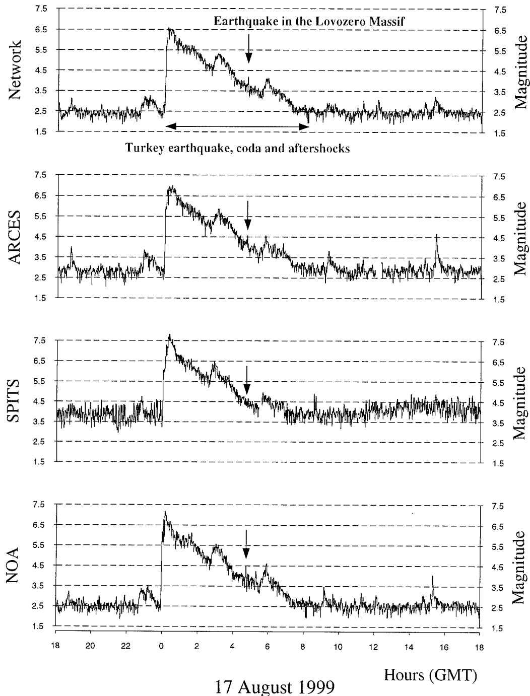
Figure 44. Surface threshold monitoring for the location of the Lovozero event of 17 August 1999, using data filtered between 17 and 24 s. The lower three traces represent thresholds (upper 90% magnitude limits) for each of the three stations; the top trace shows the combined network threshold. The peaks corresponding to the Lovozero event are indicated on each trace.
