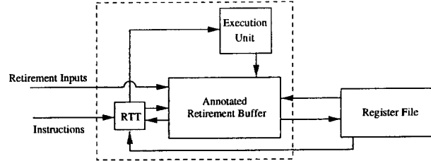
Fig. 2. Instruction flow in the intermediate abstraction.
