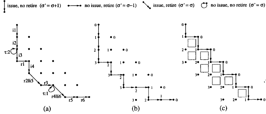
Fig. 3. (a) A Max-n execution \varepsilon_n . (b) An equivalent non-diagonal execution \varepsilon_{\hat{n}} . (c) An equivalent Max-1 execution \varepsilon_1 . Labels in and rn denote the issue and retirement of instruction number n . The label rn||in denotes simultaneous issue and retire. \tau : n is a shorthand for n cycles where in each cycle, bubbles are issued and nothing is retired. The numbers indicate the sizes of each state. The squares indicate the distance between \varepsilon_{\hat{n}} and \varepsilon_1 .
