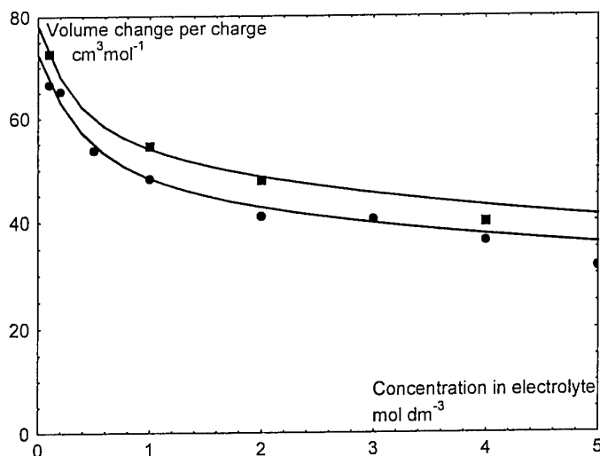
Figure 1: Expansion of two different PPy-DBS strips when the potential is swept between -0.85 V and 0.3 V vs. SCE in NaCl solutions of different concentrations. The expansion is recalculated as volume change per charge on the polymer backbone. Curves are fitted to the model for osmotic expansion [5].
