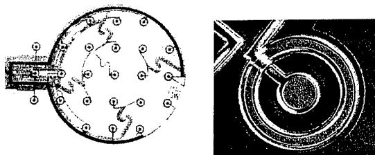
Fig. 3: Microelectrode array on ultra-thin PI substrate at 2 magnifications. The outer electrode ring (left) has a diameter of 4 mm.
