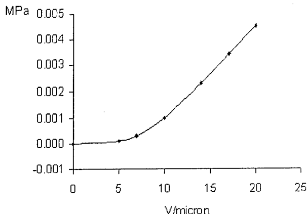
Figure 5 – Force/ m^2 versus Voltage for the actuator under test
