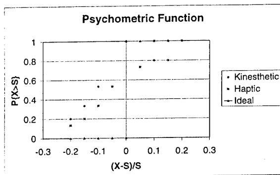
Fig. 7. Psychometric function of the CASR display. The reference stimulus S corresponds to an air pressure of 0.5 bar in the displays, i.e. in the middle of the operating range of the devices. Each data point represents the average of 30 trials (2 trials by 15 subjects).
