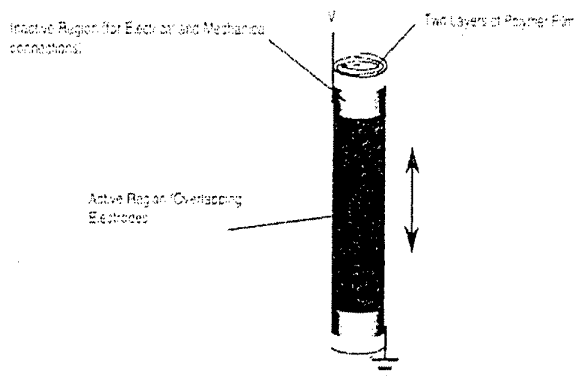
Figure 3 - Schematic of an electrostatically stricted polymer layer (ESSP) actuator
