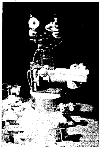
Figure 1: Babybot
