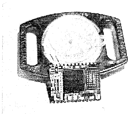
Figure 5: WESCOR Sweat sampling 'watch' with integrated flow channel containing two sensors ( \text{Na}^+ and \text{Cl}^- ). Bluecore RF communications platform shown for size comparison.
