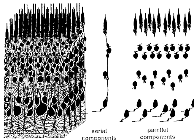
Figure 1: A scheme of the retinal modular circuitry: neurons are stacked in layers, subserving serial processing, while the arrays of like neurons within the layers support parallel processing.
