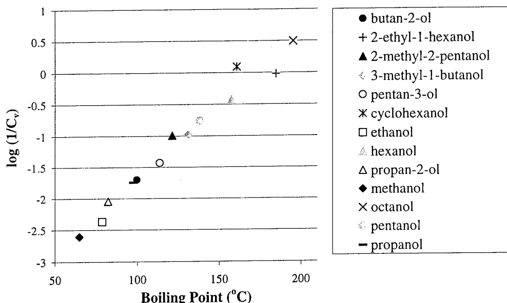
Figure 4. Log (1/C v ) vs. T b for sensor DEC/ClO 4 in response to a variety of alcohols.
