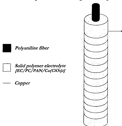
Figure 7. PANi dry polymer actuator
