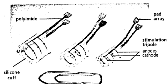
Fig. 8: Various designs of cuff microelectrodes for interfacing peripheral nerves. A method has been developed for integrating the thin film microelectrodes on polyimide with PDMS based cuffs.
