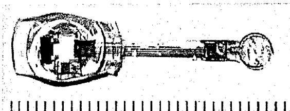
Fig. 11: A complete epiretinal implant packaged in silicone. The receiving electronics is housed in an intraocular lens made of silicone. The distance between two bars of the scale correspond to 1 mm.
