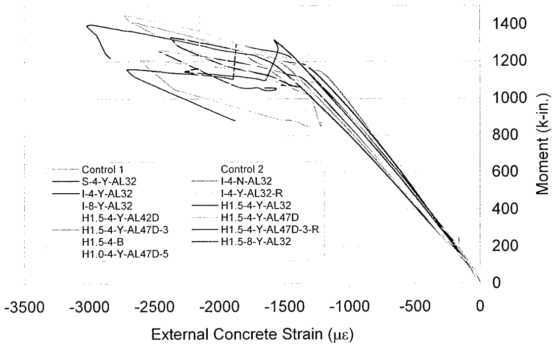
Moment - External Concrete Strain
