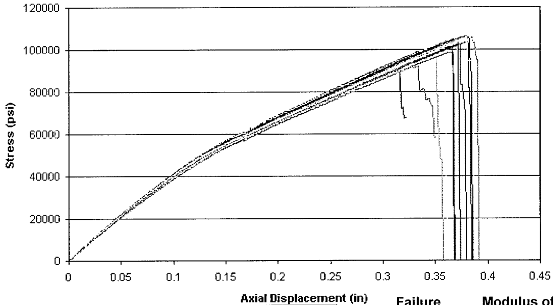
Stress vs. Displacement
