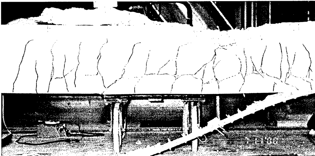
H1.5-8-Y-AL32 crack pattern in the moment span
