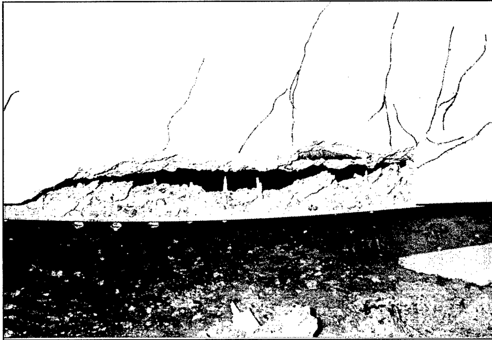
Figure 21. After testing, large chunks of concrete had fallen out of beam H1.5-4-Y-AL47D
