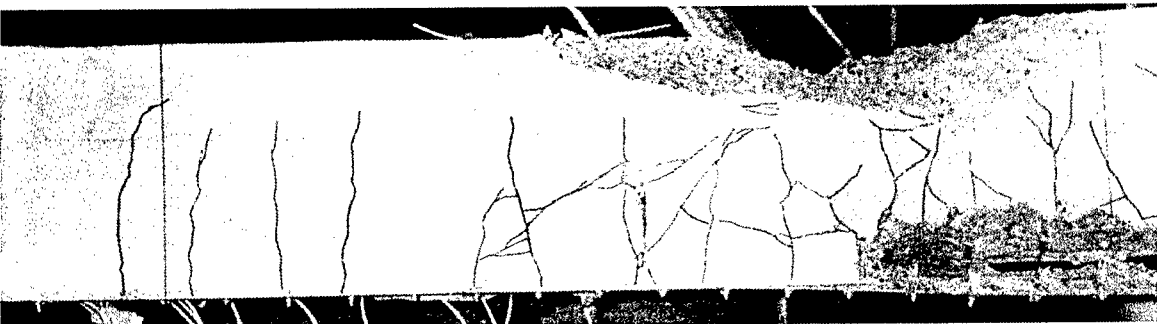
H1.5-4-Y-AL47D-3 crack pattern in the moment span
