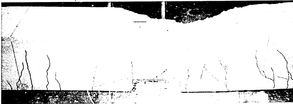
H1.5-4-Y-AL42D crack pattern in the moment span
