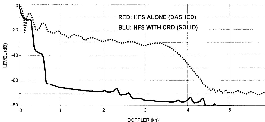
Figure 1. HFS Q-functions, T = 10 , f_c = 500 Hz, N = 8 . Graph shows amount of reverberation that can be suppressed by these waveforms as a function of target Doppler.
