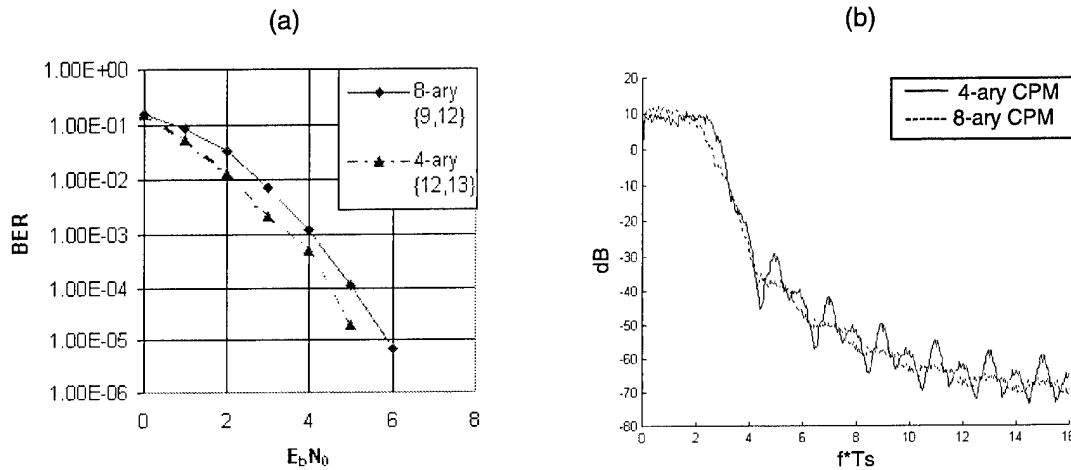
Figure 1. Comparison of 8-ary CPM using \{9/32, 12/32\} and 4-ary CPM using \{12/16, 13/16\} . 1(a) shows the BER performances and 1(b) compares the power spectra at a fixed symbol rate.
