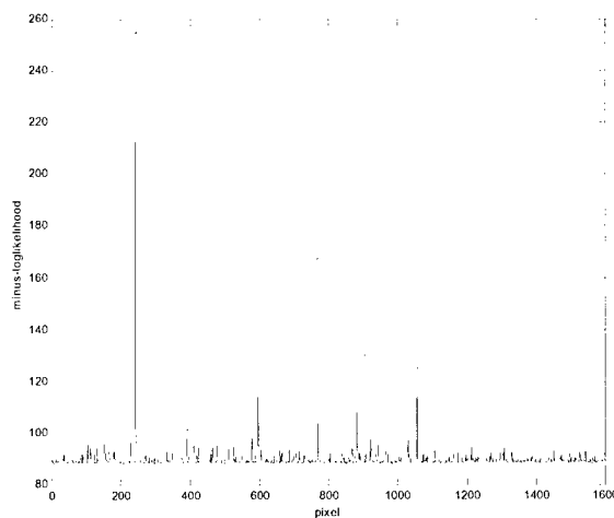
Figure 5. Magnitude of the residual of simulated hyperspectral imagery after stochastic unmixing. Asterisk indicates target pixels.
