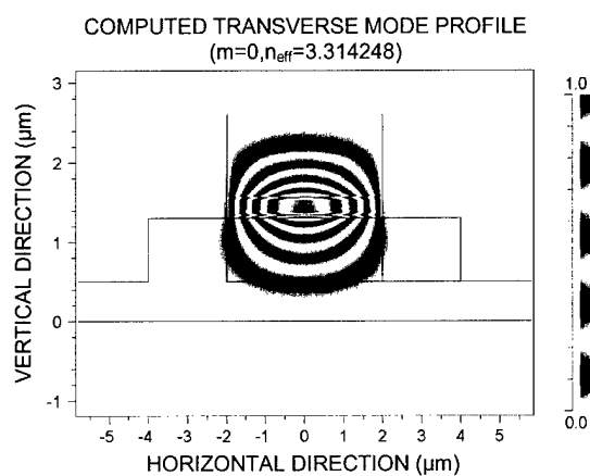
Figure 4. The LOC device structure and the corresponding mode profile.
