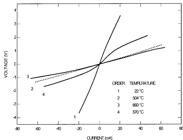
Figure 2. Current versus voltage curves measured between two silver/tungsten/titanium contacts on cubic boron nitride thin film (measured during the furnace heating/cooling cycle at the indicated temperatures and in the order given).
