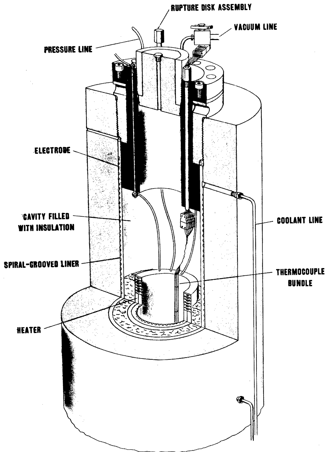
Figure 3-4. Sectional View of Cold-Wall High-Pressure Autoclave. (From: "Gas-Pressure Bonding," DMIC Report 159, September 25, 1961, p. 7, Reference 20).
