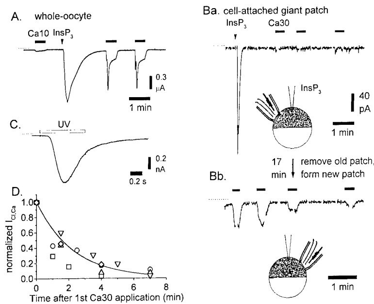
Figure 1. Blockade of Activation of Store-Operated Ca^{2+} Influx by G\Omega Sealing Procedure (A) Ca^{2+} release activated Ca^{2+} influx in oocyte recorded with two-electrode voltage clamp. Ca^{2+} influx was monitored by switching bath from Mg70 to Ca10 where indicated by heavy bars. Dotted lines in this and subsequent panels indicate zero current levels. (Ba) Ca^{2+} release failed to activate Ca^{2+} influx in preformed cell-attached giant patch. Solution inside patch pipette was alternately changed between Mg70 and Ca30 Ringer. (Bb) A new cell-attached giant-patch recording was made about 17 min after InsP_3 injection from the same oocyte. Note that the Ca^{2+} influx was recorded now in the patch formed after activation of the capacitative Ca^{2+} influx. InsP_3 (2 mM of 25 nl) was injected in both recordings from whole oocyte and patch as indicated by arrow heads in (A) and (B). Voltage ramps were repetitively applied during the patch recording to monitor the I-V curve. The corresponding transient currents have been blanked for clarity. (C) I_{Cl,Ca} was elicited by uncaging caged InsP_3 in a cell-attached giant patch. Oocyte had been loaded with 30 nl of 10 mM caged InsP_3 .
